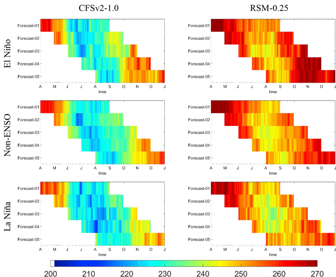
Fig. 13. Outgoing length radiation (W/m 2 ) represented in averaged domain - time of CFSv2-1.0 (left) and RSM-0.25 (right) in summer of El Niño, Neutral-ENSO and La Niña. Forecast-01 from April to September; Forecast-02 from May to October; Forecast-03 from June to November; Forecast-04 from July to December; Forecast-05 from August to January.
