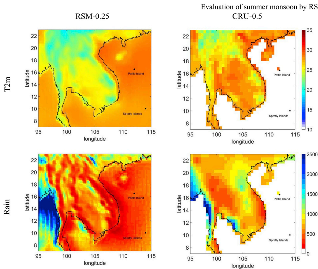
Fig. 3. Averaged surface air temperature (°C) and total rainfall (mm) of summers based on RSM-0.25 (left) and CRU with the horizontal resolution of 0.5° (CRU-0.5, right).
