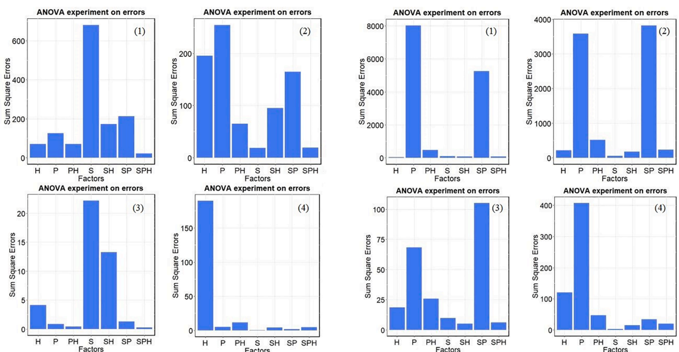
Fig. 5. ANOVA bar plot for factor combinations at (a) 0-hour and (b) 30-hour lead-times: (1) North Fork Little Beaver Creek; (2) Tygart River Valley at Daily; (3) Busseron Creek; (4) Sitlington Creek-Greenbrier River.
