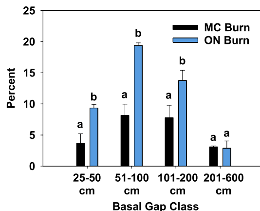
Fig. 5. Basal cover gaps (distance between plant bases) by gap class measured on site characterization plots (990 m 2 ) in burned areas at the Marking Corral (MC) and Onaqui (ON) study sites 9 yr after prescribed fire. Error bars depict standard error. Site means within a gap class followed by a different lowercase letter are significantly different ( P < 0.05 ).
