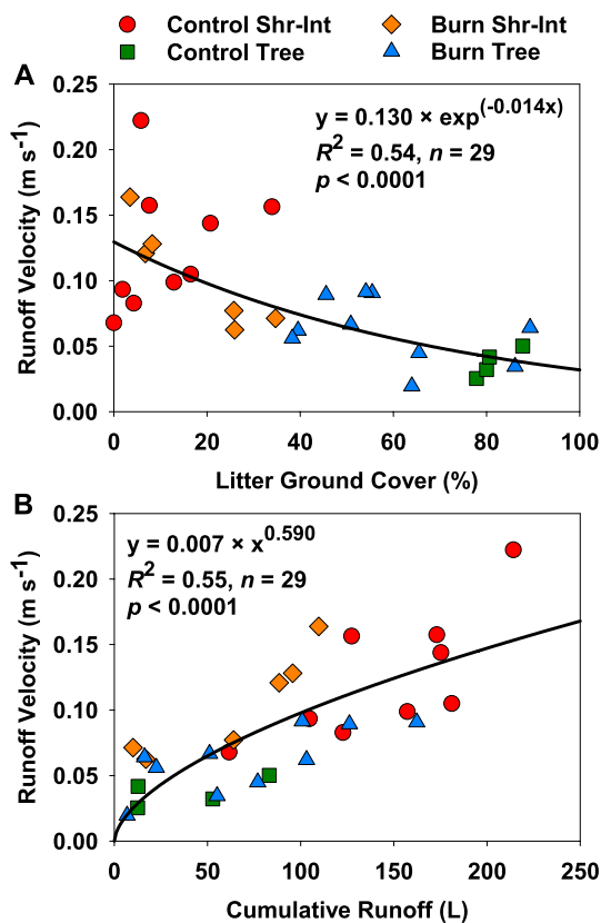
Fig. 10. Runoff velocity versus litter ground cover (A) and cumulative runoff (B) as measured on control and burned shrub-inter-space (Shr-Int) and tree (Tree) zone concentrated overland flow plots (9 m 2 ) for the 30 L min -1 flow release rate at the Marking Corral and Onaqui study sites 9 yr after prescribed fire.
