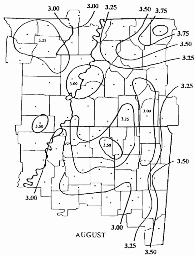
Figure 9. Distribution of 'normal' precipitation across Memphis CWA during summer.
