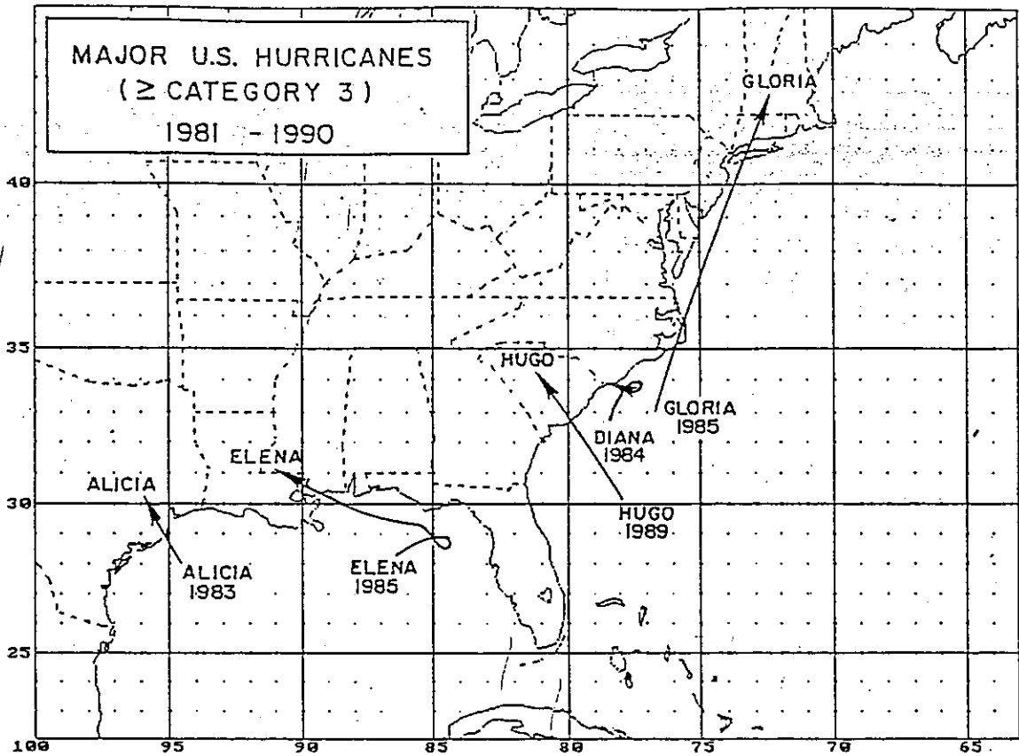
Figure 9. Major landfalling United States hurricanes (greater than or equal to a category 3) during the period 1981-1990.
