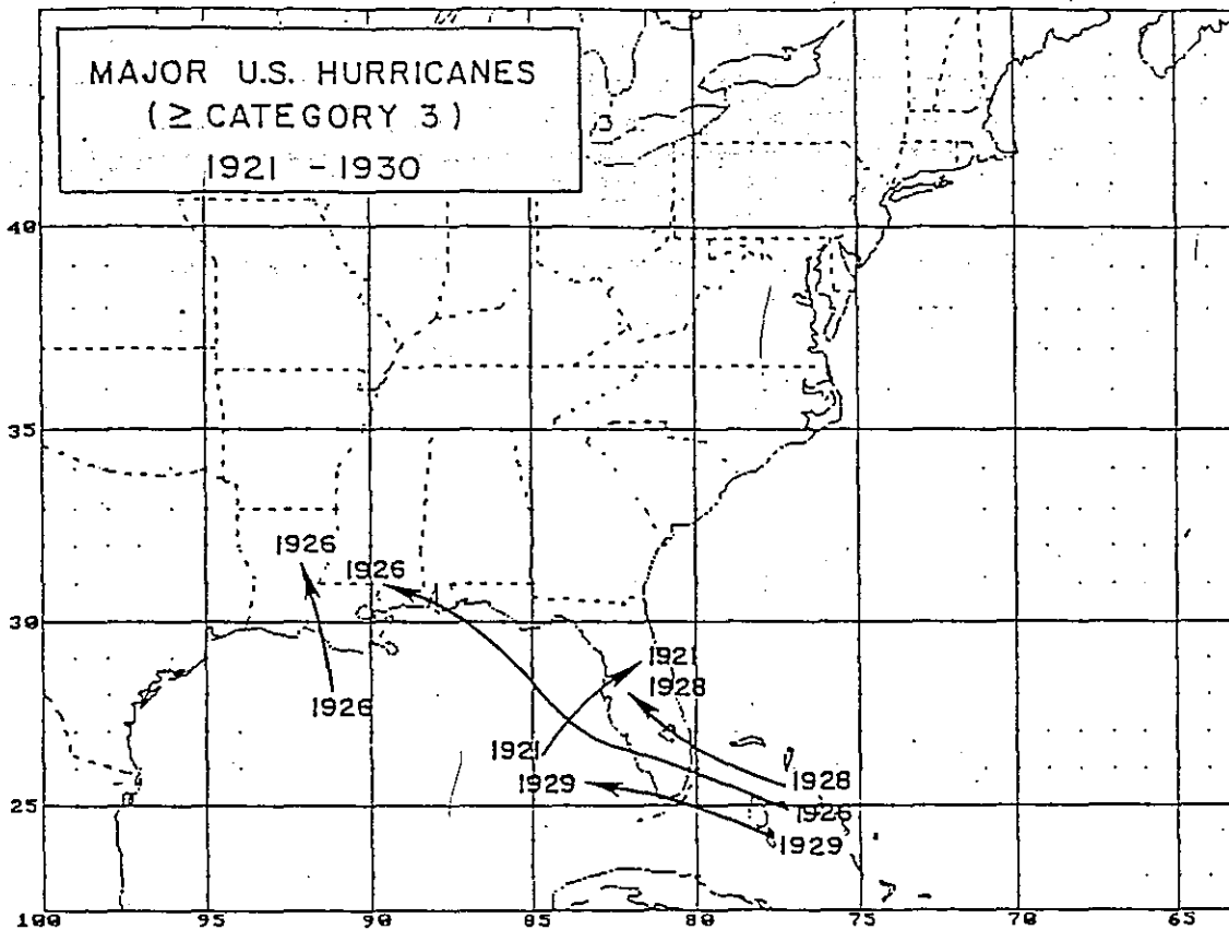
Figure 3. Major landfalling United States hurricanes (greater than or equal to a category 3) during the period 1921-1930.
