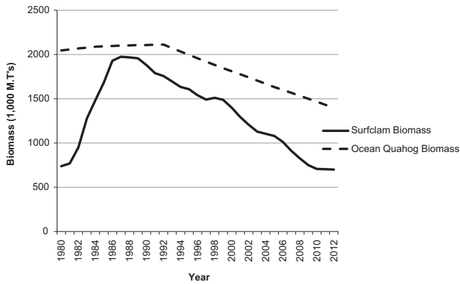
Fig. 4. Exploitable biomass (1000 Metric Tons) surfclam and ocean quahogs 1980–2012.
