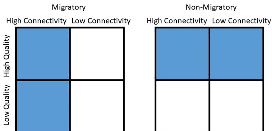
Fig. 1. Schematic of proposed vulnerability (low = shaded, high = white) to habitat quality (vertical axis) or connectivity (horizontal axis) for migratory animals (left panel) vs non-migratory animals (right panel).
