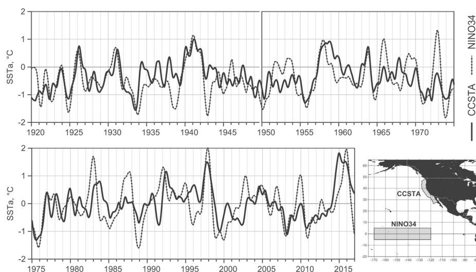
Figure 1. Monthly SST anomalies 1920–2016, 12 month low-pass smoothed, in two regions indicated in the inset: the California Current (CCSTA) and the tropical Pacific (NINO34, the NINO3.4 ENSO index region). Data are from NOAA/CDC ERSST V4; anomalies calculated from 1981 to 2010 monthly means.
