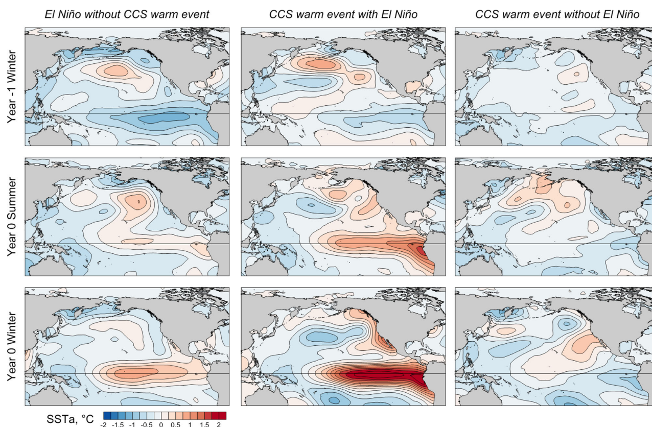
Figure 7. Sea surface temperature: spatial composites of 6-month means of monthly SSTa for El Niños and/or CCS warm events.
