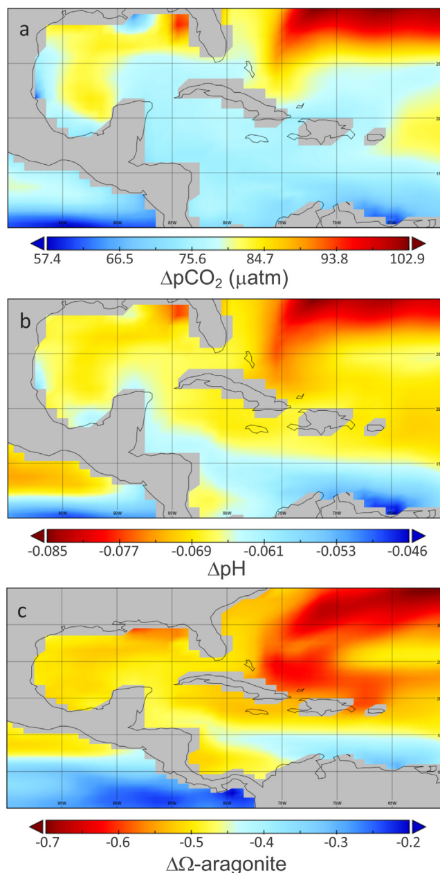
Fig. 2. Calculated changes ( \Delta ) in (a) surface seawater \text{pCO}_2 , (b) pH and (c) aragonite saturation state ( \Omega_{\text{ar}} ) in the Caribbean-wide region between 1863 and 2003 based on NOAA GFDL model output. Red colors represent areas that have experienced large changes in \text{pCO}_2 , pH and \Omega_{\text{ar}} whereas blue colors represent areas that have experienced smaller changes. (For interpretation of the references to color in this figure legend, the reader is referred to the web version of this article.)
