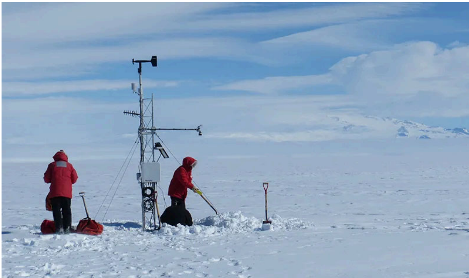
Installation and maintenance of an AWS station in the Antarctic of a type similar to D-80 AWS, which recorded the highest temperature seen on the Antarctic Plateau ( -7.0^{\circ}\text{C} on 28 December 1989). Credit: David Mikolajczyk
