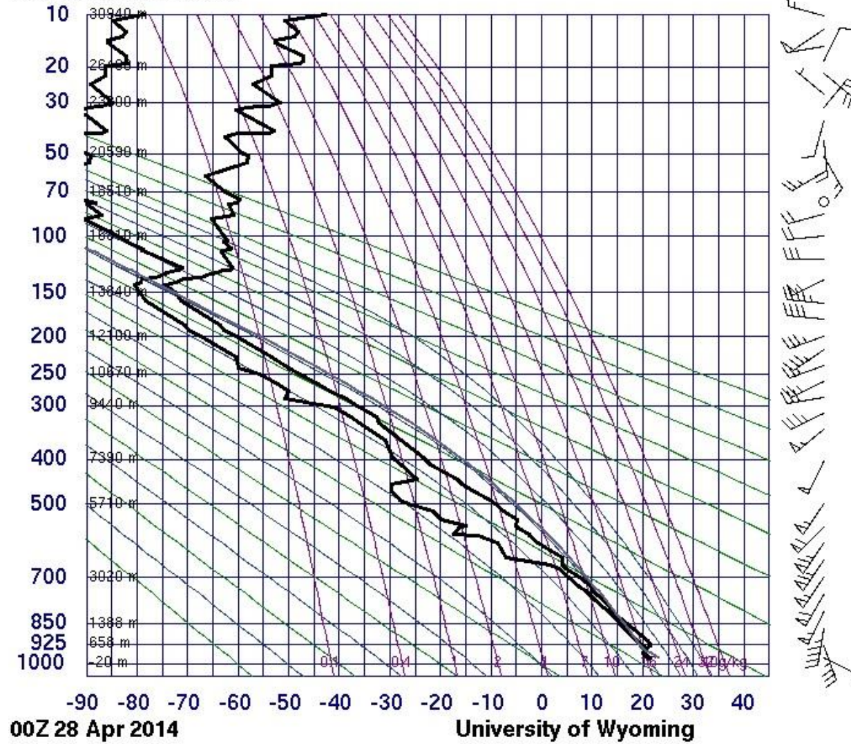
Figure 8. Stuve diagram to 10 hPa. (Plot Courtesy of the University of Wyoming)
