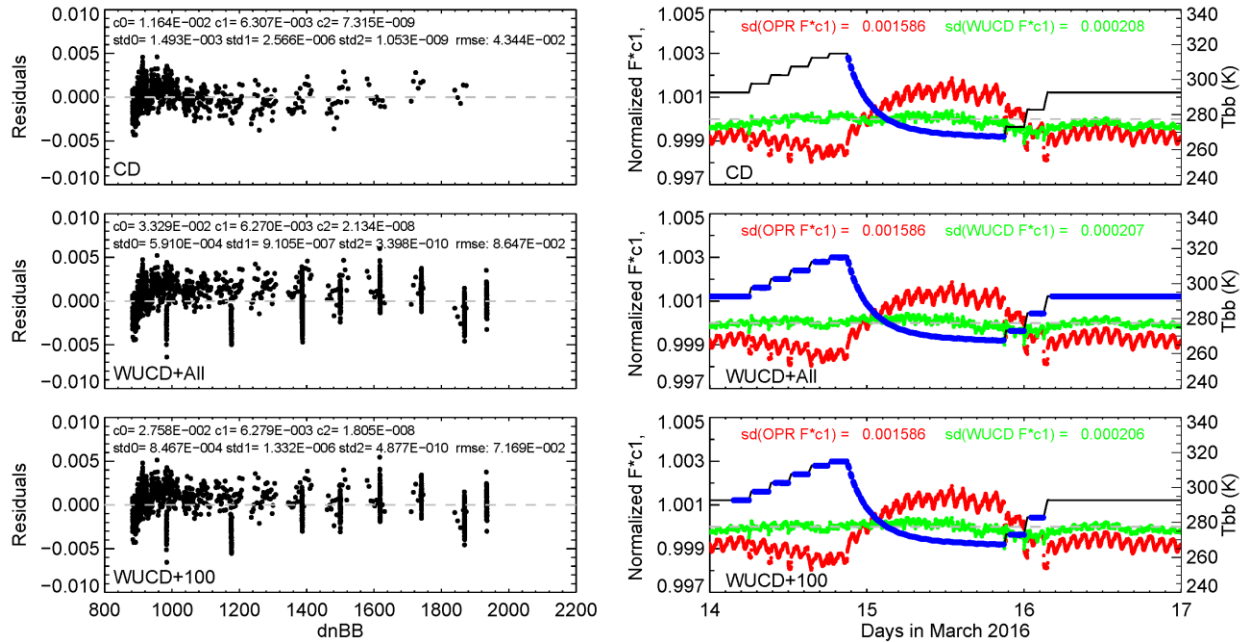
Fig. 11. (Left) Residual errors, in W/(m^2 sr \mu m) , of WUCD C-coefficients fitting results using three subsets of data (M15, detector 8, HAM-A); (right Time series of F \cdot c_1 for (red) prelaunch and (green) WUCD-derived C-coefficients. Subset of WUCD data used for fitting is marked by blue color in T_{bb} time series.
