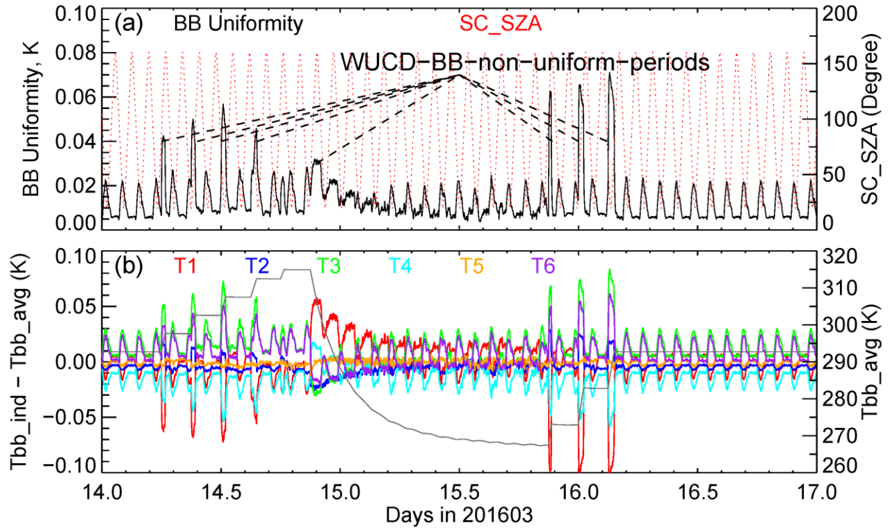
Fig. 3. Time series of (a) BB uniformity (defined as standard deviation of temperatures of six thermistors), and (b) anomalies of individual BB thermistor temperature (individual thermistor temperature readings minus average temperature of the six thermistors). Nominal operations took place before March 14, 2016 6:00 GMT and after March 16, 2016 3:00 GMT). WUCD event was conducted from March 14, 6:00 GMT to March 16 3:00 GMT, 2016.
