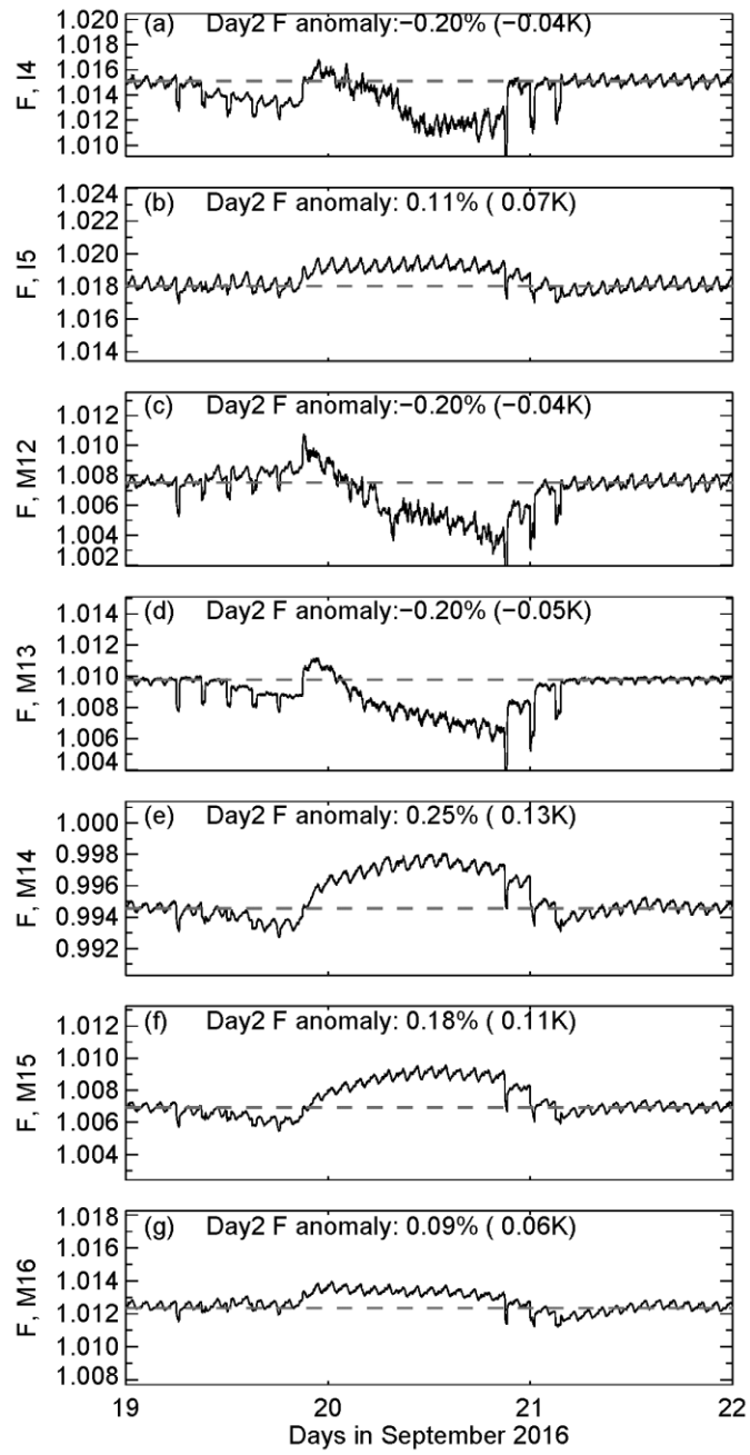
Fig. 6. Time series of band-averaged F-factors in seven VIIRS TEBs during the September 2016 WUCD.
