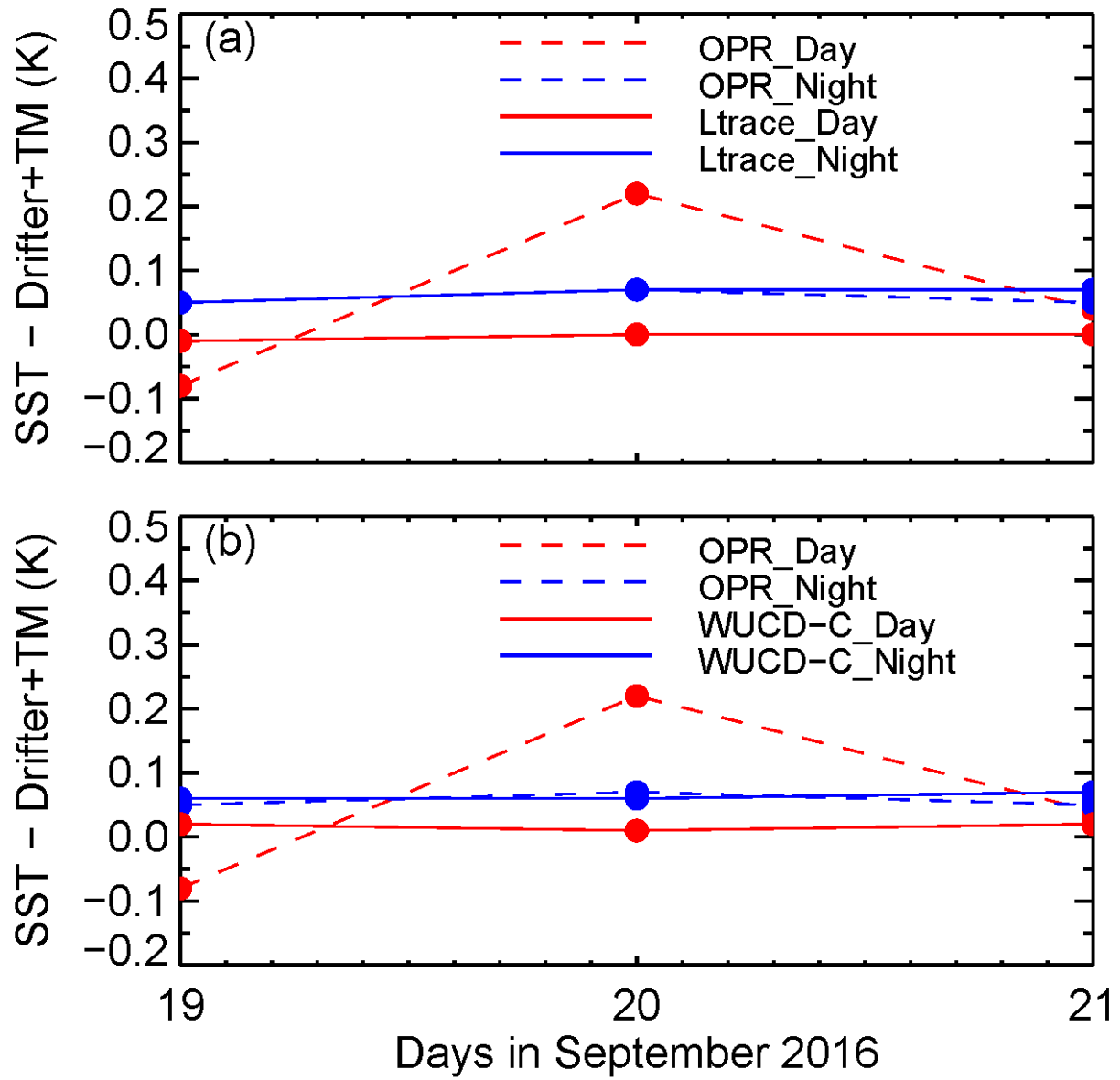
Fig. 17. Global daily-averaged SST anomaly time series during the September 2016 WUCD before and after correction: (a) the Ltrace method; (b) the WUCD-C method.
