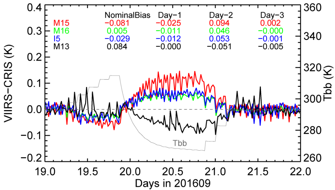
Fig. 2. VIIRS-CrIS BT difference time series during the September 19-21, 2016 WUCD event.
