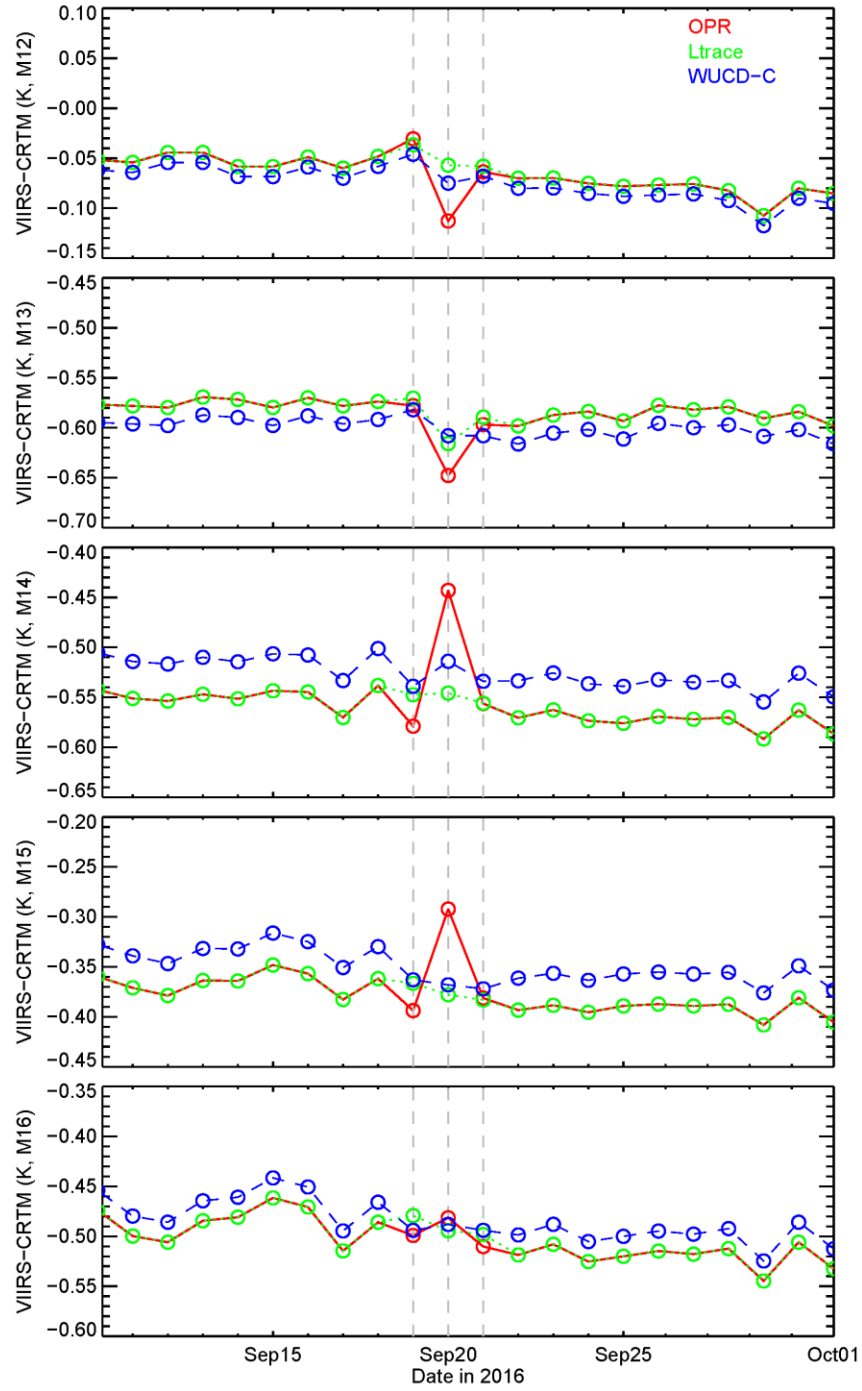
Fig. 16. Nighttime daily averaged VIIRS-CRTM BT difference time series (M12-M16, September 10, 2016 - October 1, 2016) over clear-sky ocean before (OPR, red) and after the Ltrace correction (green) and WUCD-C correction (blue).
