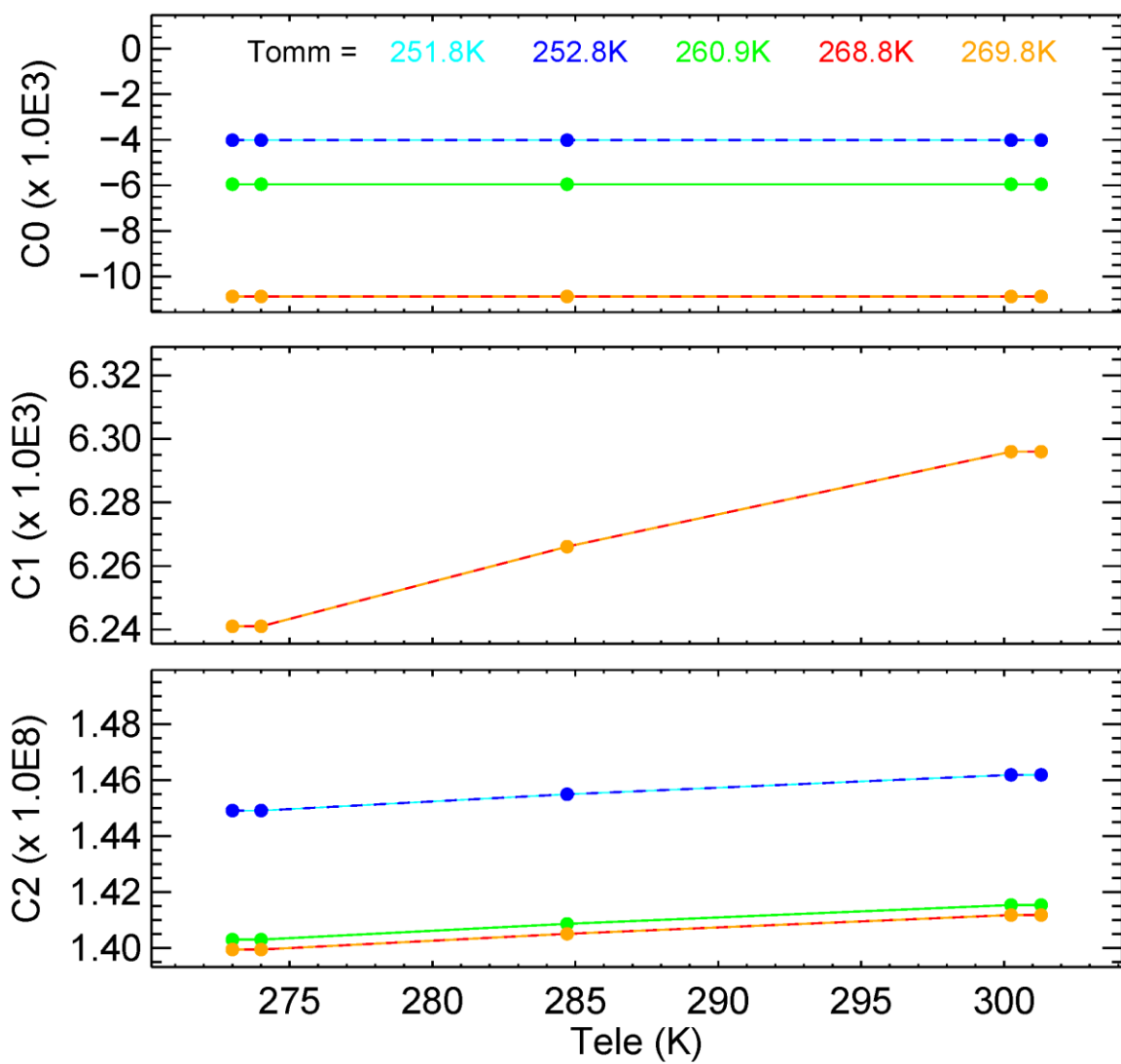
Fig. 4. Examples of prelaunch C-coefficients for M15 (electronic side-B, HAM-A, detector 1).
