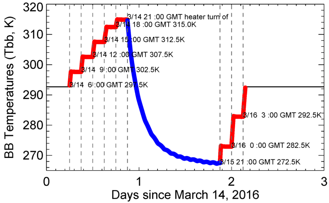
Fig. 1. Blackbody temperature sequences during the March 14-16, 2016 WUCD event. The warm-up phase is shown in red color; the cool-down phase is shown in blue color.
