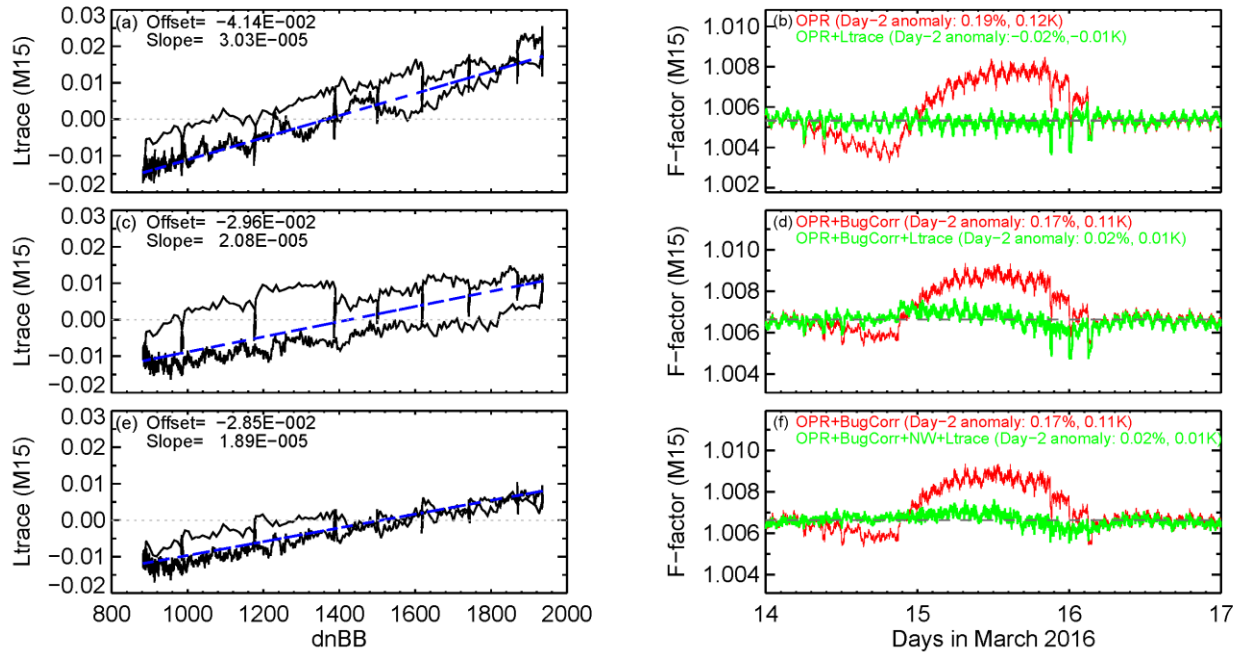
Fig. 8. (Left) Example of the Ltrace coefficients, offset and slope, for M15 (Detector 1, HAM-A) and (right) time series of band-averaged (in M15) F-factor during the March 2016 WUCD (red) before and (green) after the Ltrace correction. Top panel: before the correction of the IDPS C-coefficients implementation error and using equal BB thermistor weights. Middle panel: same as in the top panel, but after the correction of the C-coefficients implementation error (BugCorr). Bottom panel: same as in the middle panel, but after additionally applying non-equal BB thermistor weights (NW). The black lines in the left panel show Ltrace term (see Eq. 7) as a function of dn_{bb} ; the fitted line defined by the Ltrace coefficients are shown in blue dash lines.
