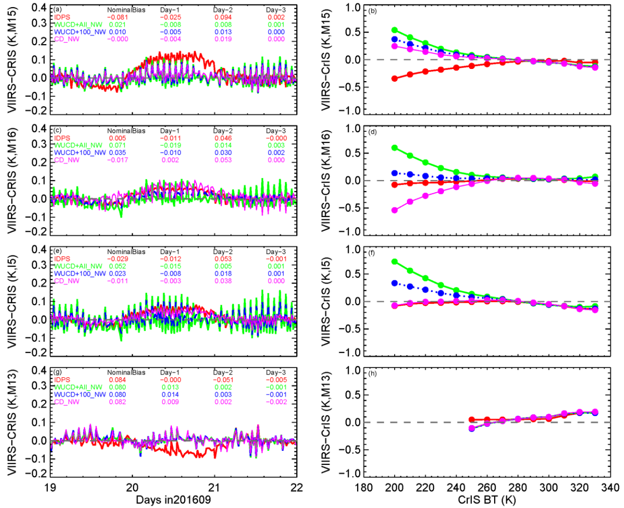
Fig. 15. (Left) time series of VIIRS-CrIS BT difference and (right) scene temperature dependent biases in bands M15-M16, I5, and M13 during the September 2016 WUCD for the NOAA operational processing (OPR, red) and after the WUCD-C corrections reprocessed with: (1) WUCD+All C-coefficients (WUCD+All_NW, green), (2) WUCD+100 C-coefficients (WUCD+100, NW, blue), and (3) CD-only C-coefficients (CD_NW, magenta). Non-equal BB thermistor weights were applied during the reprocessing.
