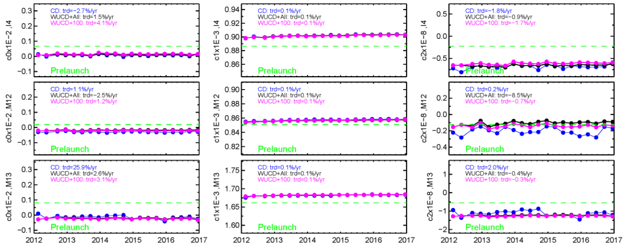
Fig. 13. Band-averaged C-coefficients for the MWIR bands from February 2012 to December 2016 (I4, M12-M13). Prelaunch C-coefficients are shown in green color for comparison purpose.
