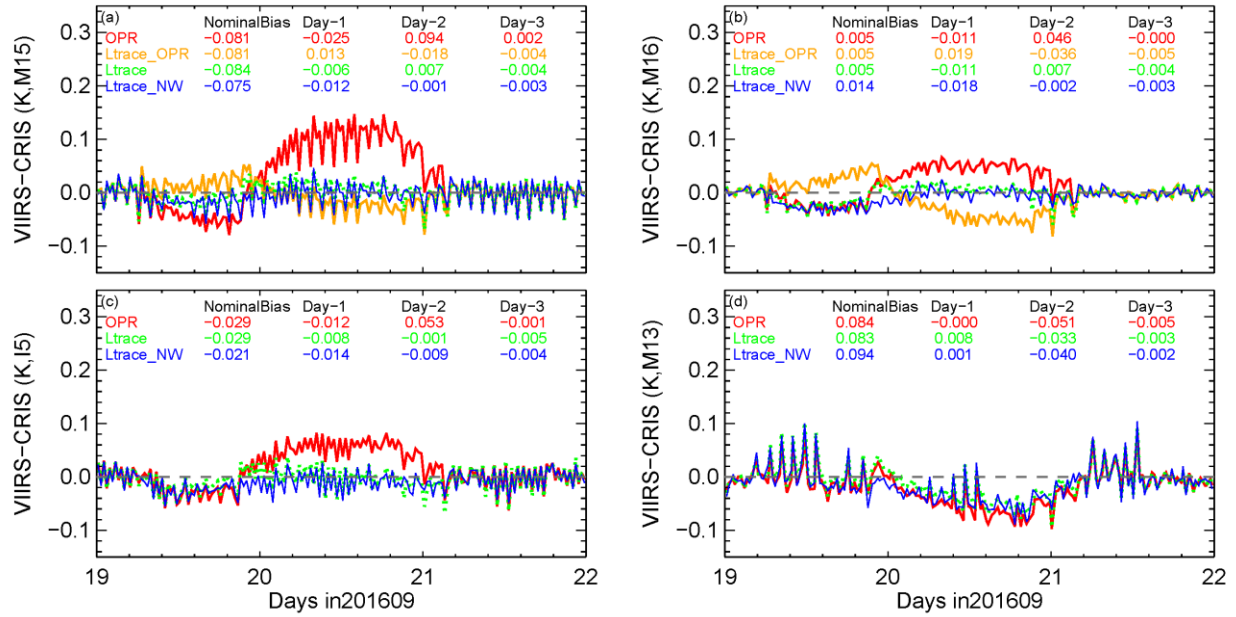
Fig. 14. Time series of VIIRS-CrIS BT difference in M15-M16, I5, and M13 during the September 2016 WUCD event: (1) NOAA operational processing (OPR, red), (2) same as (1) but after the Ltrace correction (Ltrace_OPR, orange, in M15 and M16 only), (3) same as (2), but after the correction of the IDPS C-coefficients implementation error (Ltrace, green), and (4) same as (3), but with non-equal BB thermistor weights (Ltrace_NW, blue).
