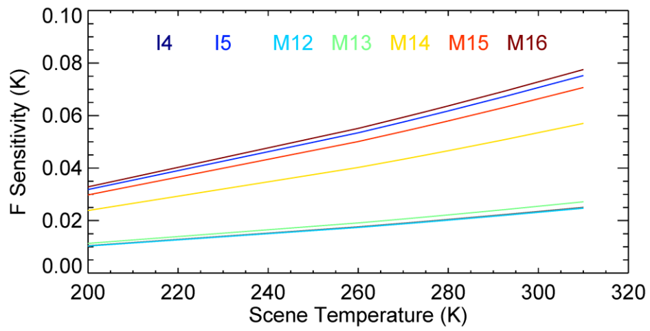
Fig. 7. Sensitivity of scene temperatures to a hypothetical 0.1% anomaly in F-factor (theoretically calculated based on Planck's function. Curves for I4 and M12 overlap each other).
