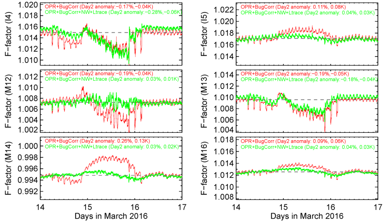
Fig. 9. Time series of band-averaged F-factor (red) before and (green) after the Ltrace correction for I4-I5, M12-M14, and M16 for the March 2016 WUCD. The IDPS C-coefficients implementation error (BugCorr) is corrected and non-equal BB thermistor weights (NW) are applied in all bands.
