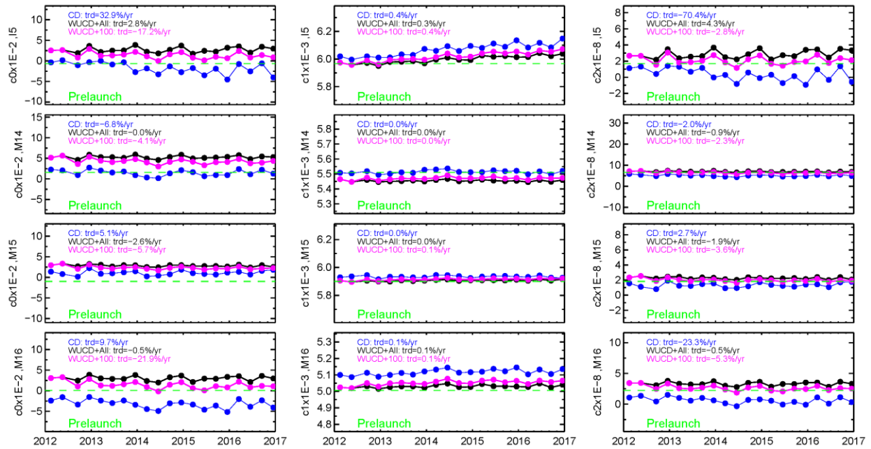
Fig. 12. Band-averaged C-coefficients derived from the three subsets of WUCD data for LWIR bands from February 2012 to December 2016 (I5, M14, M15 and M16). Prelaunch C-coefficients are shown in green color for comparison.
