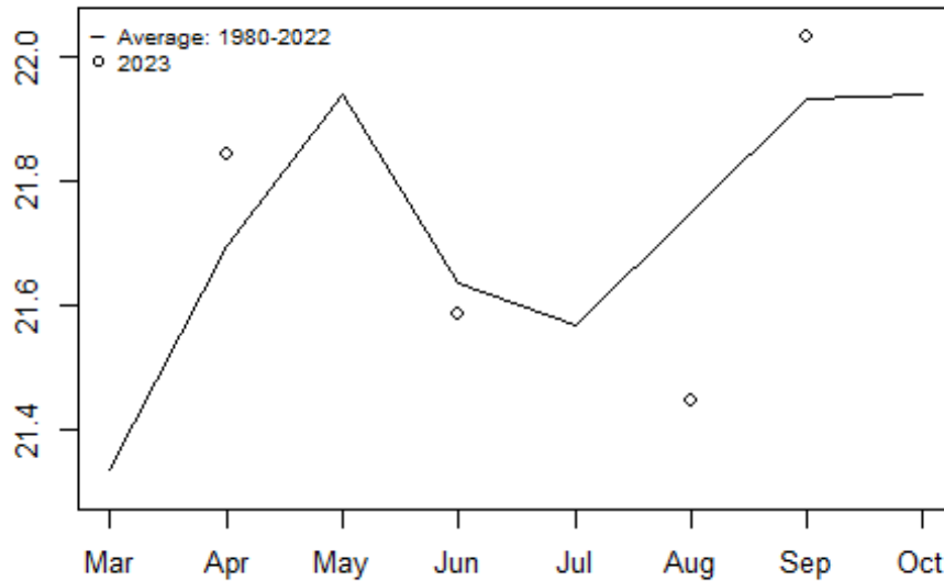
Figure 6. -- Average monthly gauge height against month in Auke Creek for 2023 and the 1980-2022 average.
