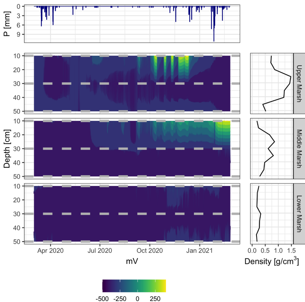
Figure 2 Redox potential (Eh) contour graphs across the experimental transect. The grey, dashed lines at 10, 30 and 50 cm indicate the Eh probe's depth, the values in between are linearly interpolated. Soil bulk density at each marsh position is shown to the right of each contour plot. Precipitation time series for the studied period is shown above the Eh profile to illustrate the timing of storm events.
