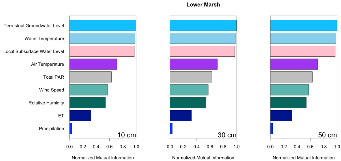
Figure 4 Mutual information between Eh time series and other hydroclimatic parameters used to explore Eh 's temporal variability. All the relationships between Eh and the parameters shown in the figure are statistically significant ( p -value < 0.0001 ). The mutual information values are normalized by the Entropy of each individual signal.
