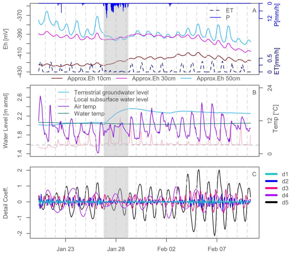
Figure 5 Multilevel decomposition of Eh for the 10 cm, 30 cm, and 50 cm depths in the lower marsh position between January 20th and February 10th, 2021 (marked in Figure 3 by a shaded rectangle). A) shows the Eh approximate coefficients at 16 h, hourly precipitation (P), and hourly evapotranspiration (ET). B) shows local subsurface water level, air temperature, water temperature, and regional terrestrial groundwater level. C) shows the detailed components of Eh at dyadic scales of 2 (d1), 4 (d2), 8 (d3), 16 (d4), and 32 (d5). The shaded region marks a precipitation event that occurred in the area in late January. The dashed gray line in B) marks the elevation (amsl) of the salt marsh. The vertical dashed gray lines mark the beginning of every new day (midnight).
