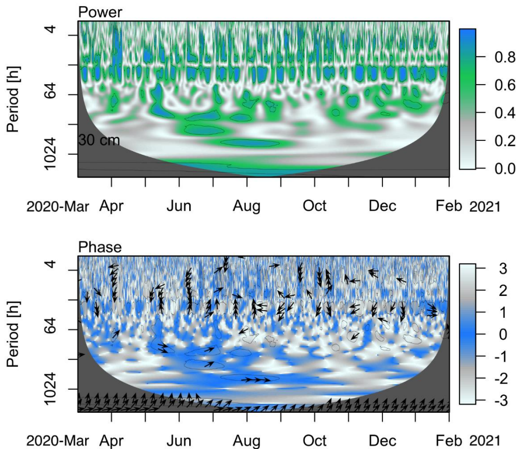
Figure 6 Cross wavelet analysis of subsurface water level and Eh signals at the 30 cm depth in the lower marsh position. The figure shows the modulus (power) and phase (angle in radians) of the wavelet cross-spectrum in the top and bottom panels, respectively. The power plot indicates higher coherences with blue and green colors while low coherence is illustrated by gray colors. In the phase shift, the 0-radian value indicates that the two time series are in phase while +3 radians and -3 radians indicate anti-phase (Note that the color scale actually goes from -\pi to +\pi ). Arrows pointing towards the right indicate that the time series are in phase, arrows pointing to the left indicate that the two time series are anti-phase, arrows pointing downward explain that the subsurface water level is leading, and arrows pointing upward indicate that the subsurface water level is lagging.
