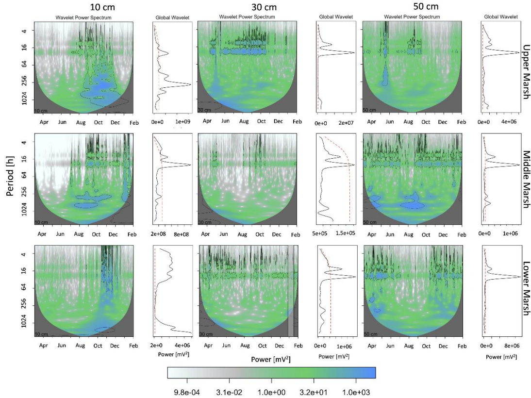
Figure 3 Continuous wavelet spectrum and global wavelet spectrum of Eh time series between March 2020 and February 2021. In the wavelet spectrum, the shaded regions signify the cone of influence. The color bar signifies the strength of power in the wavelet spectrum. Areas surrounded by the black polygons display significant powers (within 95% significance level). In the global wavelet spectrum, the red-dashed line is the 95% significance level using a red-noise background spectrum. The shaded area in the 30 cm depth of the lower marsh (bottom center panel) marks the time of a precipitation event studied in detail in Figure 5.
