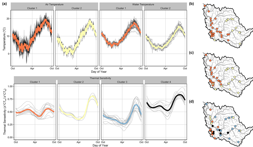
Figure 4. Average time series (a) and spatial clustering results (columns and colors indicate unique clusters) for average annual air temperature (b), water temperature (c), and thermal sensitivity (d) in the Snoqualmie basin. The colored lines indicate mean average annual values for each cluster, and gray lines denote average annual values for each site within a given cluster.
