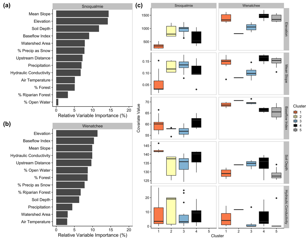
Figure 6. Relative variable importance for all covariates in the Snoqualmie (a) and Wenatchee (b) basins, together with the distributions of variables across clusters for the four most important variables (c) in the Snoqualmie basin (mean slope, elevation, soil depth, and baseflow index) and in the Wenatchee basin (elevation, baseflow index, mean slope, and hydraulic conductivity). Boxes are grouped and colored by cluster membership. See Fig. S8 for plots of the remaining relative variable importance.
