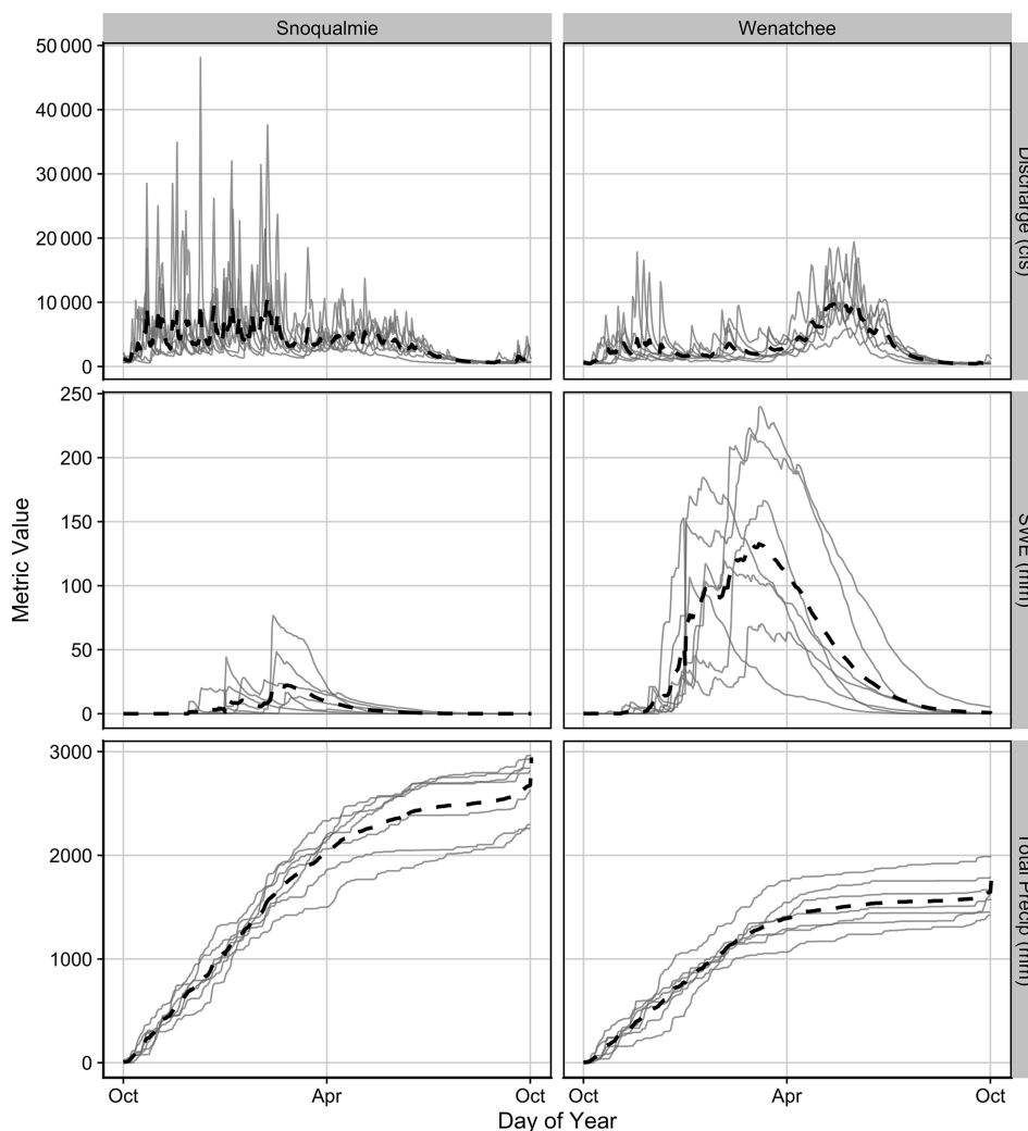
Figure 2. Average annual discharge, snow water equivalent (SWE), and total precipitation for the outlets of the Snoqualmie and Wenatchee basins across the sampling time frame (black dashed lines) and interannual variability across the 7 water years included in this analysis (2015–2021, gray lines). Discharge gage locations can be found in Fig. 1a and b, and SWE and precipitation data are from DAYMET Daily Surface Weather data for the upstream watershed of each discharge gage (Thornton et al., 2020).
