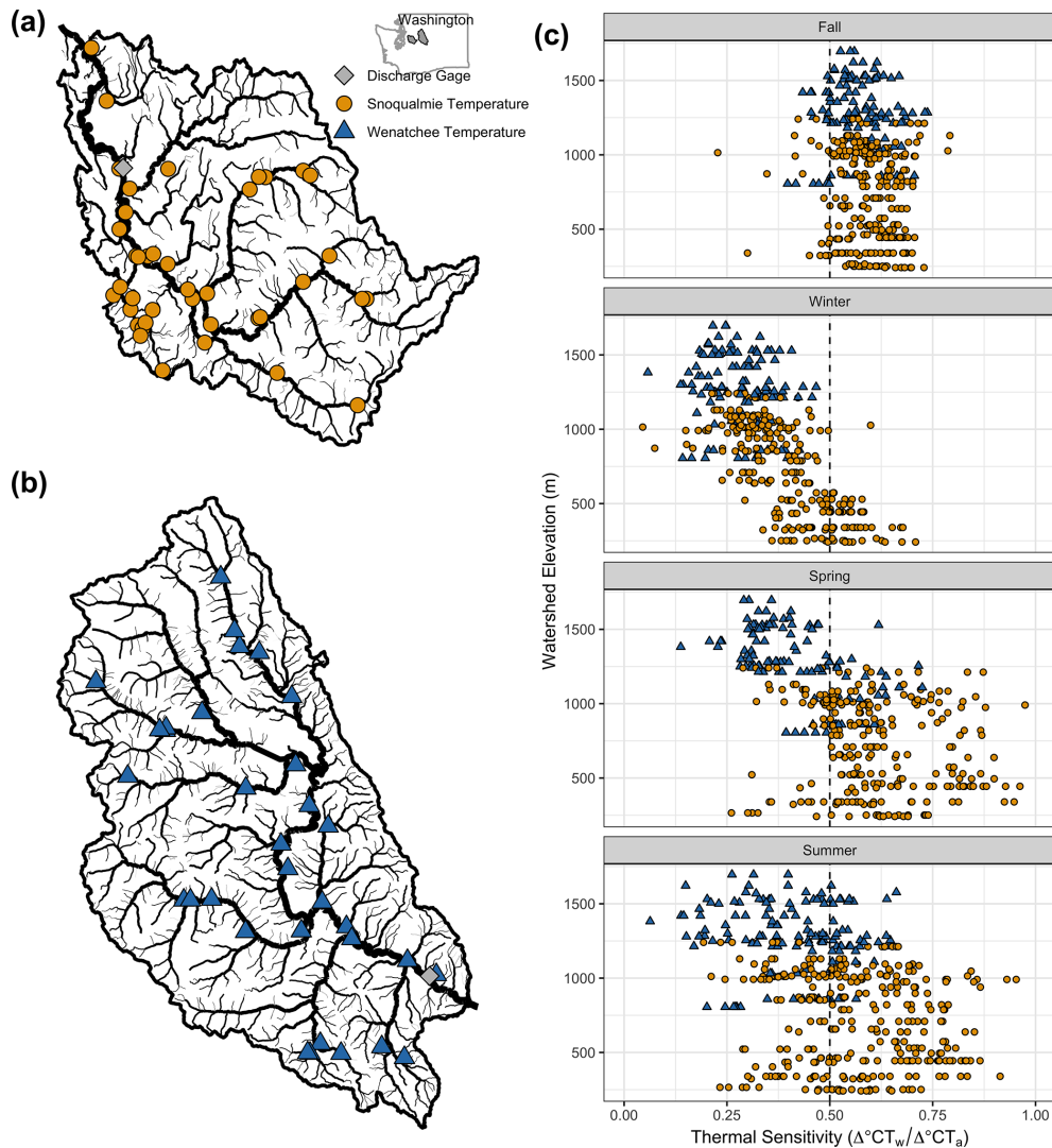
Figure 1. A map of the Snoqualmie (a) and Wenatchee (b) basins' water and air temperature monitoring sites as well as the most downstream USGS gage for each basin. Thermal sensitivity, defined as the change in water temperature with a single degree change in air temperature, versus mean watershed elevation (MWE) for each site–year combination (c). The dashed line in panel (c) is included as a reference.
