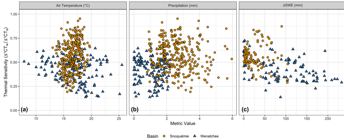
Figure 3. Summer thermal sensitivity values for all site–year combinations in the Snoqualmie and Wenatchee basins versus air temperature (a) and precipitation (b). Spring thermal sensitivity values for all site–year combinations versus the total snow water equivalent (SWE) (c) from gridded DAYMET data for each sampling point. Points are colored by basin. Basins that have no snowmelt in a given year are not shown in panel (c).
