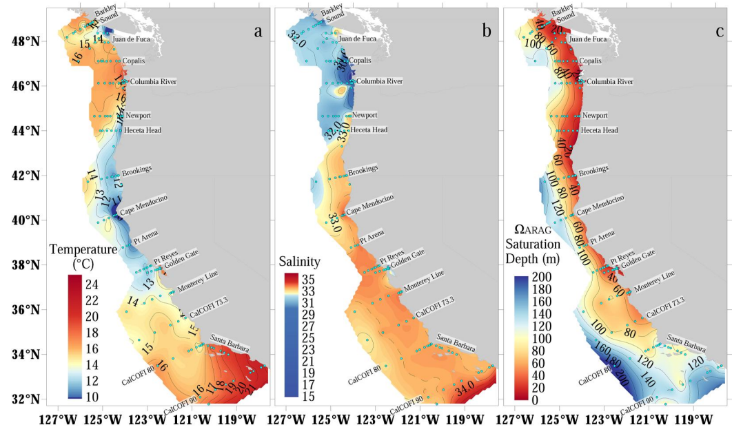
Figure 2. Surface distribution of: (a) temperature; (b) salinity; and (c) aragonite saturation depth along the coastal margin of the CCE during the WCOA2021 cruise in June–July.
