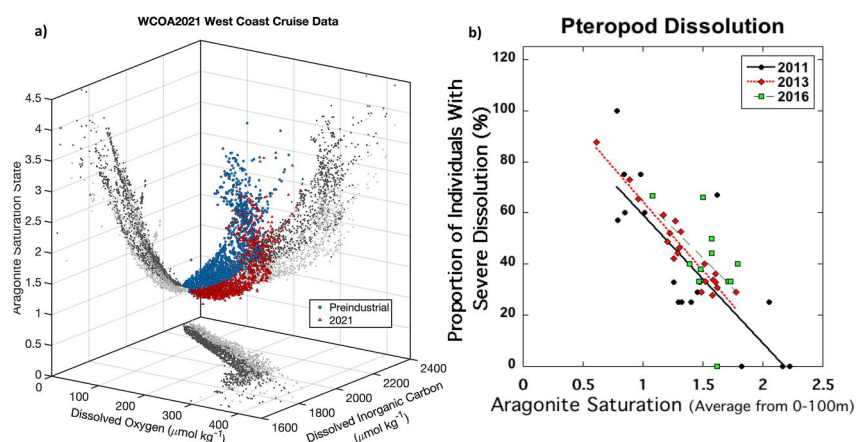
Figure 7. (a) 3-D plot of the relationship between aragonite saturation state versus dissolved oxygen and dissolved inorganic carbon for preindustrial (blue and dark gray dots) and the 2021 observations (red and light gray triangles); and (b) relationship between the proportion of L. helicina pteropods that exhibit Type II or Type III dissolution versus aragonite saturation state averaged over the upper 100 m of the water column from the 2011, 2013, and 2016 cruises with linear fit of y = -49.43x + 112.22 ; R^2 = 0.65 . The threshold for severe dissolution has been determined to be at an aragonite saturation state value \sim 1.2 based on the expert consensus studies (after Bednaršek et al., 2019). The pteropods that show severe dissolution from the cruise results are primarily from the samples located shoreward of the shelfbreak.
