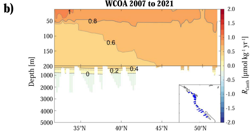
Figure 3. Distribution of: (a) anthropogenic CO 2 (in \mu\text{mol kg}^{-1} ) at the surface; and (b) anthropogenic CO 2 rate of change in \mu\text{mol kg}^{-1} \text{yr}^{-1} along the coast from south to north. Vertical white lines below \sim 400 m indicate locations where the accumulation rates in the region are not significantly different from 0.
