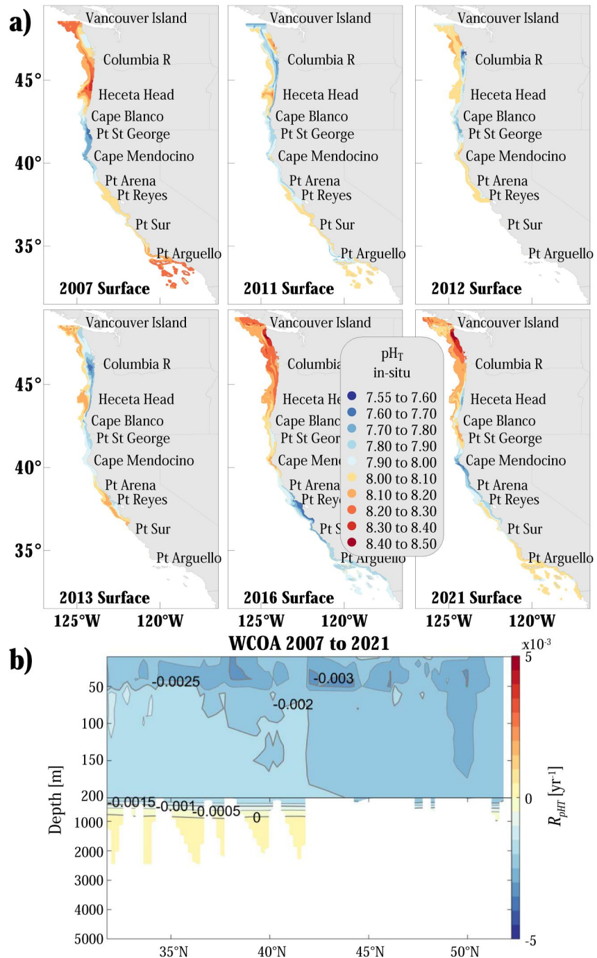
Figure 6. Distribution of: (a) pH_T at the surface; and (b) south to north vertical distribution of pH_T rate of change in the California Current Ecosystem.
