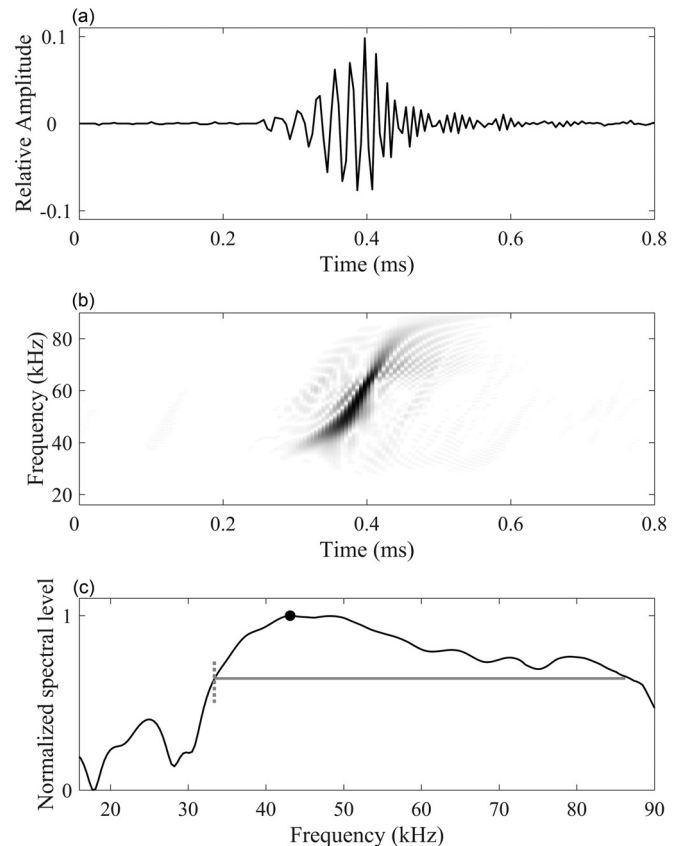
FIG. 3. Exemplar click recorded during the 2017 encounter with True's beaked whales shown as the waveform (a), Wigner-Ville plot (b), and normalized power spectrum (c). The peak frequency in the power spectrum is denoted by the circle, the -10 dB lower frequency bound is denoted by a dashed line, and the -10 dB bandwidth is shown as a solid grey line.
