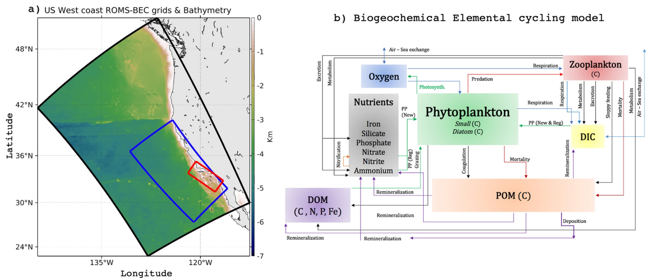
Figure 1. (a) Regional Oceanic Modeling System-Biogeochemical Elemental Cycling (ROMS-BEC) model configurations. \Delta x = 4 km is the black box, \Delta x = 1 km is the blue box, and \Delta x = 0.3 km is the red box. Background color shading show the topography from \Delta x = 4 km. (b) Schematic of the Biogeochemical Elemental Cycling model. The schematic shows state variables (boxes) and biogeochemical rates and feedback (arrows).
