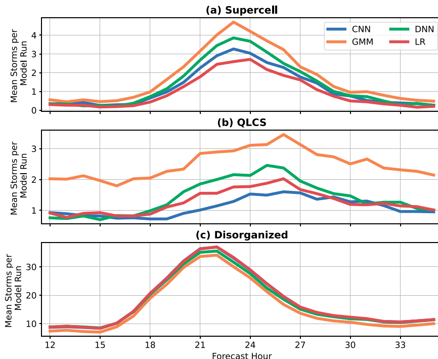
FIG. 14. The average number of 2016 NCAR-WRF storms per model run classified as (a) supercells, (b) QLCSs, and (c) disorganized for each forecast hour for the CNN (blue), GMM (orange), DNN (green), and LR (red) classifiers.
