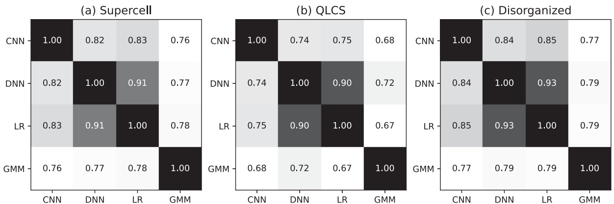
FIG. 8. Correlation matrices for the (a) supercell, (b) QLCS, and (c) disorganized predictions from the four classifiers for all ~40 000 storms in the 2016 NCAR-WRF dataset. Darker shading indicates higher correlation.
