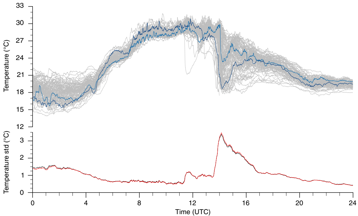
Fig. 3. Time series of (top) temperature and (bottom) its standard deviation across the network measured at the APOLLONs and WXT stations on 29 Jun 2021. Cold pool passage can be recognized by the strong drop in temperature around 1330 UTC [or 1530 Central European summer time (CEST)]. Blue-colored lines highlight the propagation of the cold pool between two stations distanced by 7.2 km. The red line shows the variability computed by removing stations closer than 1 km to each other.
