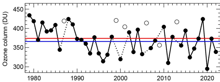
Fig. 5.32. Minimum of the daily average total ozone column (Dobson units, DU) for Mar poleward of 63°N equivalent latitude (Butchart and Remsberg 1986). Open circles represent years in which the polar vortex was not well-defined in Mar, resulting in relatively high values owing to mixing with lower-latitude air masses and a lack of significant chemical ozone depletion. Red and blue lines indicate the average total ozone column for 1979–2021 and 2005–21, respectively. Ozone data for 1979–2019 are based on the combined NIWA-BS total column ozone database version 3.5.1 (Bodeker and Kremser 2021). Ozone data for 2020–22 are from OMI. Adapted from Müller et al. (2008) and WMO (2022), and updated using ERA5 reanalysis data (Hersbach et al. 2020) to determine equivalent latitude.
