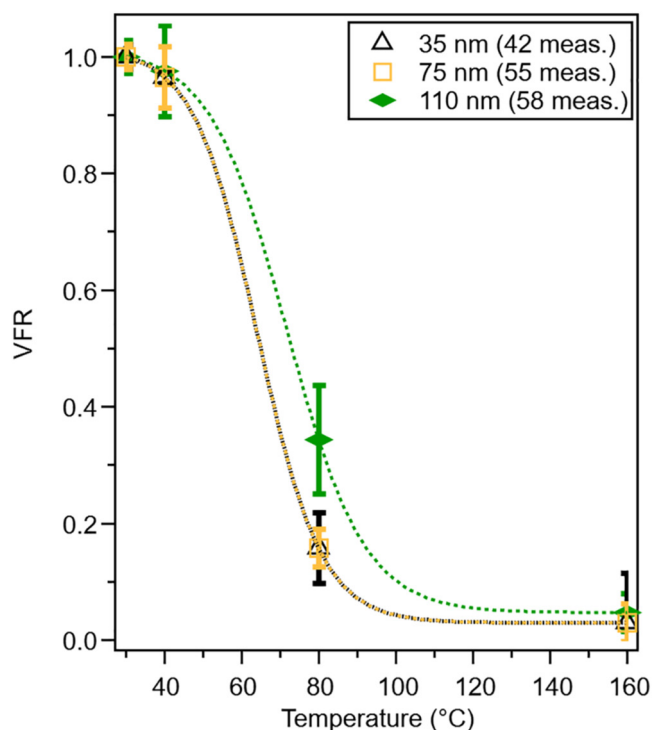
Figure 3. Average volume fraction remaining at 40, 80, and 160 °C for 35, 75 and 110 nm size-selected particles during the background period (March 27–31) with sigmoidal fits to data. The error bars represent standard deviation and the number of measurements at each size is shown in the legend. Initial volume ( VFR = 1 ) is assumed to be the volume at 30 °C.
