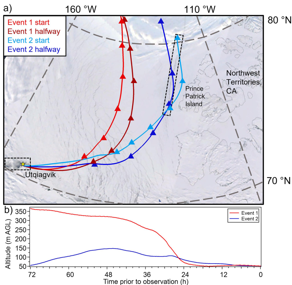
Figure 5. Air mass back trajectory analysis for each growth event. (a) Hybrid Single-Particle Lagrangian Integrated Trajectory (HYSPPLIT) 72-hr back trajectories for each event plotted with corrected-reflectance MODIS satellite images from March 11, with one trajectory at the beginning of each event and one halfway through growth. Triangles mark 12-hr time points. The blue region in the upper-left corner is an imaging artifact and does not represent open ocean. Black boxes highlight regions with sea ice leads. (b) Average altitudes above ground level (AGL) of the two trajectories calculated for each event.
