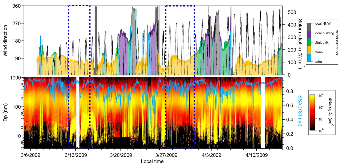
Figure 1. Meteorological data and bulk particle properties during the entire Ocean-Atmosphere-Sea Ice-Snowpack (OASIS) observation period. Plotted above are wind direction (color-coded to show relative direction of origin) and downwelling solar radiation. The lower plot is the particle number-size distribution (diameters 4–1,000 nm) and single scattering albedo measured at 781 nm (light blue). The focus of this work is a background period (March 27–31) and two distinct ultrafine particle growth events (March 12–14), which are boxed in blue.
