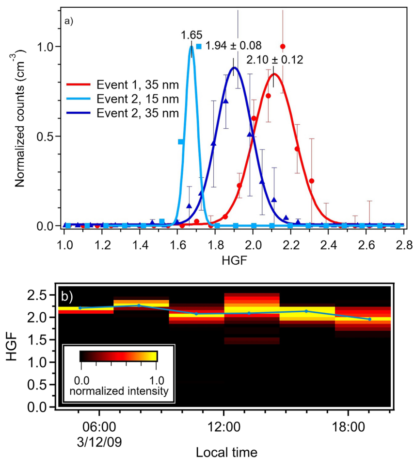
Figure 6. (a) Measured hygroscopic growth factors ( HGFs ) at 90% RH for 15 and 35 nm size-selected particles during each event (15 nm data missing for Event 1). Markers are the averaged size distributions measured during each event. The error bars represent standard deviation and the number of measurements at each size is shown in the legend. Solid lines are Gaussian fits of the data. Distributions were normalized prior to plotting to facilitate comparison. (b) Time evolution of Event 1 HGF . The Event 2 HGF distribution did not change during the growth period.
