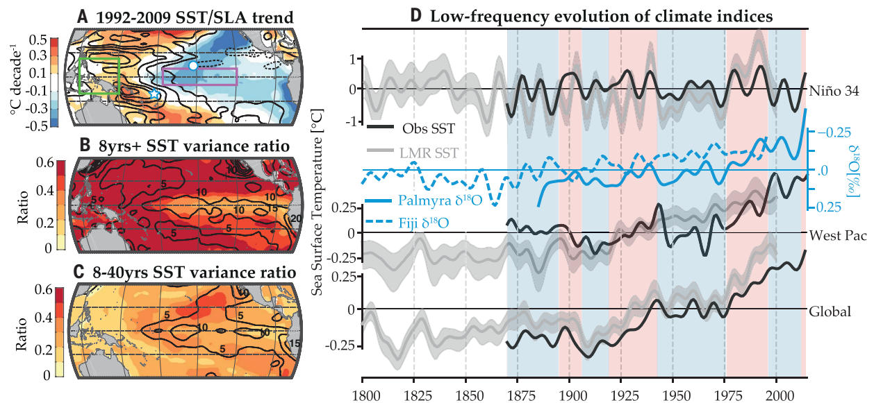
Fig. 1. Observed decadal variability in the tropical Pacific. (A) 1992–2009 linear trend of annual SST (shading, 0.1^{\circ}\text{C decade}^{-1} ) and sea surface height (black contours, 2\text{ cm decade}^{-1} , where dashed contours indicate negative trends, solid contours indicate positive trends, and the zero contour is omitted). (B and C) Eight-year low-pass (B) and 8- to 40-year band-pass (C) filtered SST variance (black contours, in 10^2\text{ }^{\circ}\text{C}^2 ) and ratio of the filtered SST variance to total SST variance (shading). (D) Eight-year low-pass filtered time series of SST averaged over the Niño34 region ( 5^{\circ}\text{N} to 5^{\circ}\text{S} ; 170^{\circ}\text{W} to 120^{\circ}\text{W} ), over the western tropical Pacific ( 10^{\circ}\text{N} to 10^{\circ}\text{S} ; 120^{\circ}\text{E} to
