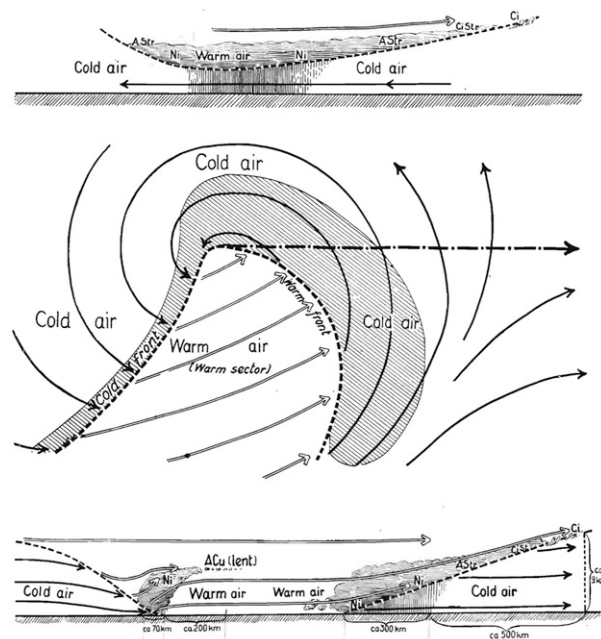
FIG. 16-4. Idealized cyclone presented by the Bergen school (Bjerknes and Solberg 1921, their Fig. 18; Bjerknes and Solberg 1922, their Fig. 1). The figure is provided through the courtesy of the Norwegian Geophysical Society.
