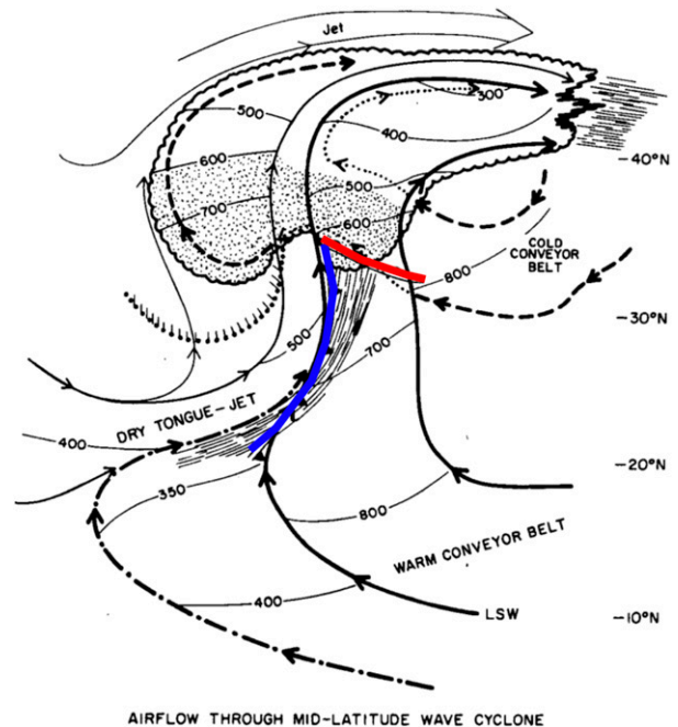
FIG. 16-16. Schematic composite of the three-dimensional air flow through a midlatitude cyclone. Heavy solid streamlines depict the warm conveyor belt, dashed lines represent the cold conveyor belt (drawn dotted where it lies beneath the warm conveyor belt or dry airstream), and the dot-dashed line represents flow originating at midlevels within the tropics. Thin solid streamlines pertain to dry air that originates at upper levels west of the trough. Thin solid lines denote the heights of the airstreams (hPa) and are approximately normal to the direction of the respective air motion (isobars are omitted for the cold conveyor belt where it lies beneath the warm conveyor belt or beneath the jet streamflow). Scalloping marks the regions of dense clouds at the upper and middle levels, stippling indicates sustained clouds at the upper and middle levels, and streaks denote thin cirrus. Small dots with tails mark the edge of the low-level stratus. The major upper-tropospheric jet streams are labeled "Jet" and "Dry Tongue Jet." The limiting streamline for the warm conveyor belt is labeled "LSW." Warm and cold fronts are identified by the thick red and blue lines, respectively, and coincide with the boundaries between airstreams. The figure and caption are adapted from Carlson (1980, his Fig. 9).
