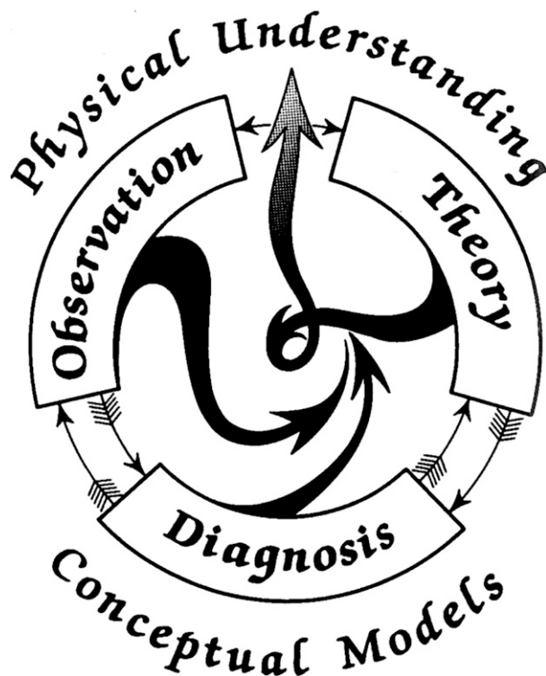
FIG. 16-2. Physical understanding and conceptual representation through the union of theory, diagnosis, and observation. The figure and caption are from Shapiro et al. (1999, their Fig. 1).
