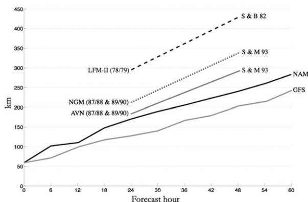
FIG. 16-26. Extratropical cyclone displacement errors (km) vs forecast hour for the LFM-II (Silberberg and Bosart 1982; 1978/79 cool season for CONUS and oceans), the NGM and AVN (Smith and Mullen 1993; 1987/88 and 1989/90 cool seasons for the Atlantic), and the NAM and GFS (2002–07 cool seasons) (Atlantic). The figure is from Charles and Colle (2009a, their Fig. 16).
