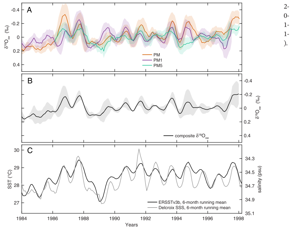
Figure 7. (a) Seasonal \delta^{18}\text{O}_{\text{sw}} reconstructions from cores PM (orange), PM1 (purple), and PM5 (green), compared to (b) a composite of all three records in (a), and (c) six-month running means of temperature (black line) from ERSSTv3b and SSS (gray line) from Delcroix et al. (2011). Shading in (a) represents the compounded 2\sigma uncertainty for each record, accounting for analytical uncertainties and Sr/Ca-SST calibration errors, whereas the shading in (b) (gray shading) is the standard error ( 2\sigma ) compounded with the uncertainties shown in (a).
