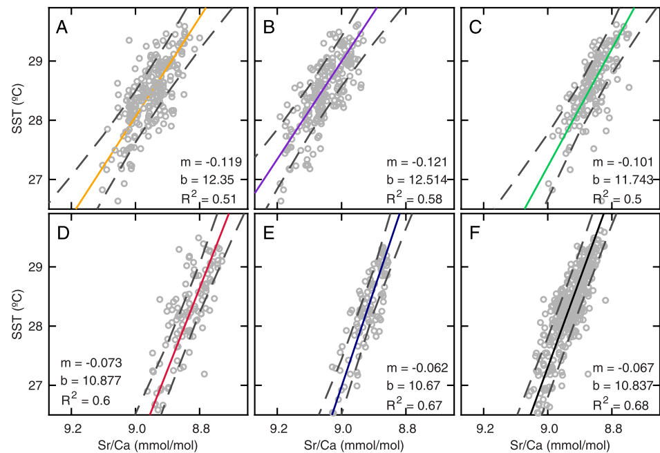
Figure 4. Coral Sr/Ca-SST calibrations for cores (a) PM, (b) PM 1 , (c) PM 5 , (d) P13, (e) PAL2, and (f) coral Sr/Ca composite. Coral Sr/Ca and SST pairs used in each calibration are shown in gray, m and b represent the slope and intercept for the equation Sr/Ca = m * SST + b , and dashed lines represent the 95% prediction bounds for each calibration.
