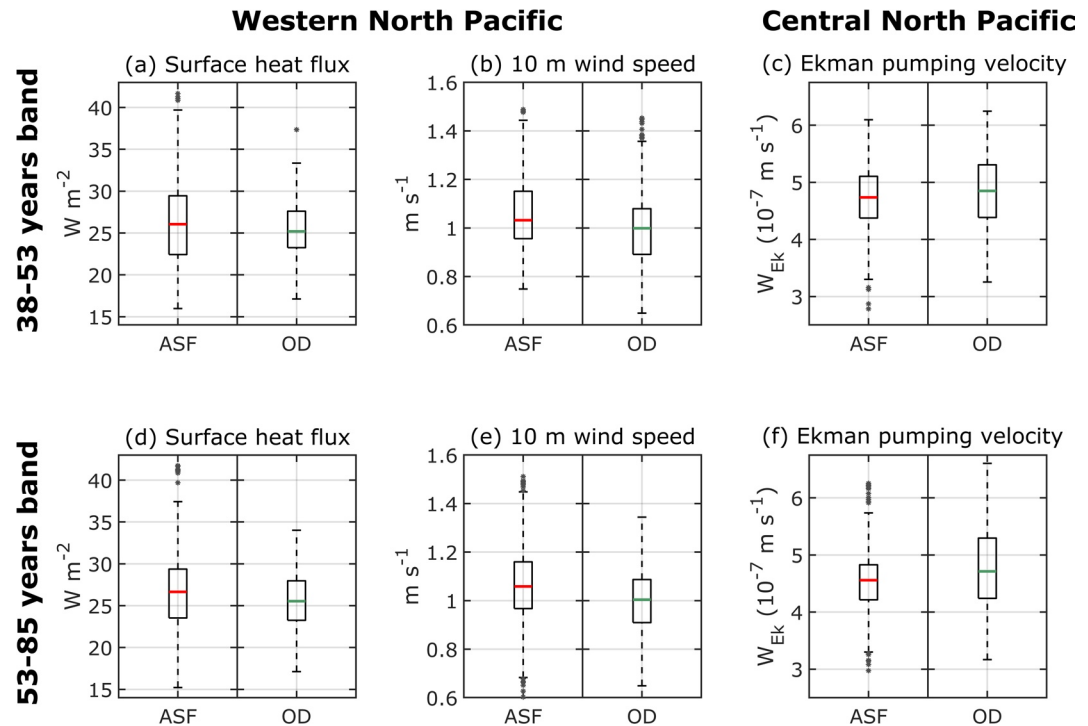
Figure 4. Box-and-whisker plots for 25-year moving standard deviation of anomalous winter (DJFM) (a) net surface heat flux, (b) 10 m wind speed averaged over a Northwest Pacific region (140–160°E, 29–37°N; magenta box in Figure 3), and (c) Ekman pumping velocity averaged in a central North Pacific region (180–140°W, 29–37°N; green box in Figure 3) in the air-sea flux (ASF) and ocean dynamics (OD) epochs based on the 38–53 years band-pass filtering. The solid boxes indicate 25th and 75th percentiles and thick red and green lines in the box denote the median values. The whiskers (upper and lower dashed lines) correspond to the 0.7th and 99.3rd percentiles ( \pm 2.7\sigma ) of the samples. Asterisks denote the outliers (beyond the whisker). (d–f) Same as (a–c) but for the ASF and OD epochs based on the 53–85 years band-pass filtering. The two box-whisker plots in all six panels are significantly different at 95% based on the two-sided Mann-Whitney-Wilcoxon test.
