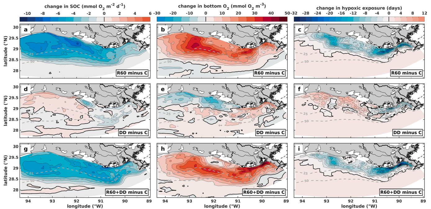
Figure 8. Changes in sediment oxygen consumption (SOC; left column), bottom oxygen concentration (middle column), and cumulative hypoxic exposure (right column) relative to the control simulation (C) for the different model scenarios and averaged over summer (June–August) 2001 to 2011: (a, b, c) 60% N load reduction (R60); (d, e, f) discharge diversion (DD); (g, h, i) combined 60% N load reduction and discharge diversion (R60 + DD). Thick isopleths indicate zero change. Gray dashed lines indicate isobaths (in meters).
