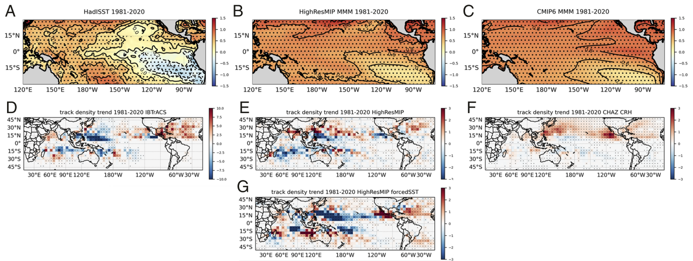
Fig. 3. Historical trends (1981 to 2020) in SST from (A) observations, (B) HighResMIP simulations, and (C) CMIP6 historical simulations; and in tropical cyclone track density from (D) observations, (E) HighResMIP coupled historical simulations, (F) CHAZ, downscaling the same CMIP6 models as in (C), and (G) HighResMIP atmosphere-only simulations using observed SST up to 2014 and observed SST blended with CMIP5 RCP8.5 SST from 2015 to 2020. The units are similar to Fig. 1 but over 40 y.
