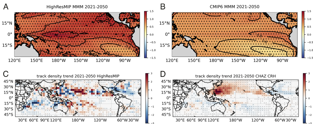
Fig. 1. Projected trends in ^{\circ}\text{C} over 2021–2050 in tropical Pacific SST from the multimodel means of (A) coupled HighResMIP models under the SSP5-8.5 scenario, and (B) 12 CMIP6 models under the SSP2-4.5 scenario; and projected trends in number of storm per grid box over 2021–2050 in track density of TCs simulated by (C) the same HighResMIP models under the SSP5-8.5 scenario tracked with TempestExtremes, and (D) CHAZ, downscaling the same CMIP6 models as in (B). Note that different future scenarios are used for the CHAZ and HighResMIP data, so that the magnitudes of the trends should not be compared, only the spatial patterns.
