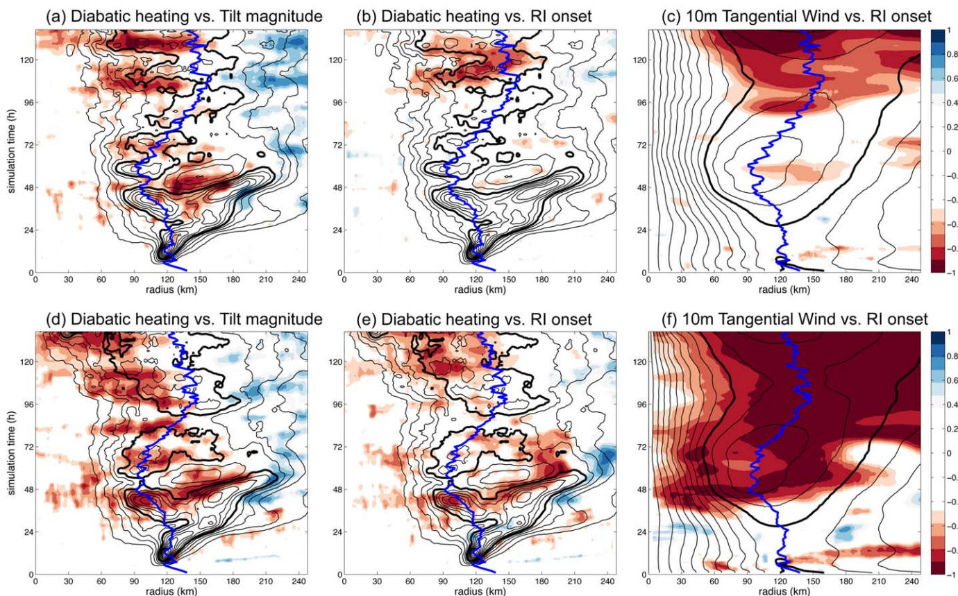
Figure 15. Radius-time plots. The black contours are the composite azimuthally averaged (a, b, d, and e) column-integrated diabatic heating (interval 0.002 \text{ K s}^{-1} , thick black line for 0.01 \text{ K s}^{-1} ) and (c and f) tangential wind (interval 1 \text{ m s}^{-1} , thick black line for 10 \text{ m s}^{-1} ). The blue thick line is the radius of maximum tangential wind. The shading is (a and d) correlation between diabatic heating and tilt magnitude at the same time, (b and e) correlation between diabatic heating and rapid intensification onset times, and (c and f) correlation between tangential wind and rapid intensification onset times. The shading is from -1 to 1 with 0.1 interval and small correlation ( <0.5 ) masked out. (first row) SH6-STD0.1 and (second row) SH6-STD0.5. Contours are not showing the whole range in order to leave the shading more clear to be seen.
