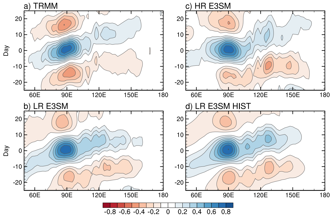
Figure 1. Longitude–lag diagram of equatorial ( 10^{\circ}\text{S} – 10^{\circ}\text{N} ) precipitation regressed against intraseasonal precipitation anomalies in the Indian Ocean reference region ( 5^{\circ}\text{S} – 5^{\circ}\text{N} , 85 – 95^{\circ}\text{E} ) during NDJFMA for (a) Tropical Rainfall Measuring Mission and (b–d) Energy Exascale Earth System Model version 1 simulations. For (b) and (c) low resolution and high resolution simulations of a recent 20-year period are used, while for (d) the lag–regression diagram is first obtained from each of the five ensemble members of the CMIP6 Historical simulation (1850–2014) and then averaged across all ensemble members.
