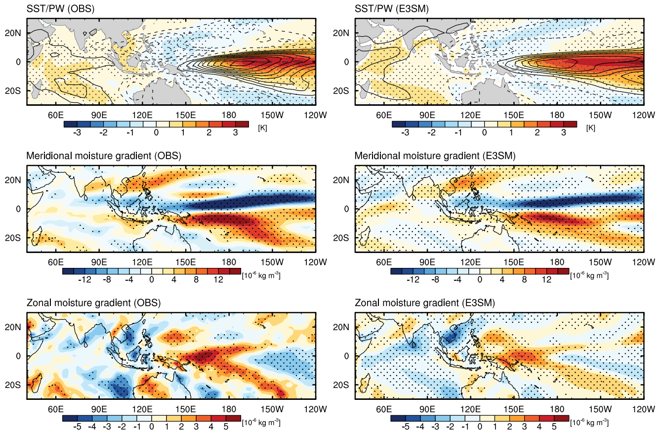
Figure 13. Differences between the El Niño and La Niña years in DJF mean state: (left) observations and (right) 5-ensemble CMIP6 Historical simulation made with low resolution Energy Exascale Earth System Model version 1 (LR E3SMv1). (top) Sea surface temperature (K, shaded) and precipitable water (PW; \text{kg m}^{-2} , contour), (middle) meridional and (bottom) zonal gradient of PW ( \times 10^{-6} \text{ kg m}^{-3} ). Black dots indicate the differences are statistically significant at the 95% confidence level. For observations, 11 El Niño and 14 La Niña years were used, while 146 El Niño and 164 La Niña years were used for LR E3SMv1.
