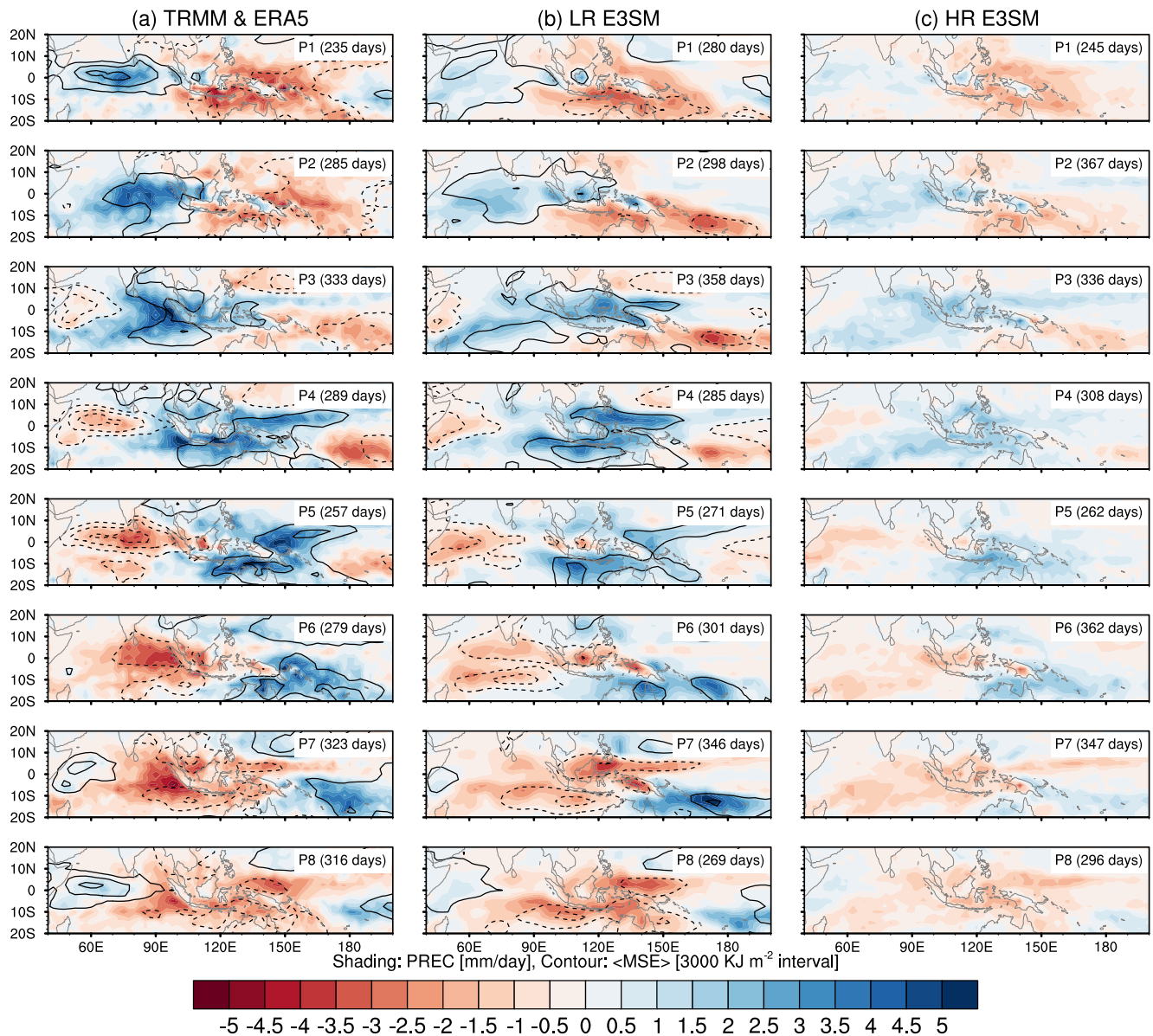
Figure 3. Madden-Julian oscillation (MJO) life cycle composite maps of intraseasonal precipitation ( \text{mm day}^{-1} , shaded) and column-integrated moist static energy (MSE) anomalies ( \text{kJ m}^{-2} , contour) obtained from each Real-Time Multivariate MJO (RMM) phase (RMM amplitude >1 ) during NDJFMA: (a) observations, (b) low resolution Energy Exascale Earth System Model version 1 (E3SMv1), and (c) high resolution E3SMv1. The contour interval for column-integrated MSE anomalies is 3000 \text{ kJ m}^{-2} . The number of days used in each phase composite is indicated in the parentheses.
