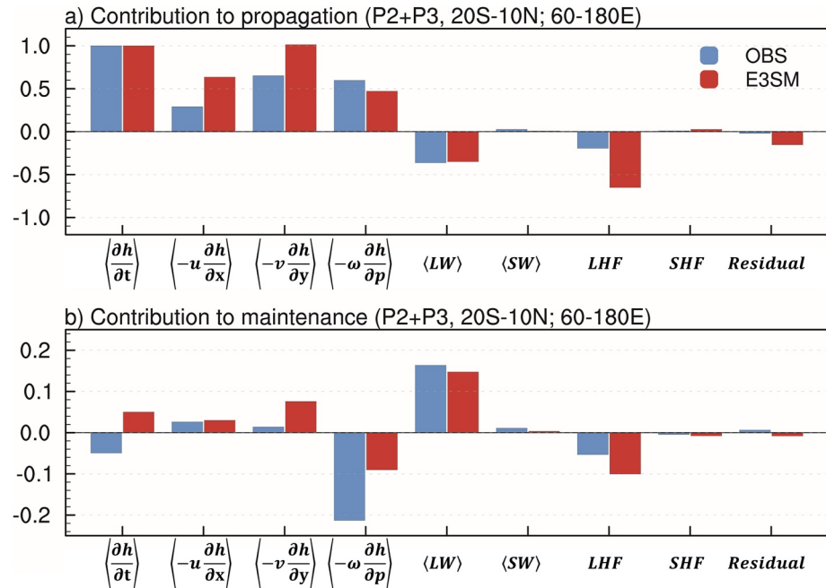
Figure 5. Contribution of each moist static energy budget term to the (a) propagation and (b) maintenance of the Madden-Julian oscillation (MJO) during Real-Time Multivariate MJO phases 2 and 3 over the Indo-Pacific warm pool (20°S–10°N and 60–180°E) during NDJFMA. Blue and red bars indicate results from observations and low resolution Energy Exascale Earth System Model version 1, respectively.
