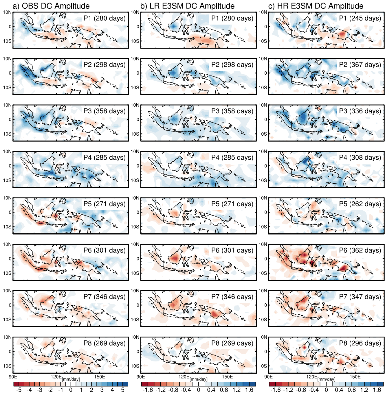
Figure 8. Madden-Julian oscillation (MJO) life cycle composite maps of anomalous diurnal harmonic amplitude of precipitation ( \text{mm day}^{-1} ) obtained from each Real-Time Multivariate MJO phase during NDJFMA: (a) Tropical Rainfall Measuring Mission, (b) low resolution Energy Exascale Earth System Model version 1 (E3SMv1), and (c) high resolution E3SMv1.
