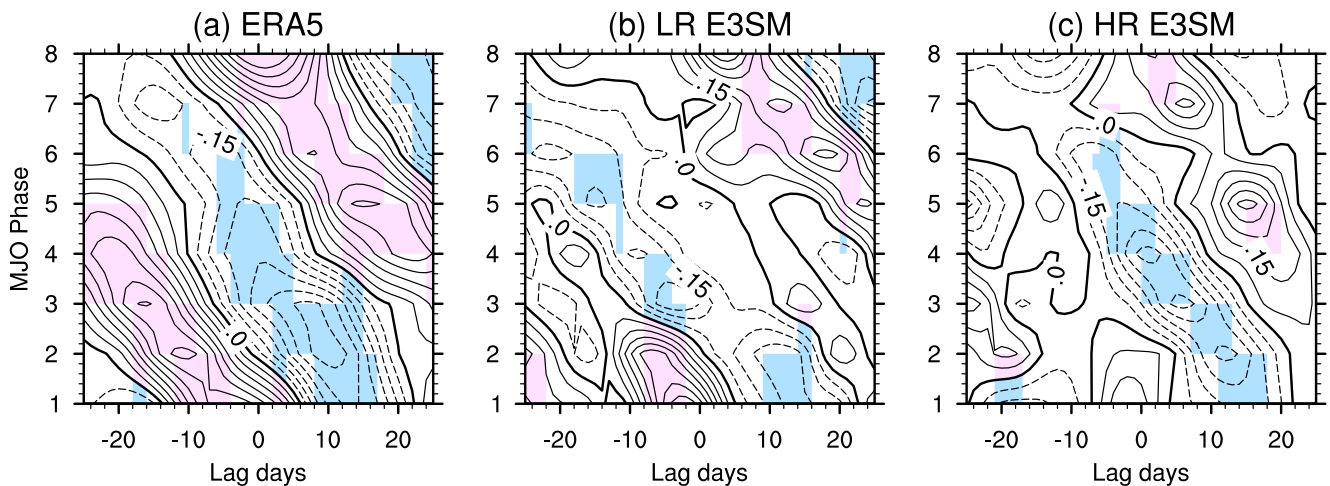
Figure 11. Lead-lag composite of the Pacific North American index around strong Madden-Julian oscillation (MJO) days for each MJO phase during NDJFMA: (a) ERA5, (b) low resolution Energy Exascale Earth System Model version 1 (E3SMv1), and (c) high resolution E3SMv1. Pink and blue shading indicates that positive and negative composite values are statistically significant at the 95% confidence level.
