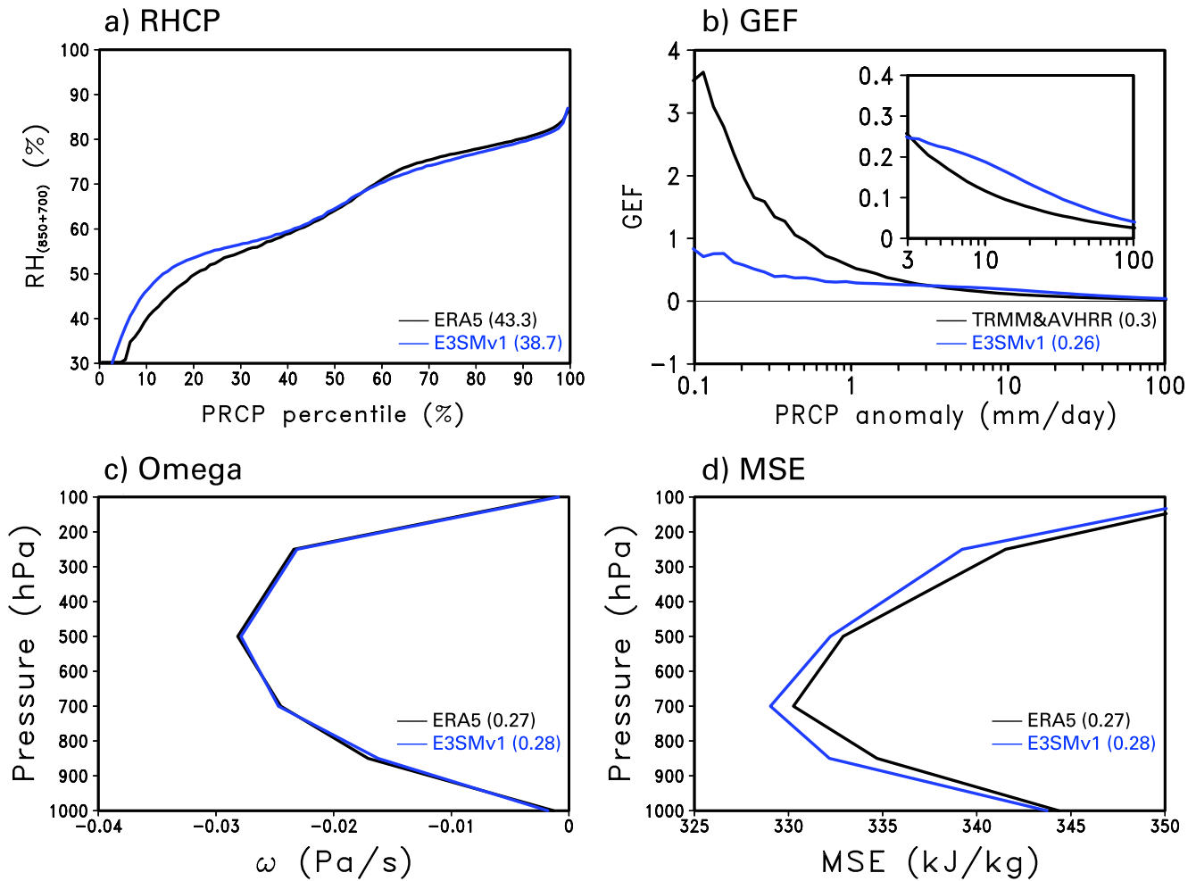
Figure 16. Process-oriented Madden-Julian oscillation diagnostics: (a) the relative humidity composite based on precipitation percentile (RHCP, %), (b) the greenhouse enhancement factor (GEF, unitless), and the vertical profiles of the mean state (c) pressure velocity ( \text{Pa s}^{-1} ) and (d) moist static energy (MSE, \text{kJ kg}^{-1} ) from observations (black) and low resolution Energy Exascale Earth System Model version 1 (blue). The pressure velocity and MSE profiles are used for the calculation of normalized gross moist stability (NGMS). The Indo-Pacific warm pool area ( 60\text{--}180^\circ\text{E} , 15^\circ\text{S}\text{--}15^\circ\text{N} ) excluding land grid points is used for all the process-oriented diagnostics. Numbers in parentheses next to data labels denote the process-oriented metric values of RHCP, GEF, and NGMS.
