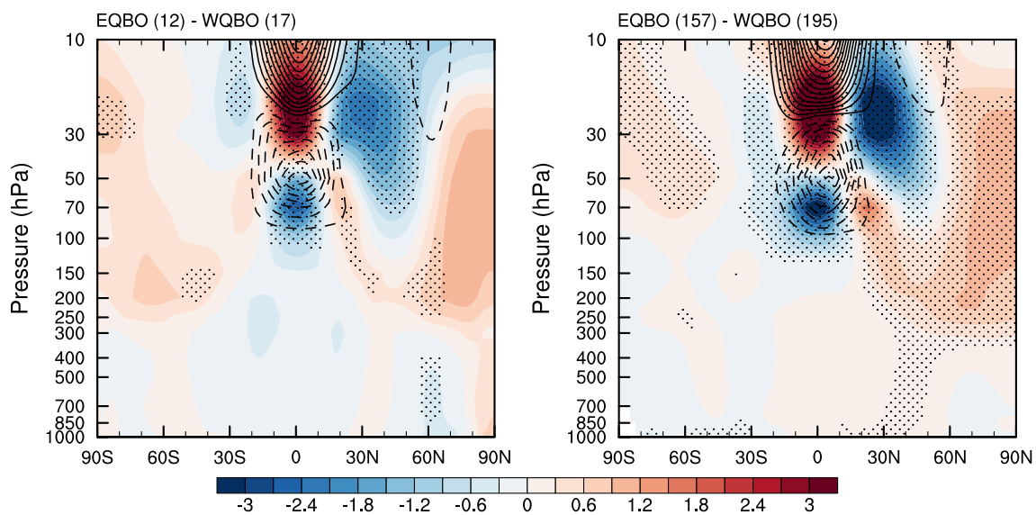
Figure 15. Differences between the EQBO and WQBO years in DJF-mean zonal-mean temperature (K, shaded) and zonal wind ( \text{m s}^{-1} , contour): (left) observation and (right) 5-ensemble CMIP6 Historical simulation made with low resolution Energy Exascale Earth System Model version 1. The contour interval is 3 \text{ m s}^{-1} and solid and dashed contours indicate positive and negative anomalies, respectively. Zero line is omitted. Black dots indicate shaded differences are statistically significant at the 95% confidence level.
