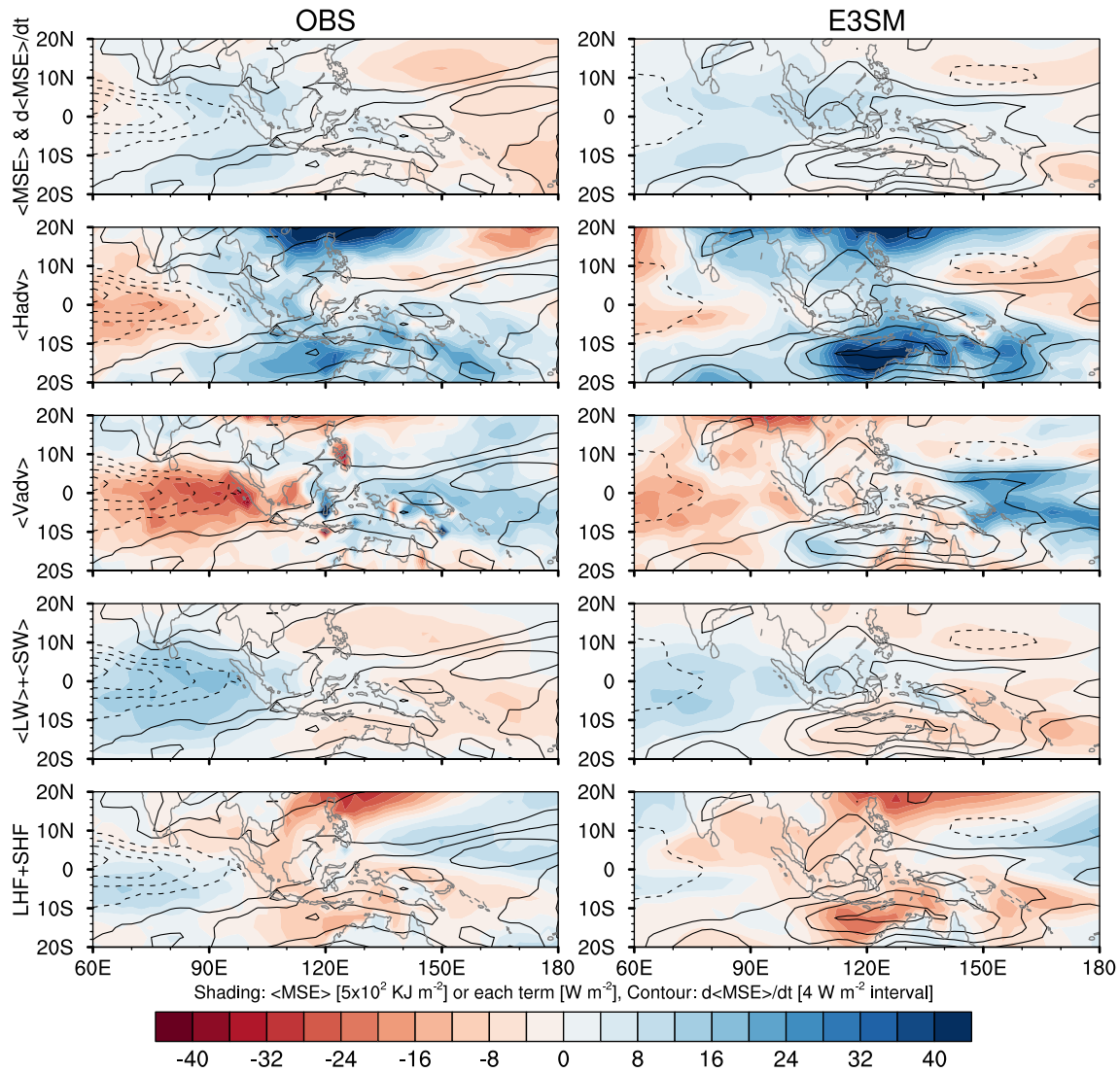
Figure 4. (first row) Column-integrated moist static energy (MSE) anomalies ( \text{kJ m}^{-2} , shaded) and total MSE tendency ( \text{W m}^{-2} , contour) composited for Madden-Julian oscillation phases 2 and 3: (left) ERA5 and (right) low resolution Energy Exascale Earth System Model version 1. (second to fifth rows) Same as the first row, except that shading indicates horizontal advection, vertical advection, radiative heating, and surface turbulent fluxes, respectively. The contour interval for total MSE tendency is 4 \text{ W m}^{-2} .
