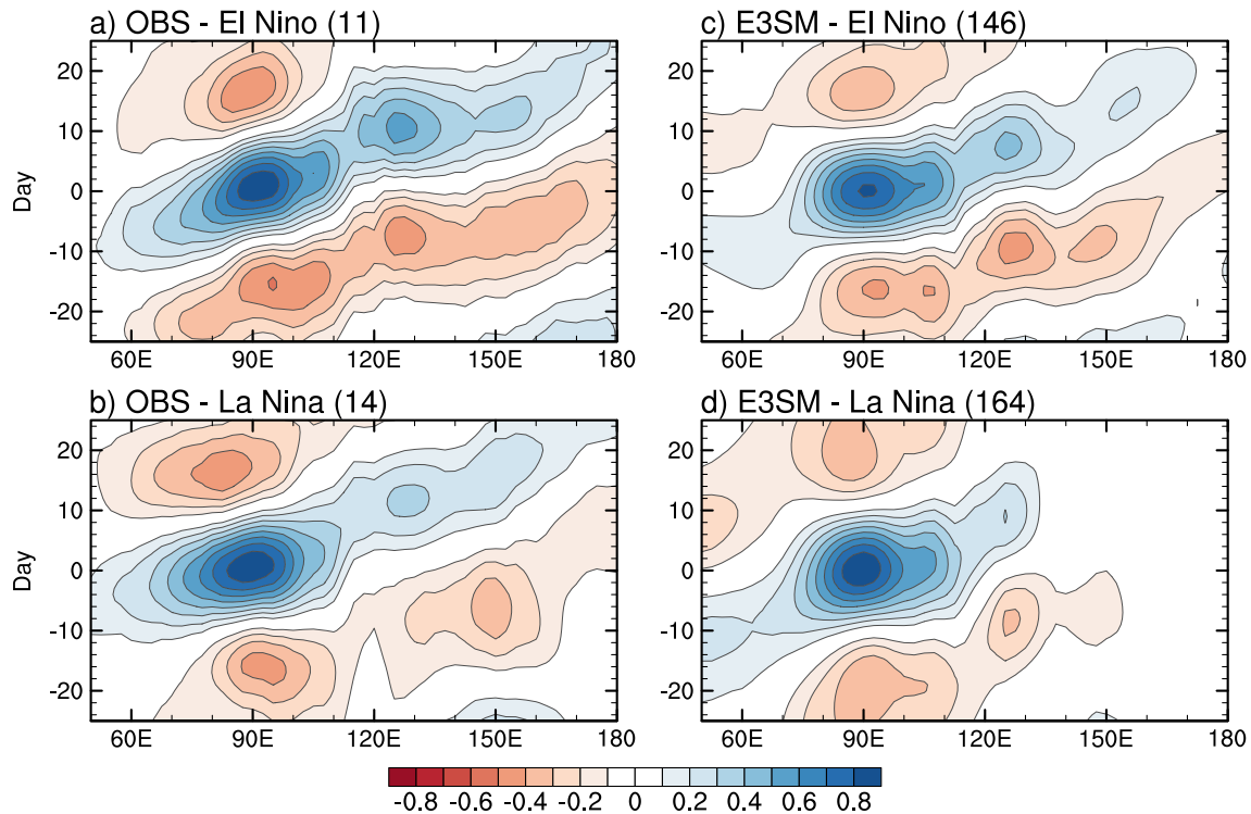
Figure 12. Longitude–lag diagram of equatorial ( 10^{\circ}\text{S} – 10^{\circ}\text{N} ) outgoing longwave radiation (OLR) regressed against intraseasonal OLR anomalies in the Indian Ocean reference region ( 5^{\circ}\text{S} – 5^{\circ}\text{N} , 85^{\circ} – 95^{\circ}\text{E} ) during DJF for the El Niño and La Niña years from (left) observations and (right) 5-ensemble CMIP6 Historical simulation made with low resolution Energy Exascale Earth System Model version 1 (LR E3SMv1). Numbers in parentheses denote the number El Niño and La Niña years. For observations and LR E3SMv1, El Niño and La Niña years are defined as the years with sea surface temperature anomalies averaged over the Niño3.4 region ( 5^{\circ}\text{S} – 5^{\circ}\text{N} , 170^{\circ} – 120^{\circ}\text{W} ) being higher than its 0.5 standard deviation and lower than its -0.5 standard deviation, respectively.
