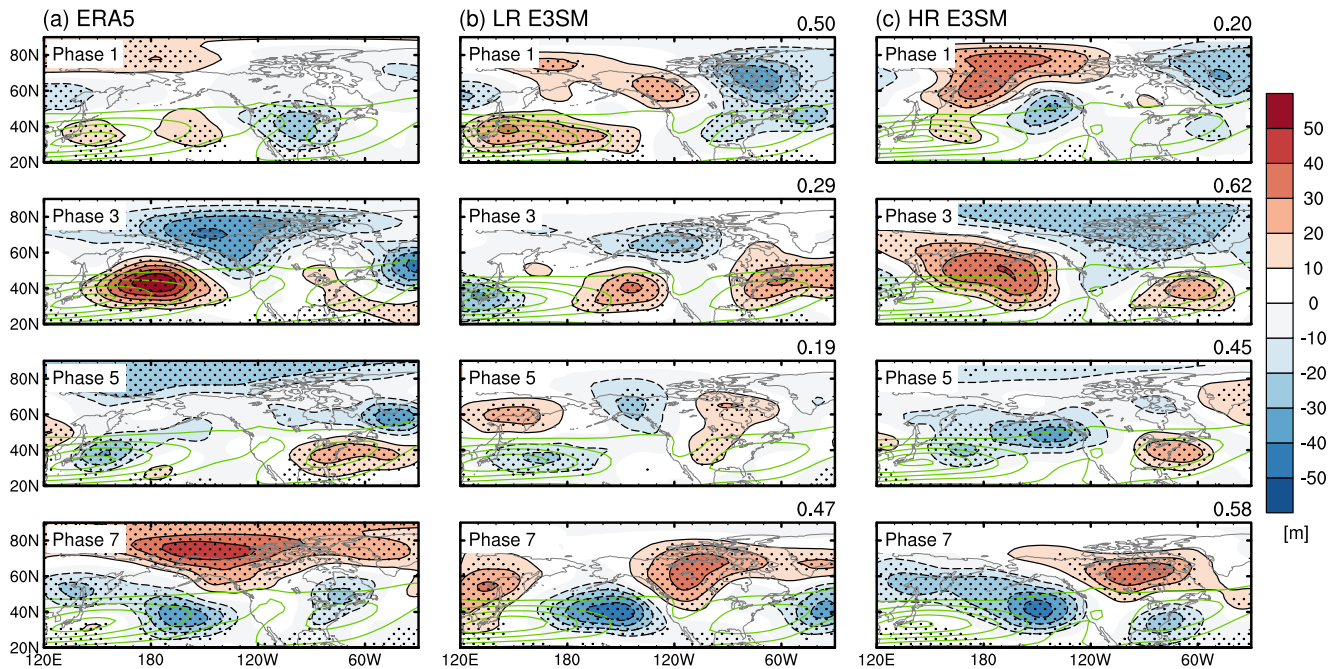
Figure 10. Madden-Julian oscillation (MJO) life cycle composite maps of 5–9 days average 500-hPa geopotential height anomalies (m, shaded) obtained from the selected four Real-Time Multivariate MJO phases during NDJFMA. Green contours indicate the climatological 300-hPa zonal wind ( \text{m s}^{-1} , contour interval: 10 \text{ m s}^{-1} ). The geopotential height anomalies that are statistically significant at the 95% confidence level are indicated by the dots. For E3SM simulation results, the pattern correlation with the observed anomalies over the domain covered by figures ( 20\text{--}90^\circ\text{N} , 120\text{--}330^\circ\text{E} ) is indicated at the right top of each panel.
