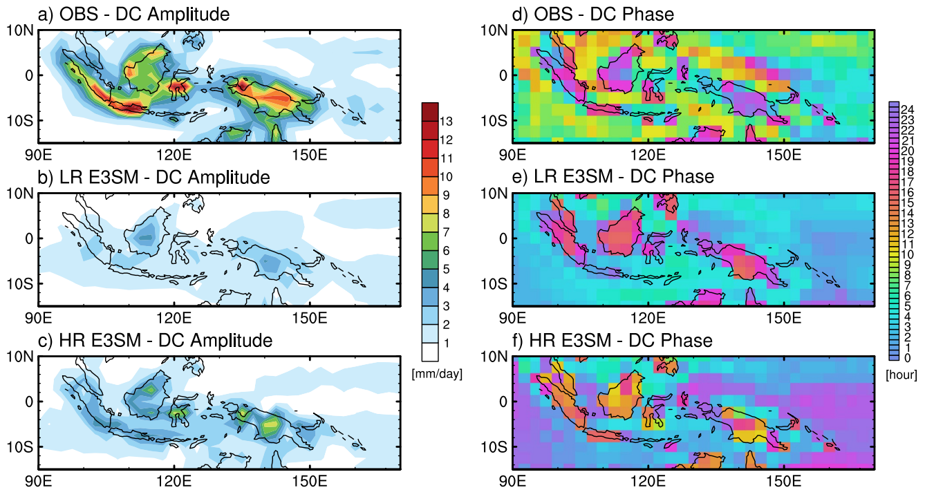
Figure 7. Climatological (left) amplitude ( \text{mm day}^{-1} ) and (right) phase (hour) of the diurnal harmonic of precipitation from (top) Tropical Rainfall Measuring Mission, (middle) low resolution Energy Exascale Earth System Model version 1 (E3SMv1), and (bottom) high resolution E3SMv1 during NDJFMA.
