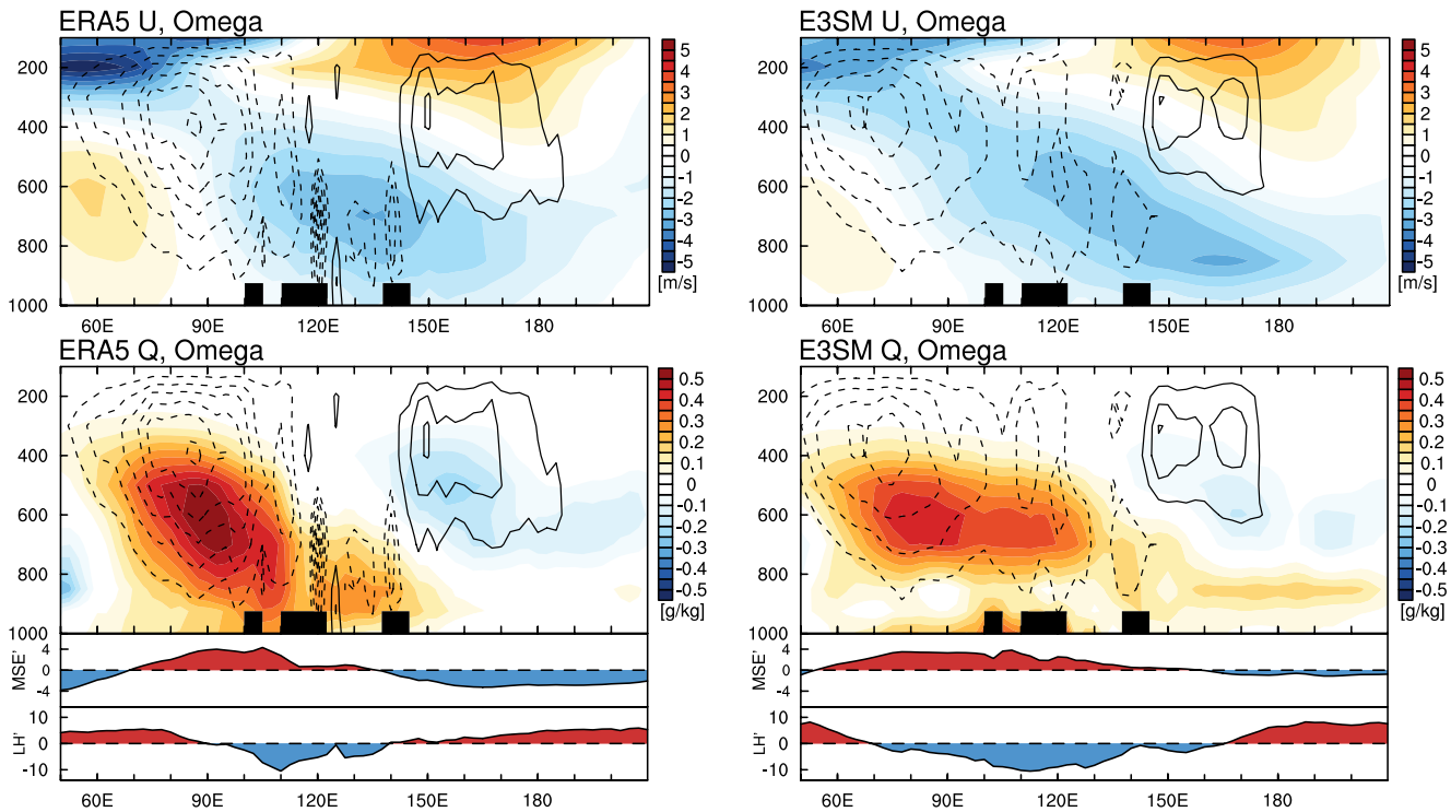
Figure 6. (top) Intraseasonal zonal wind ( \text{m s}^{-1} , shaded) and pressure velocity ( \text{Pa s}^{-1} , contour) anomalies averaged over the equatorial band ( 10^{\circ}\text{S} – 10^{\circ}\text{N} ) composited for Madden-Julian oscillation phases 2 and 3: (left) ERA5 and (right) low resolution Energy Exascale Earth System Model version 1. (bottom) Same as the top panels, except for intraseasonal specific humidity anomalies ( \text{g kg}^{-1} ) are shaded. The contour interval for pressure velocity is 0.005 \text{ Pa s}^{-1} . Line graphs at the bottom indicate column-integrated intraseasonal moist static energy ( \times 10^4 \text{ kJ m}^{-2} ) and latent heat flux ( \text{W m}^{-2} ) anomalies.
