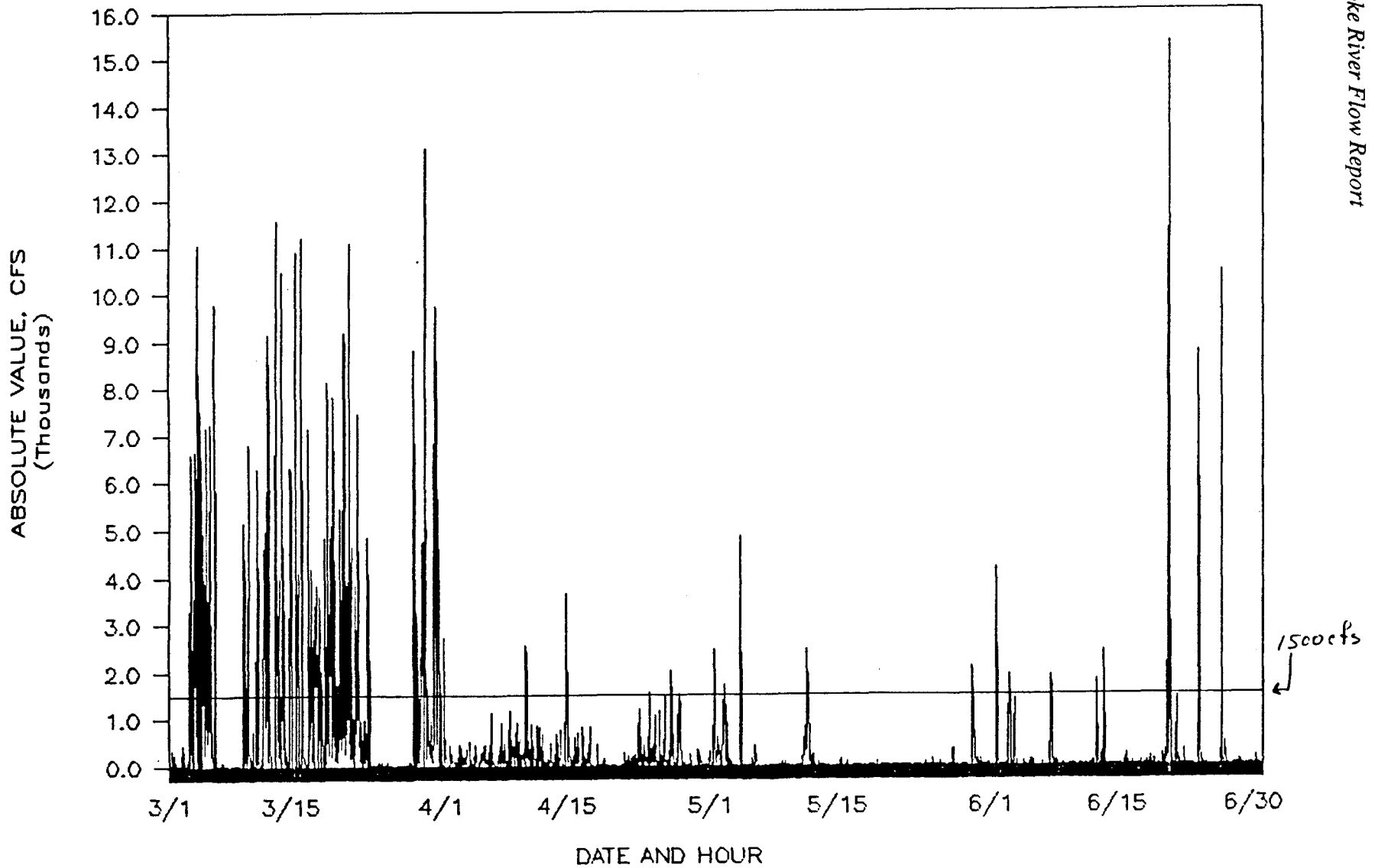
Figure 9. Hourly comparisons of differences in rate of Roanoke River flow (thousands of cfs) below the Roanoke Rapids Reservoir for March-June 1988 relative to the recommended change of 1,500 cfs/hour.
