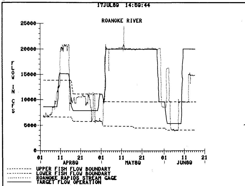
Figure 16. U.S. Army Corps of Engineers, Wilmington District, modeling of 1989 Kerr Reservoir water releases under a "target flow operation" scenario showing (a) hypothetical changes in Kerr surface water elevation relative to the Rule Curve and observed values, and (b) river flow downstream of Roanoke Rapids dam relative to the Q1-Q3 bounds and observed values.
