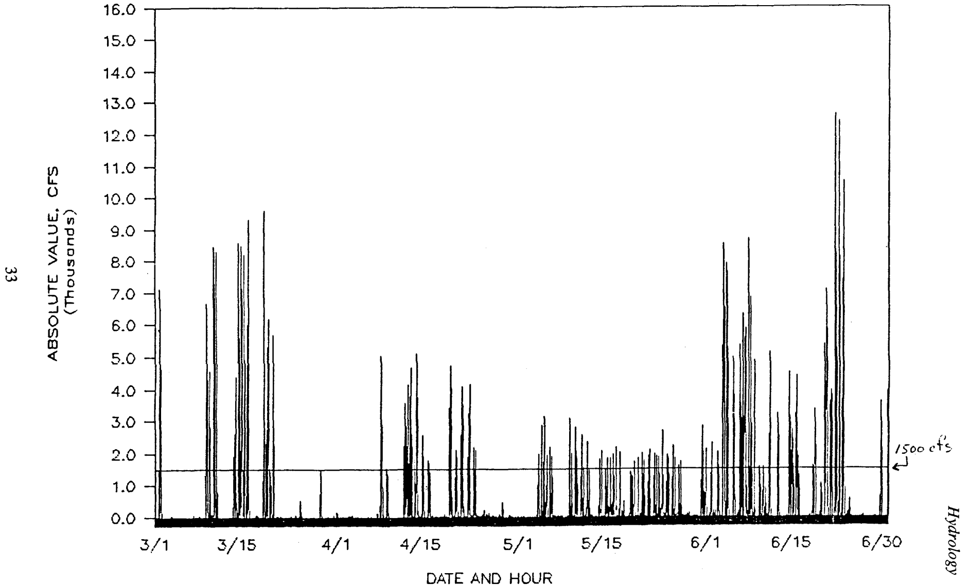
Figure 8. Hourly comparisons of differences in rate of Roanoke River flow (thousands of cfs) below the Roanoke Rapids Reservoir for March-June 1989 relative to the recommended change of 1,500 cfs/hour.
