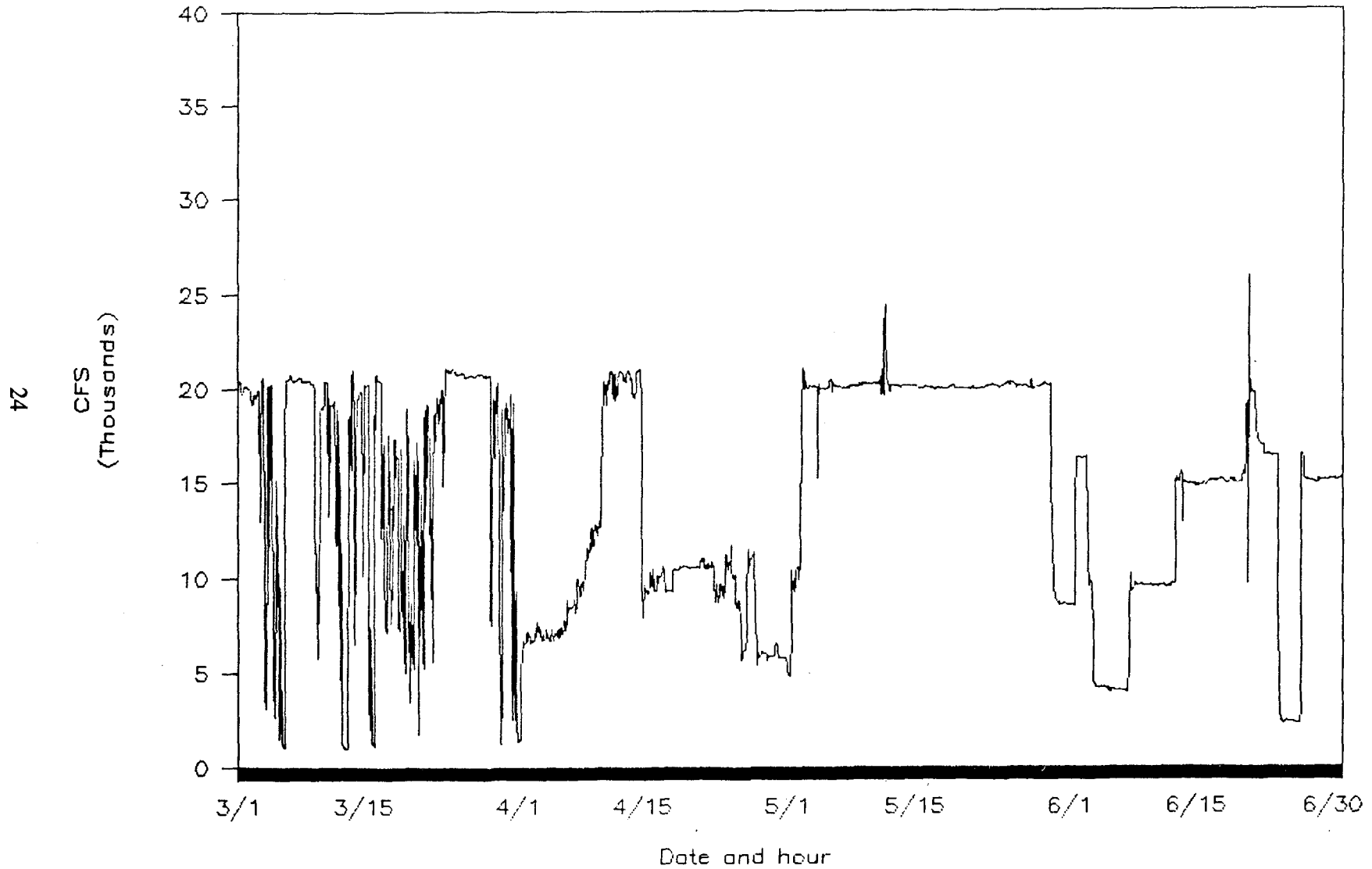
Figure 7. Hourly record of Roanoke River flows (cfs) downstream of the Roanoke Rapids Reservoir (USGS data), March through June 1989.
