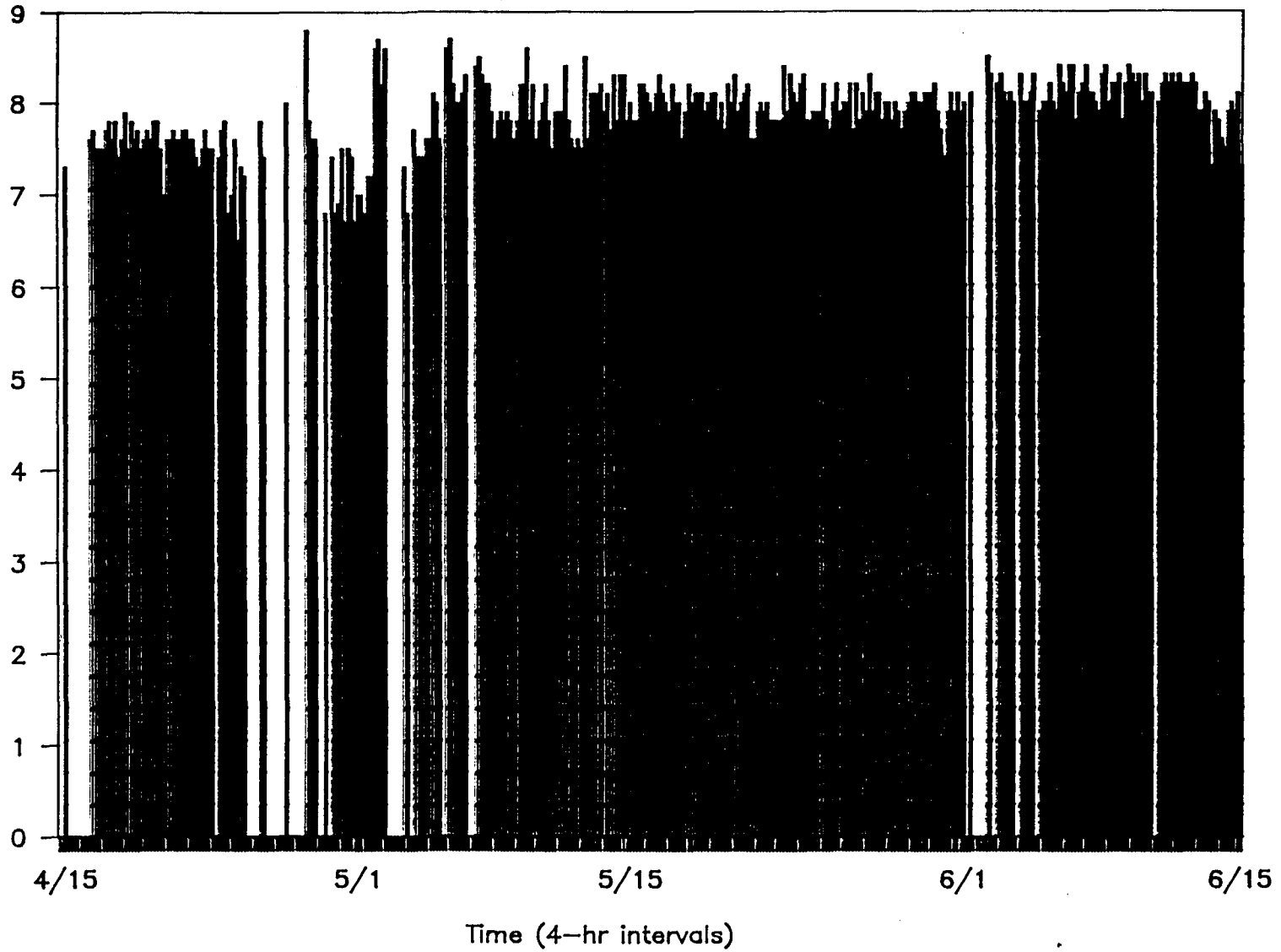
Figure 23. Surface water pH of the Roanoke River at Barnhill's Landing (RM 117) from 15 April to 15 June 1989.
