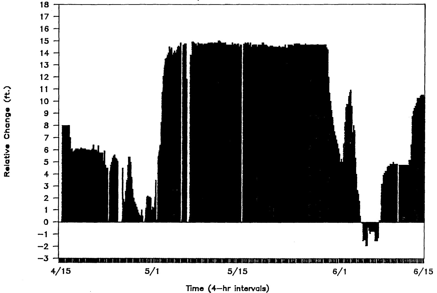
Figure 20. Relative change in stage of the Roanoke River at Barnhill's Landing (RM 117) from 15 April to 15 June 1989.
