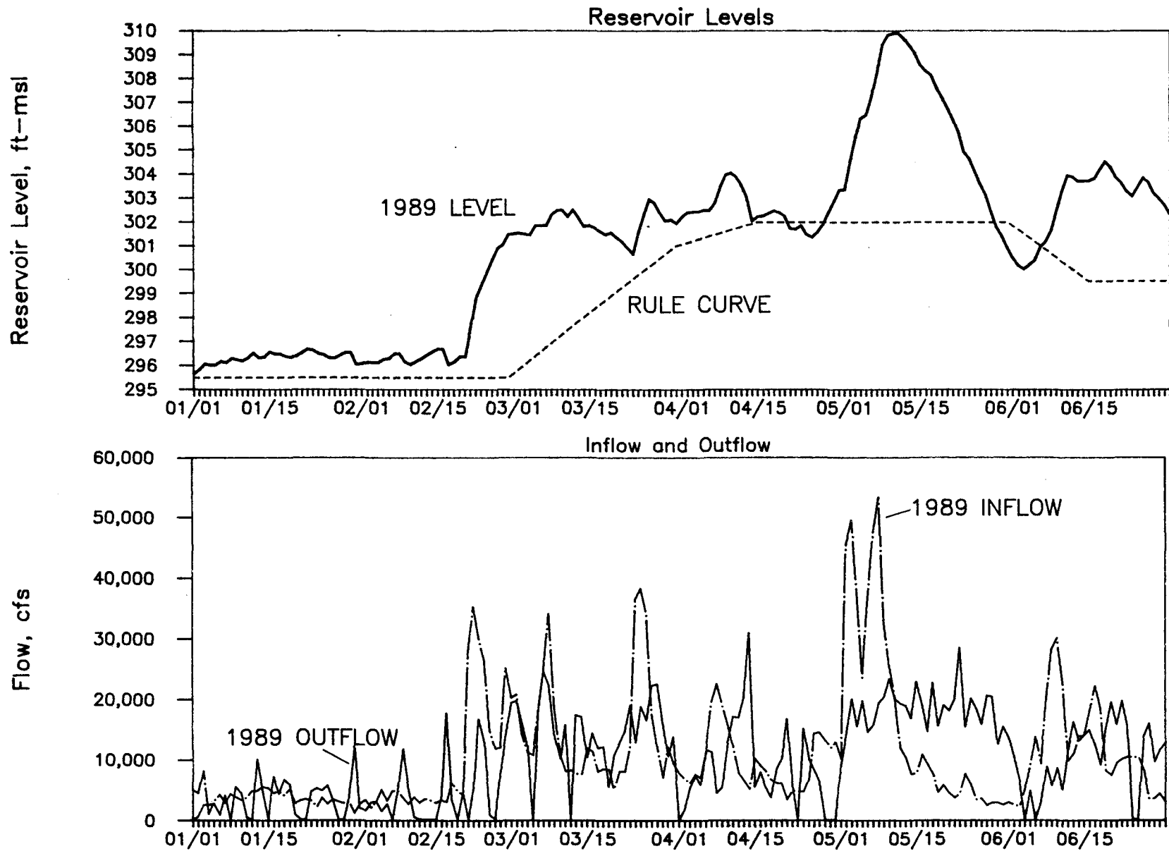
Figure 5. Kerr Reservoir daily elevations (feet above mean sea level) for 1989 and inflow and outflow in thousands of cubic feet per second (cfs).
