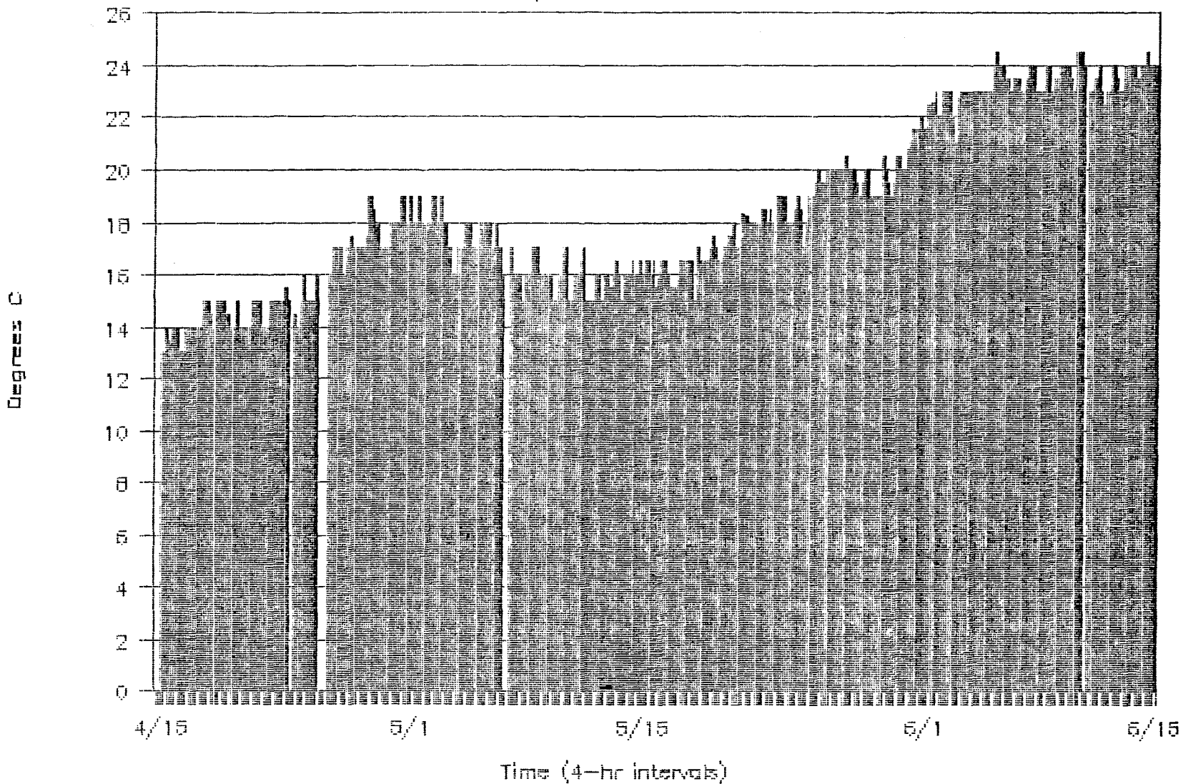
Figure 22. Surface water temperature (C) of the Roanoke River at Barnhill's Landing (RM 117) from 15 April to 15 June 1989.
