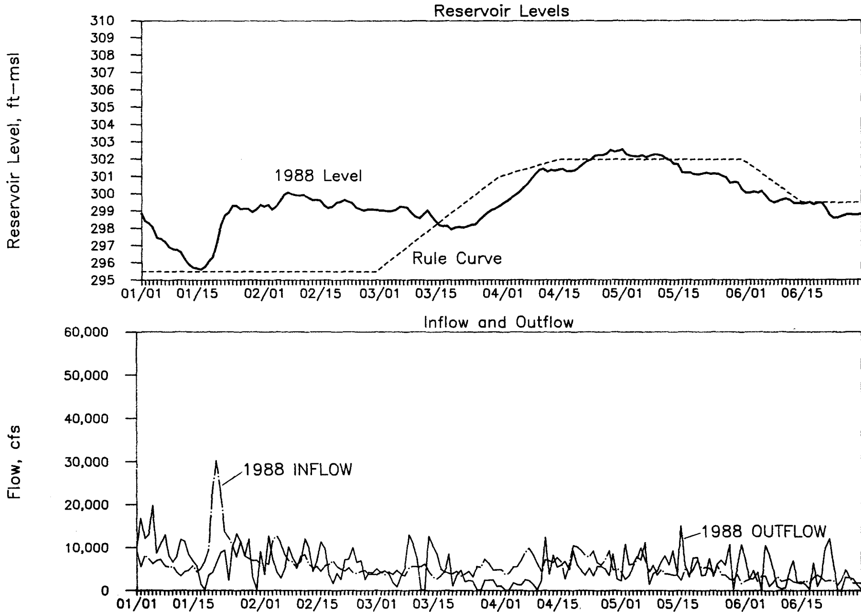
Figure 4. Kerr Reservoir daily elevations (feet above mean sea level) for 1988 and inflow and outflow in thousands of cubic feet per second (cfs).
