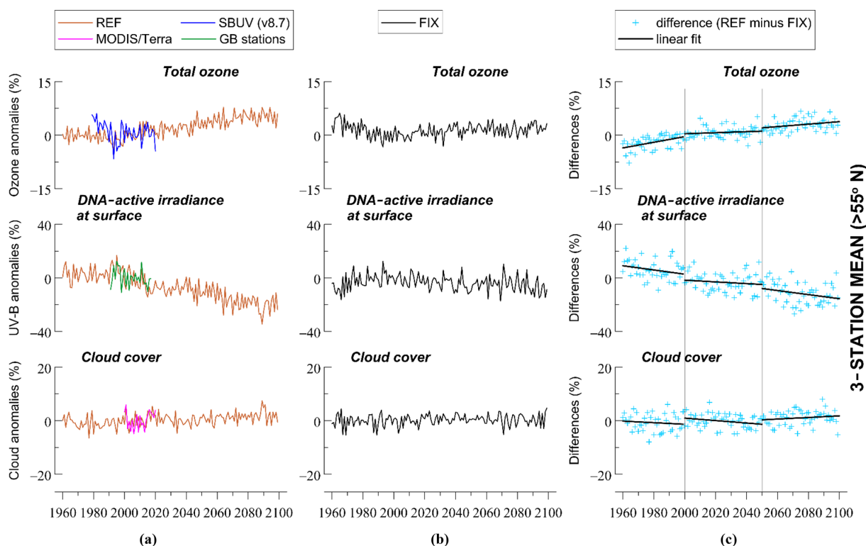
Figure 5. Same as Fig. 4 but for three UV stations in the northern high latitudes (> 55° N). The y axes in (a) and (b) show averages of monthly de-seasonalized anomalies from March to September.
