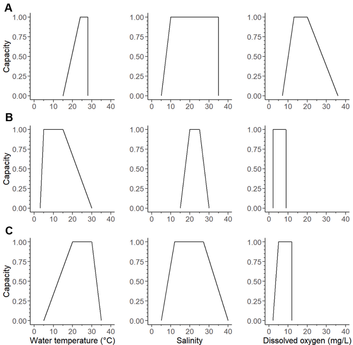
Fig. 2. Functional response curves indicative of the temperature (°C), salinity and dissolved oxygen (mg/L) tolerance capacities for adult striped bass (A), blue crab (B), and oysters (C; Knoche et al., 2020; Hill et al., 1989a; Hill et al., 1989b; Secor et al., 1995; Fisher, 1999; Secor et al., 2000; Jensen et al., 2005; Rome et al., 2005; Eastern Oyster Biological Review Team, 2007). The environmental parameter values encompassed by each curve represent the overall environmental tolerance range for each species, and the values under the flat line at the top of each curve are the optimum conditions.
