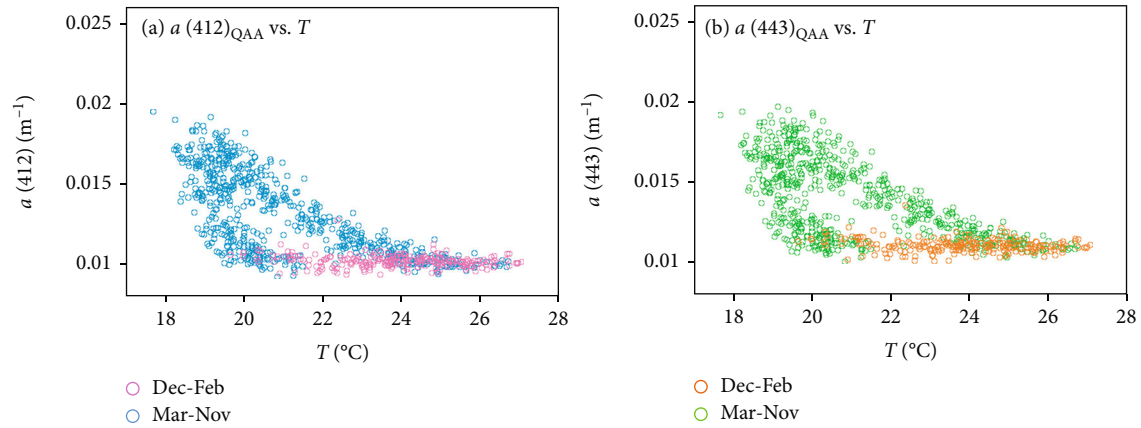
FIGURE 4: Relationships between T and a(412)_{\text{QAA}} (a) and a(443)_{\text{QAA}} (b) for waters of cSPG during the period of July 2002 to July 2020.
