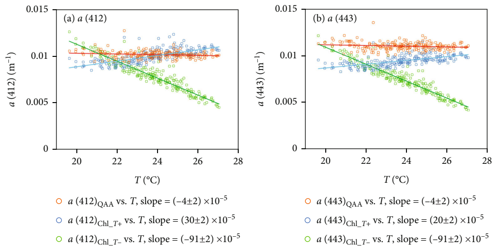
FIGURE 5: Relationships between T and a(412) (a) and a(443) (b) for waters of cSPG during December–February. The orange, blue, and green circles represent the results of a(\lambda)_{\text{QAA}} versus T , a(\lambda)_{\text{Chl}_T+} versus T , and a(\lambda)_{\text{Chl}_T-} versus T , respectively.
