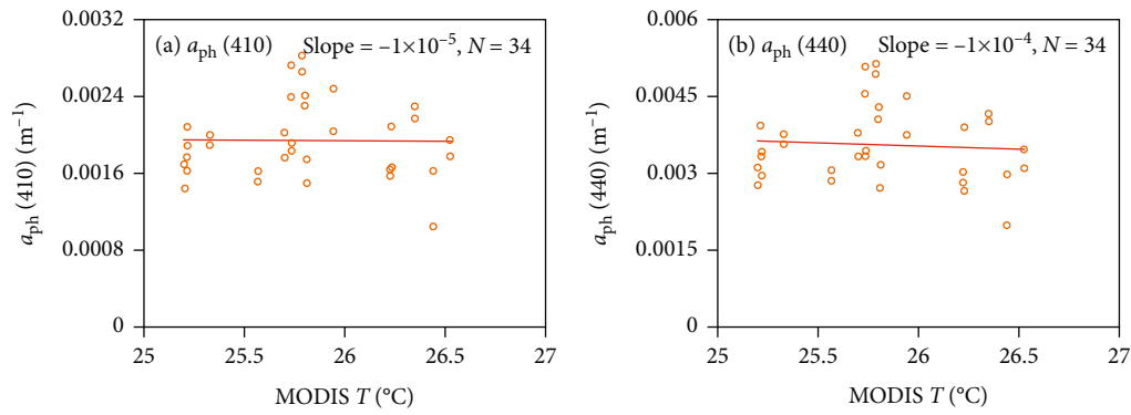
FIGURE 7: Relationship between T and field measured a_{\text{ph}}(410) (a) and a_{\text{ph}}(440) (b) at HOT for months of July–September in the period of 2006–2013.
