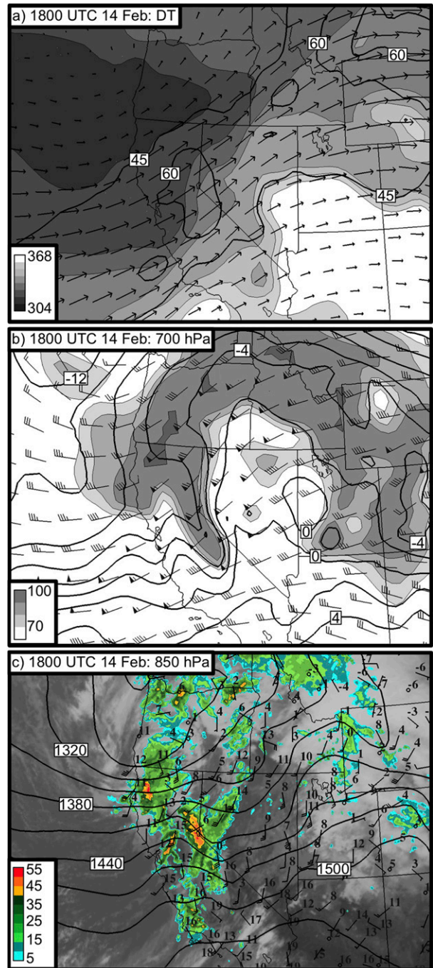
FIG. 4. Regional analyses from the RUC2 at 1800 UTC 14 Feb 2000. (a) Dynamic tropopause (DT) potential temperature (shaded every 8 K following inset scale), isotachs (contours at 45 and 60 \text{ m s}^{-1} ), and wind vectors. (b) 700-hPa temperatures (contours every 2^\circ\text{C} ), relative humidity greater than 70% (shaded every 10% following inset scale), and wind (pennants, full barbs, and half-barbs denote 25, 5, and 2.5 \text{ m s}^{-1} , respectively). (c) 850-hPa geopotential height (contours every 30 m), NEXRAD 8-km composite radar reflectivity (greater than 5 dBZ color-filled following inset scale), infrared satellite imagery, and selected MesoWest surface observations of temperature ( ^\circ\text{C} , upper right) and wind [barbs as in (b)].
