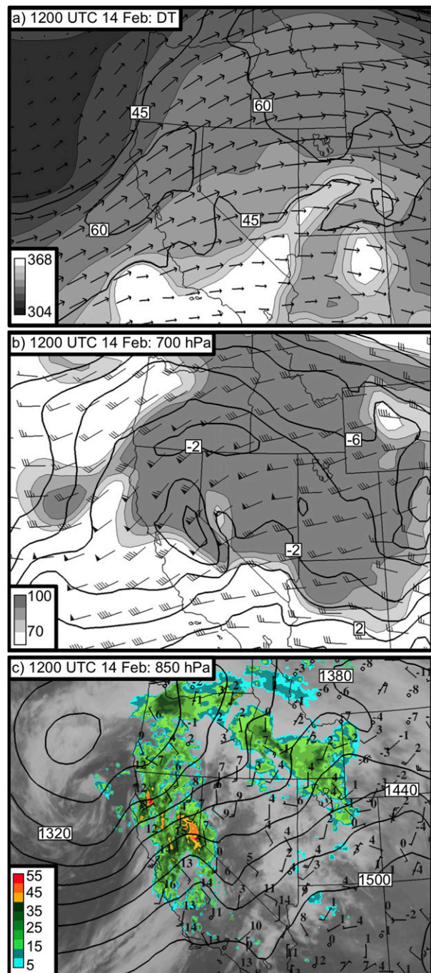
FIG. 3. Regional analyses from the Rapid Update Cycle, version 2 (RUC2; Benjamin et al. 1998) at 1200 UTC 14 Feb 2000. (a) Dynamic tropopause (DT) potential temperature (shaded every 8 K following inset scale), isotachs (contours at 45 and 60 \text{m s}^{-1} ), and wind vectors. (b) 700-hPa temperatures (contours every 2°C), relative humidity greater than 70% (shaded every 10% following inset scale), and wind (pennants, full barbs, and half-barbs denote 25, 5, and 2.5 \text{m s}^{-1} , respectively). (c) 850-hPa geopotential height (contours every 30 m), NEXRAD 8-km composite radar reflectivity (greater than 5 dBZ color-filled following inset scale), infrared satellite imagery, and selected MesoWest surface observations of temperature ( ^{\circ}\text{C} , upper right) and wind [barbs as in (b)].
