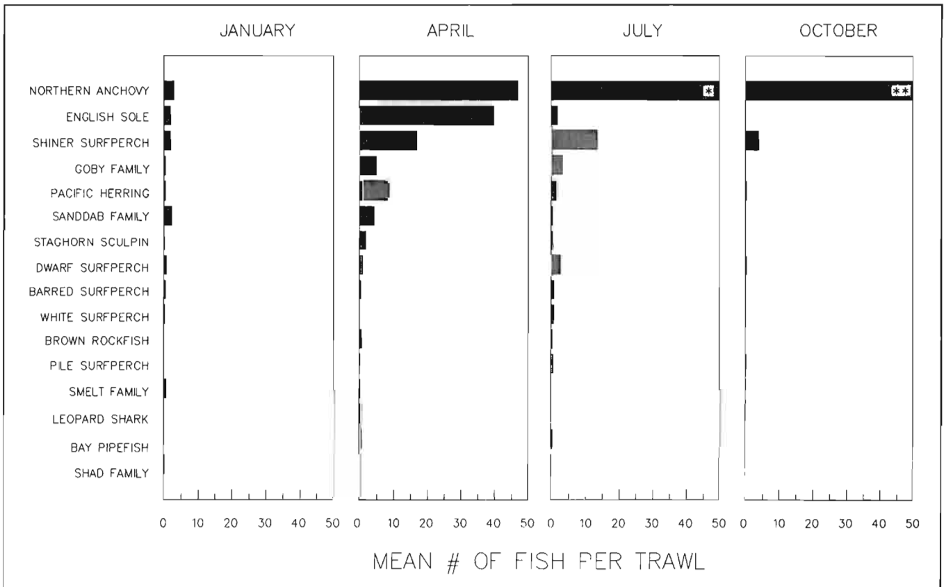
Figure 7 Seasonal comparison of the most abundant species caught in otter trawls, south San Francisco Bay, 1973-82. Abundance values are unweighted. Actual values for northern anchovy exceed the vertical axis (*80 fish per trawl, **129 fish per trawl).
