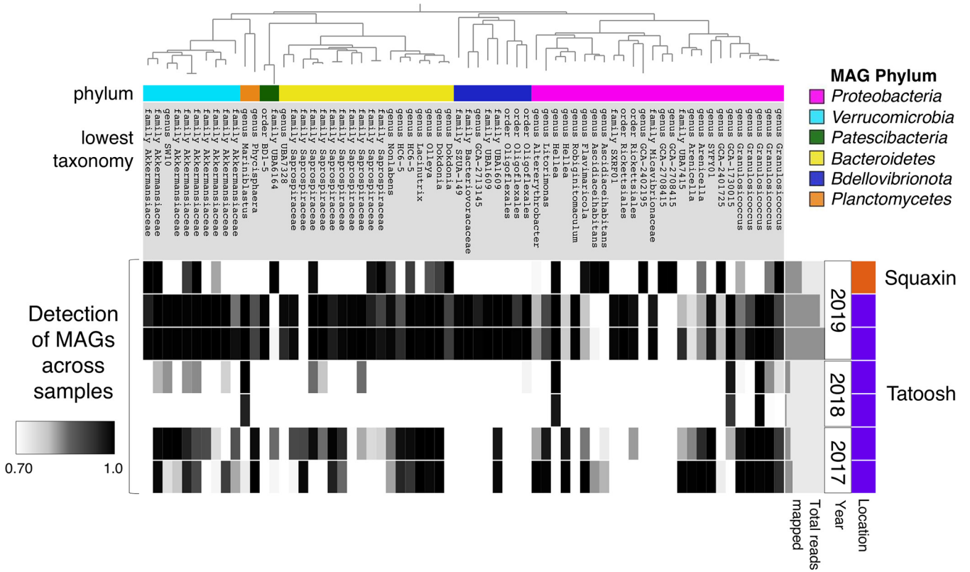
FIG 1 A maximum-likelihood phylogenetic tree of the 66 unique metagenome-assembled genomes (MAGs) (top), colored by bacterial phylum with the lowest taxonomy listed for each MAG, showing the detection of MAGs (columns) across different kelp metagenome samples (rows). MAGs are considered present in a sample if at least 70% of the genome is covered by at least one short read from that sample, so detection ranges from 0.70 to 1.0 (black and gray bars in the heatmap). White bars in the heatmap indicate the absence of a MAG in that sample, where less than 70% of the genome is covered by short reads from that sample. Samples are grouped by location and year, and the small bar graph to the right shows the total number of short reads mapped to all MAGs in each metagenome sample.
