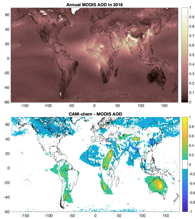
Figure 8. Global distribution of aerosol optical depth (AOD) from the Moderate Resolution Imaging Spectroradiometer (MODIS) averaged for 2018 and the corresponding Community Atmosphere Model with Chemistry (CAM-chem) model simulation bias (model minus observation) for AOD. The CAM-chem simulation used FINNv2.5(MODIS + VIIRS) for fire emissions.
