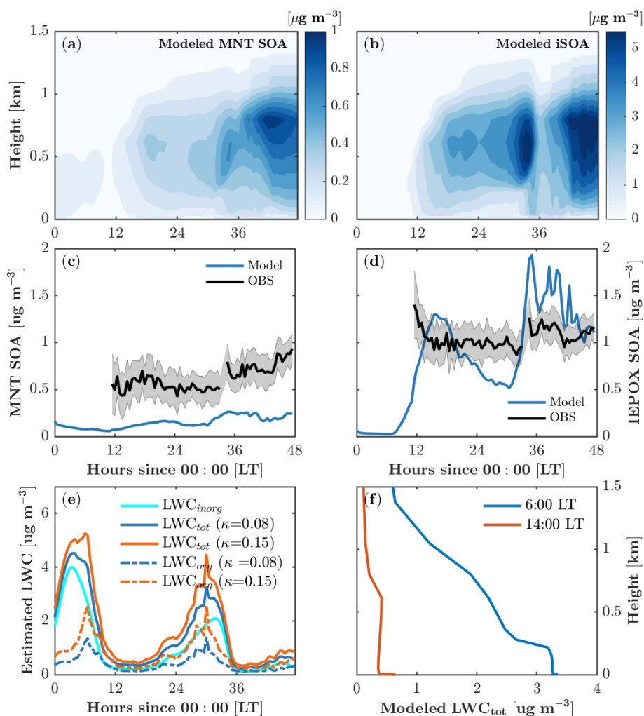
Figure 7. Monoterpene-derived secondary organic aerosol (MNT-SOA) (a) and isoprene-derived secondary organic aerosol (iSOA) (b) as a function of time and height. (c, d) Comparison of modeled MNT-SOA and IEPOX-SOA with observations at 30 m. (e) Time series of calculated liquid water content (LWC) with different hygroscopicity growth \kappa . (f) Vertical profiles of modeled LWC during the daytime (14:00 local time) and in the early morning (6:00 local time).
