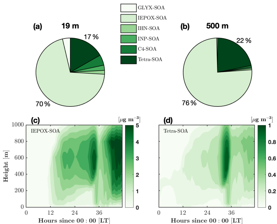
Figure 8. Composition of the average isoprene-derived secondary organic aerosol (iSOA) over the 2 d period at two different heights. The composition components are the surrogate groups of GLYX (glyoxal and methylglyoxal), IEPOX (isoprene-epoxydiol, isoprene-carbonyl-hydroxy-epoxide, and hydroxy methyl- \alpha -lactone), IHNs (isoprene hydroxy nitrates), INPs (nitrooxy hydroperoxides), C4 nitrate, and tetrafunctionals. Details about the surrogate groups can be found in Section 2.5. Composition of iSOA at 19 m (a) and 500 m (b). Isoprene-epoxydiol aerosols (IEPOX-SOA, c) and tetrafunctional compound aerosol (tetra-SOA, d) as a function of time and height.
