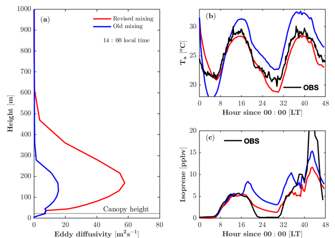
Figure 3. Impacts of the revised mixing parameterization on air temperature and isoprene. (a) Modeled vertical profile of the eddy diffusivity at 14:00 local time on 22 July 2016. (b) Modeled and observed air temperature ( T_a ) at 46 m. (c) Modeled and observed isoprene at 21 m.
