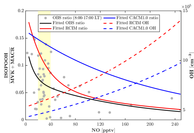
Figure 6. Daytime (08:00–17:00 local time) measurement-based and modeled ratio of ISOPOOH (isoprene hydroxy hydroperoxides) to MVK+MACR (methyl vinyl ketone + methacrolein). Measurement-based ratios of ISOPOOH to MVK+MACR are from 23–27 July 2016 (Grey dots). The fitted exponential curve is for measurement-based ratios (black line), RCIM ratios (red line), CACM1.0 ratios (blue line), RCIM OH concentrations (red dash line), and CACM1.0 OH concentrations (blue dash line). The yellow patch denotes the most frequently observed nitric oxide (NO) levels (20–40 pptv) during the period of 23–27 July 2016.
