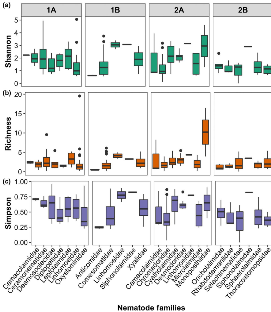
FIGURE 3 Diversity metrics according to nematode family and nematode feeding group. (a) Shannon diversity H' ( \text{Log}_2 ). (b) Margalef's species richness ( d ). (c) Inverted Simpson ( D ) diversity index. Among nematode families, significant differences ( p < .05 ) for Shannon included the following: Desmoscolecidae versus Comesomatidae, Thoracostomopsidae; Comesomatidae versus Desmodoridae; and Diplopeltidae versus Oxystominidae. In addition to those, for the Simpson index significant differences included the following: Desmoscolecidae versus Camacolaimidae, Cyatholaimidae
