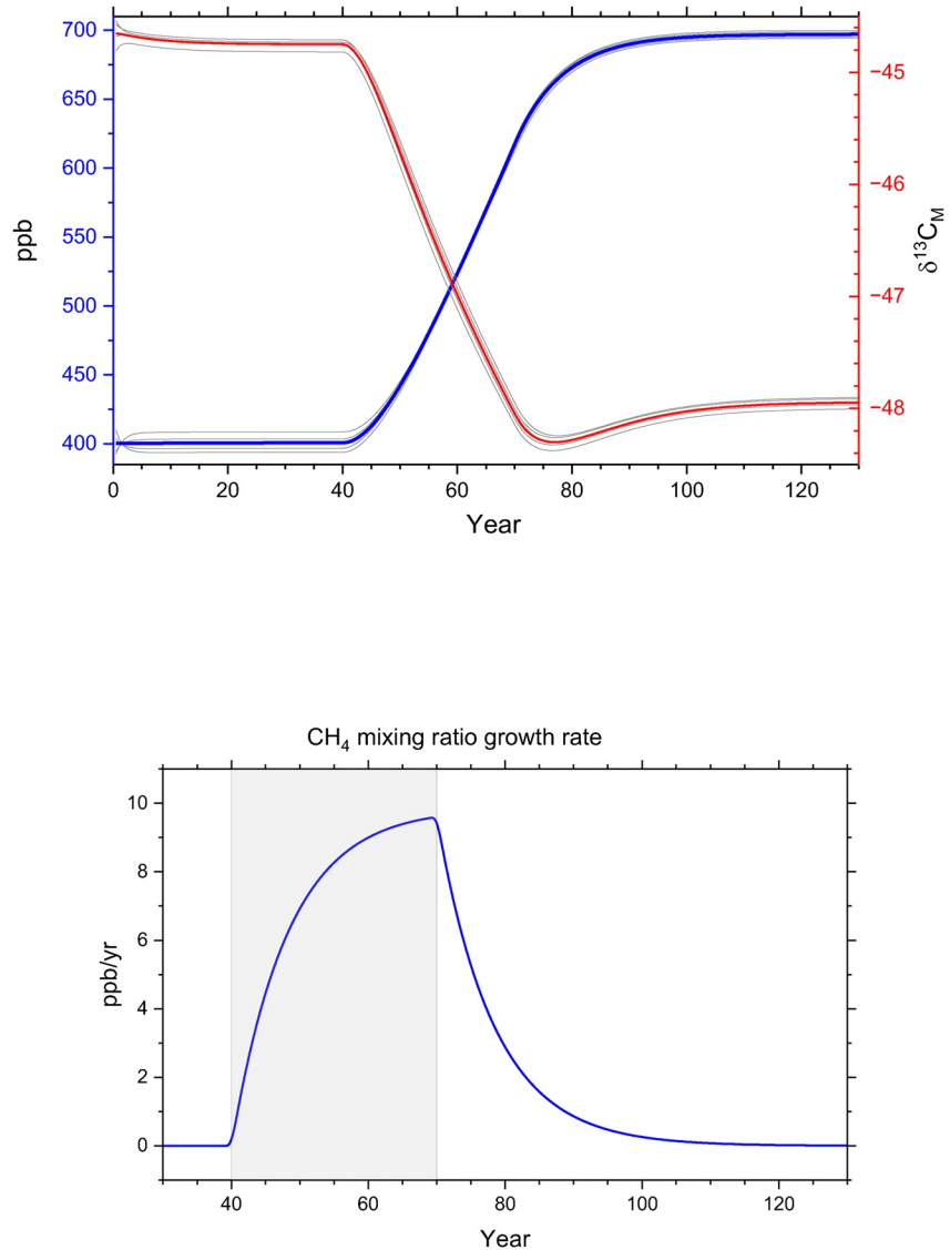
Figure 10. Termination event model (Section 9.1.1) (a) Methane mole fraction ( \delta^{13}C_M ) in ppb and \delta^{13}C_{CH_4} from the 4-box running budget analysis with a 30-yr transition from “Initial” to “Post” sources. Blue is the global average mole fraction and thin lines are for the four semi-hemispheres. The latitudinal distribution of the CH_4 mole fraction reverses from being lowest in 30°N–90°N to being the highest there. Red is the global average \delta^{13}C_M and thin lines show values for each semi-hemisphere and this change in \delta^{13}C_{CH_4} is uniform across all semi-hemispheres. (b) Growth rate (ppb/yr) of the global average CH_4 mixing ratio in Figure 10a.
