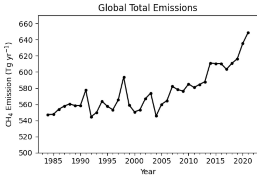
Figure 7. Global methane emissions, estimated and updated using the top-down methodology of Lan, Basu, et al. (2021) and Basu et al. (2022). For further details and data sources, see supplementary information in Lan, Basu, et al., 2021; Figure S2b in Supporting Information S1, red curve, updated.
