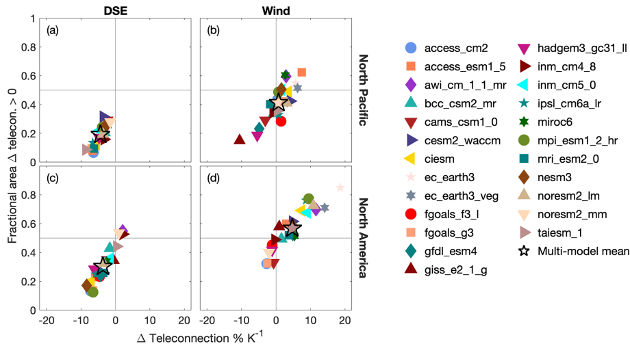
Figure 4. For individual CMIP6 model mean states and the multi-model mean, the change in the teleconnection amplitude (as a percent change per multi-model mean kelvin warming) to the North Pacific (25–70° N, 150–235° E) and North America (25–70° N, 235–290° E) between LBM simulations with mean states given by future and historical quantities. The isolated change due to (a) stability, over the North Pacific; (b) wind, over the North Pacific; (c) stability, over North America; and (d) wind, over North America. The horizontal axis is the domain mean change over the region, while the vertical axis shows the fractional area of teleconnection amplitude strengthening. DSE indicates dry static energy.
