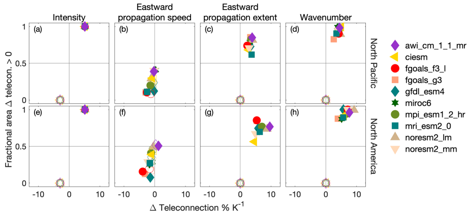
Figure 7. For individual CMIP6 model mean states, the change in the teleconnection amplitude (as a percent change per multi-model mean kelvin warming) to the North Pacific (25–70° N, 150–235° E) and North America (25–70° N, 235–290° E) between LBM simulations with the control and perturbed thermal forcing. (a, e) Response to perturbed heating intensity, (b, f) eastward propagation speed, (c, g) eastward propagation extent, and (d, h) zonal wavenumber. Unfilled (filled) markers represent the lower (upper) bounds of perturbations to each MJO feature expected at the end of the century given a high-emissions scenario (see Table 1).
