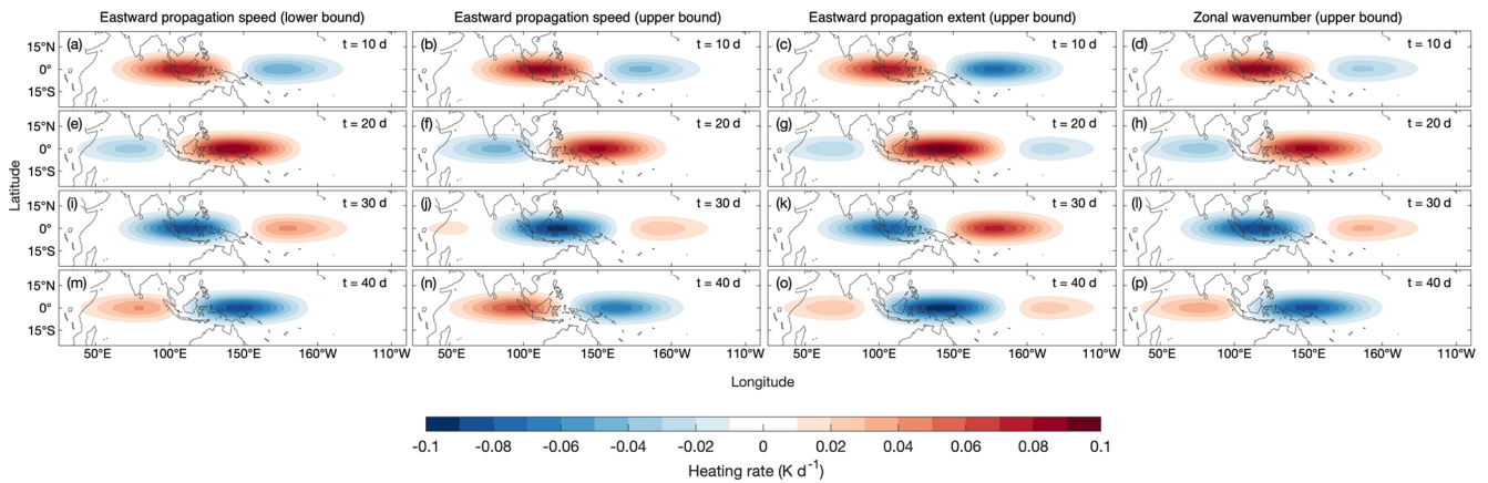
Figure A1. As in Fig. 1 but for the perturbed MJO cases for (a, e, i, m) the lower bound of the propagation speed experiment, (b, f, j, n) the upper bound of the propagation speed experiment, (c, g, k, o) the upper bound of the increased eastward propagation extent experiment, and (d, h, l, p) the upper bound of the perturbed wavenumber experiment.
