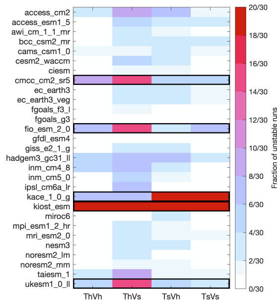
Figure A2. For each model mean state combination, the fraction of the 30 ensemble members that met the instability criterion described in Sect. 2. Models omitted from our analysis (those for which 10 or more of their ensemble members for any of the mean state combinations became unstable) are indicated by the black outline. Th (Ts) indicates the mean state dry static stability from the historical (future) period; Vh (Vs) indicates the mean state winds from the historical (future) period.
