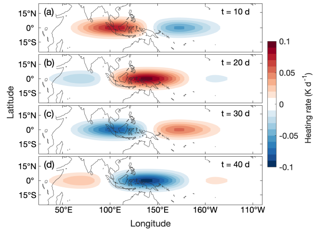
Figure 1. Propagating thermal forcing used in the LBM simulations at t = (a) 10 d, (b) 20 d, (c) 30 d, and (d) 40 d.
