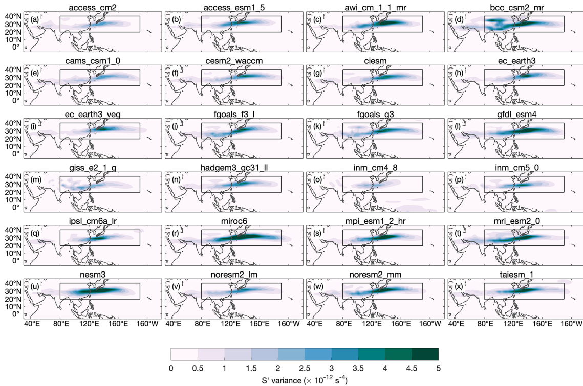
Figure A3. The temporal variance of the ensemble mean Rossby wave source ( S' ) with the full mean states given by historical quantities. The box around the region (20–40° N, 80–190° E) indicates the region used for Fig. 5 of the main text.
