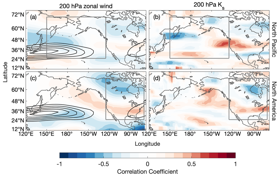
Figure 6. Correlation coefficient between the local change in the 200 hPa zonal wind and the regional mean change in the teleconnection amplitude over (a) the North Pacific and (c) North America. Correlation coefficient between the local change in the stationary Rossby wave number, K_s , and the regional mean change in the teleconnection amplitude over (b) the North Pacific and (d) North America. Grey boxes outline the North Pacific and North America regions.
