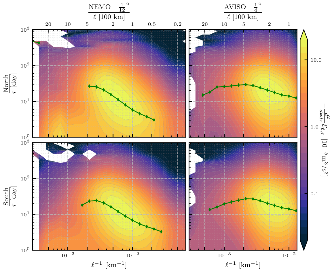
Figure 11. Combined spatio-temporal coarse-graining producing 2D spectra, -\partial_{\tau} \partial_{k_{\ell}} \mathcal{E}_{\ell, \tau} from [left] 1/12^{\circ} NEMO and [right] AVISO, averaged over the [top] NH and [bottom] SH. Mesoscale energy predominantly peaks on length-scales of 100–200 km and time-scales of 1–3 weeks. Green diamonds indicate, for each \ell , the \tau at which spectral power is maximized (cf. Figure 13).
