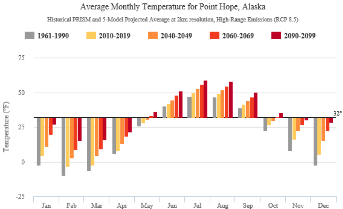
Figure 12. Decadal means of downscaled temperatures (°F) for Point Hope, Alaska as a function of calendar month (x-axis) under the RCP 4.5 scenario (upper) and RCP 8.5 scenario (lower).
