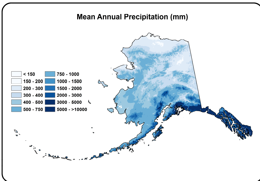
Figure 2. 1950-1999 mean annual mean temperature (upper) and total precipitation (lower) for Alaska based on downscaled CRU TS 3.1 (Scenarios for Alaska and Arctic Planning, University of Alaska, Fairbanks, after Harris et al. 2014). Alaska station data availability in CRU was most consistent for the 1950-1999 timeframe.
