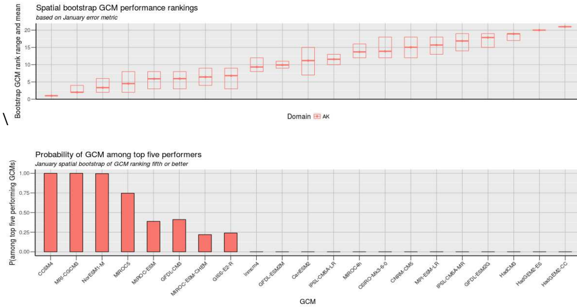
Figure 4. Upper panel: Mean value and ranges of ranks of RMSE of January temperature based on 1000 random resamplings (with replacement) of Alaska-domain grid cells. Highest-ranking (smallest RMSE) model is on left, lowest-ranking (largest RMSE) model is on right. Lower panel: Probability (based on 1000-member resampling) that a model ranks in the top five, based on the RMSE of January temperature. Source: https://uasnap.shinyapps.io/ar5eval/
