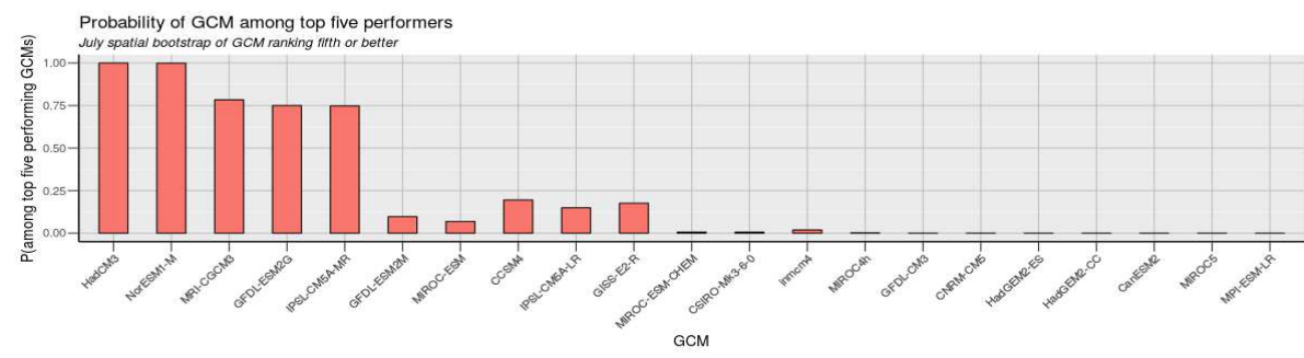
Figure 5. As in Figure 4, but for July precipitation over the Alaska domain.
