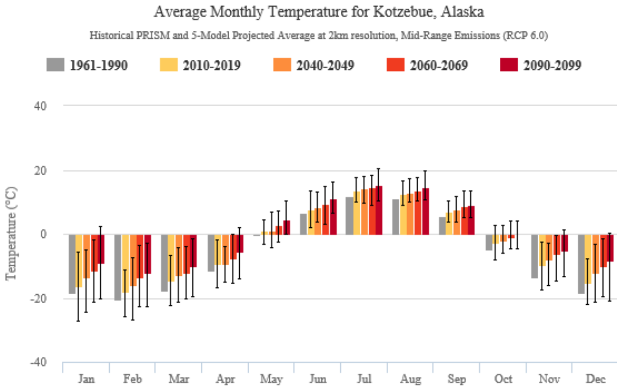
Figure 9. Decadal means of downscaled temperatures (°C) for Kotzebue, Alaska as a function of calendar month (x-axis). Colored bars are means for individual decades. Thin vertical lines denote range of the temperatures obtained from the five models. Results are for RCP 6.0 (mid-range) emission scenario.
