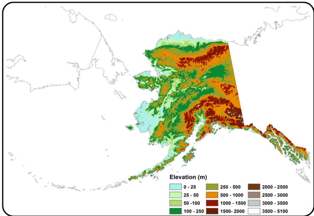
Figure 1 Topography and coastal configuration of Alaska. Source: Scenarios Network for Alaska and Arctic Planning (SNAP), http://data.snap.uaf.edu/data/IEM/Inputs/ancillary/elevation/iem_prism_dem_1km.tif , modified by J. Littell.
