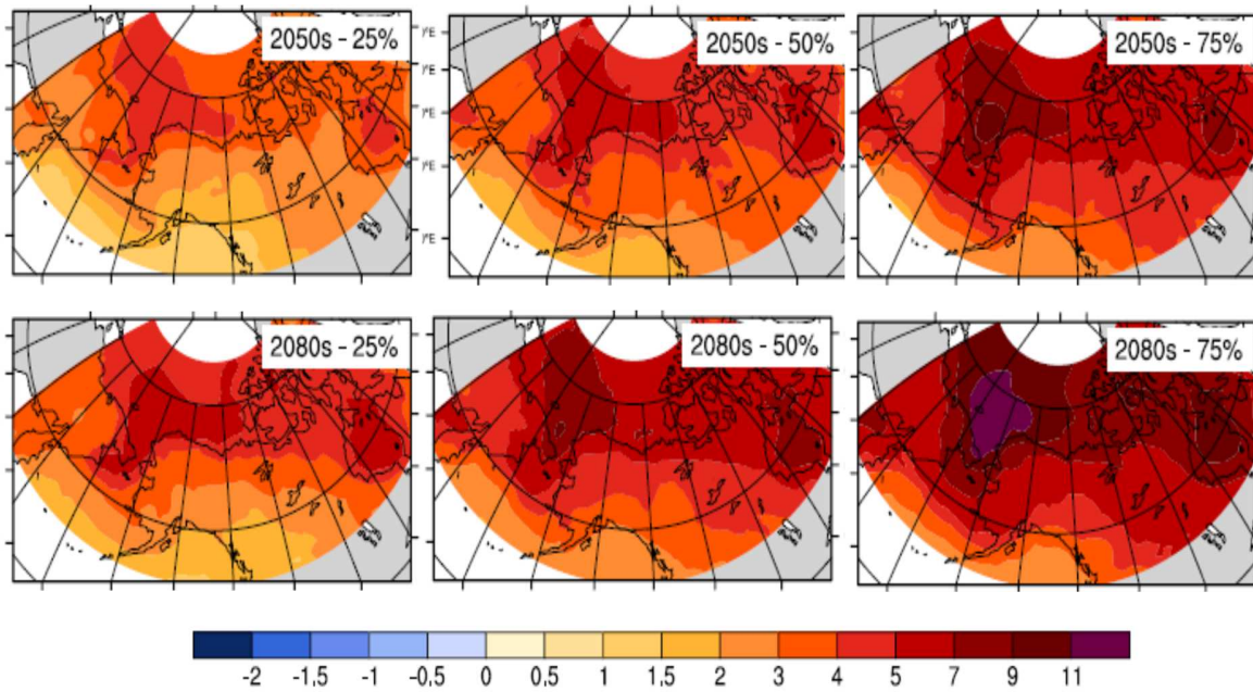
Figure 7. Projected temperature changes over Alaska and surrounding region in the 2050s (top row) and 2080s (bottom row) under the RCP 4.5 scenario. Changes for each time slice are shown for the 25 th -percentile model (left), the 50 th -percentile model (center) and 75 th -percentile model (right) based on a ranking of the models by the average warming over the domain. Figure provided by Greg Flato and Robin Rong, Environment Canada.
