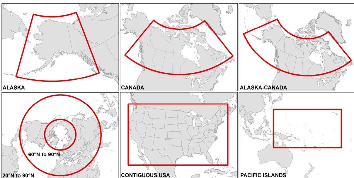
Figure 3. The seven domains for which the model evaluation was performed. Note that there are two circumpolar domains in the lower left panel: 60°-90°N and 20°-90°N.
