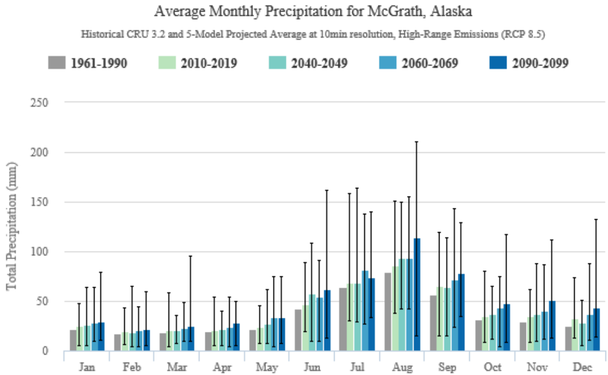
Figure 10. As in Figure 8, but for calendar-month precipitation (mm) at McGrath, Alaska under the RCP 8.5 scenario and referenced to the CRU 3.2 historical climatology.
