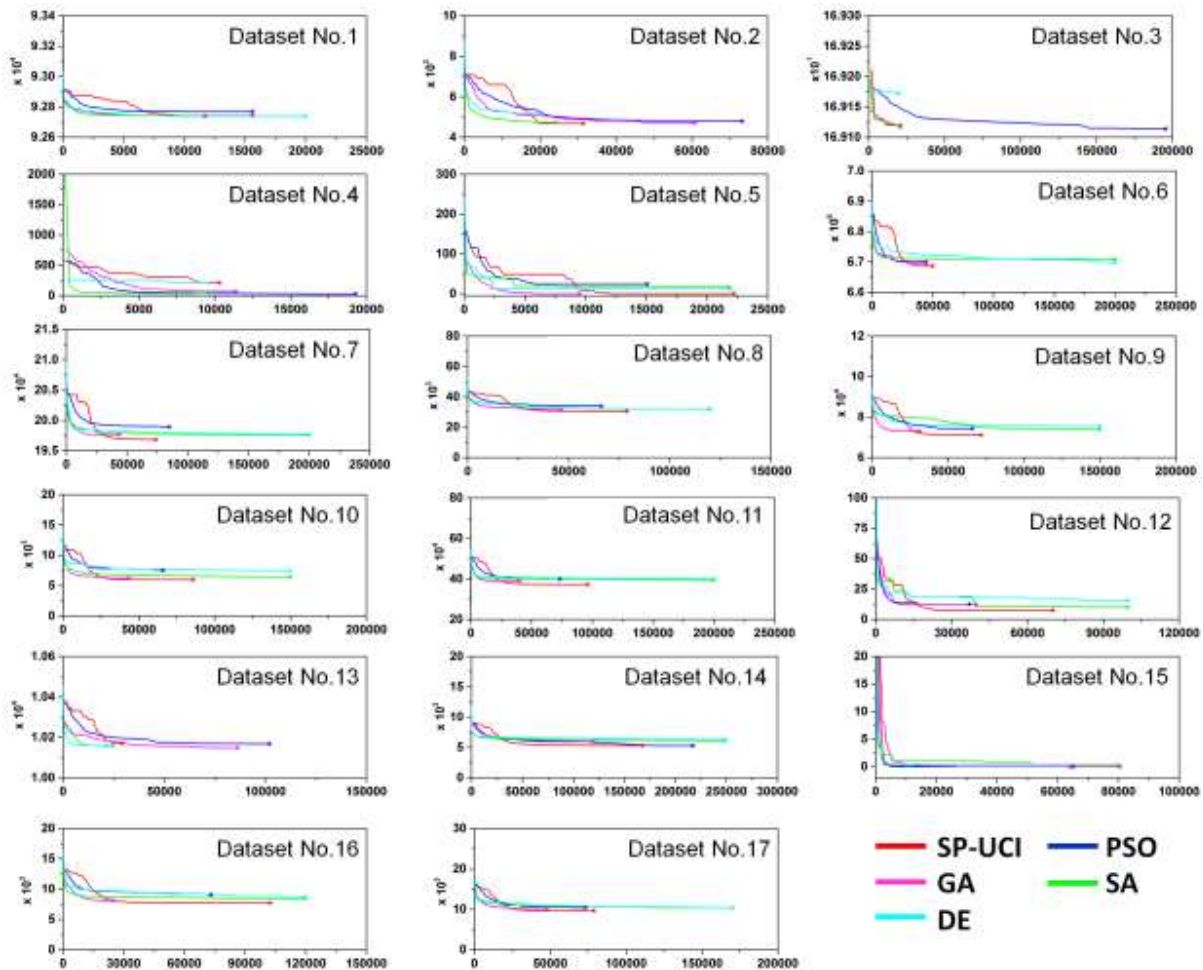
Figure 2. The evolution processes of SP-UCI-, GA-, PSO-, SA-, and DE-based ANN on different datasets
