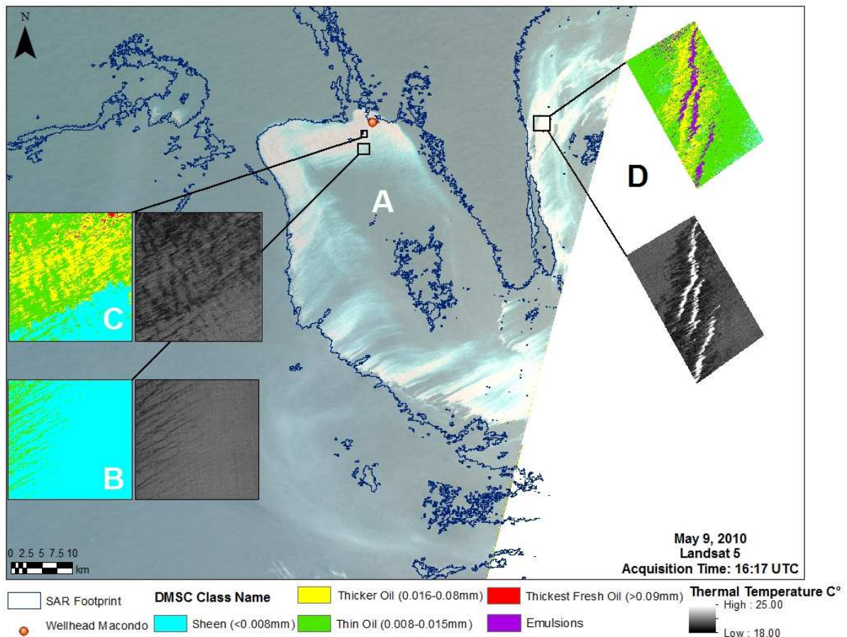
Figure 3. Landsat-5 TM blue/green/near-IR rendition of portion of the DWH spill slick acquired on 9 May, 2010. Insets show corresponding DMSC/IR oil thickness classification and thermal imagery examples in different parts of the TM-covered slick. The examples show characteristics corresponding to the different TM-derived oil volume quantification classes: (A) sheen, (B) Low Surface Oil Volume, (C) Mid-volume, (D) High Volume. The SAR-derived slick perimeter is also shown in the TM-covered portion.
