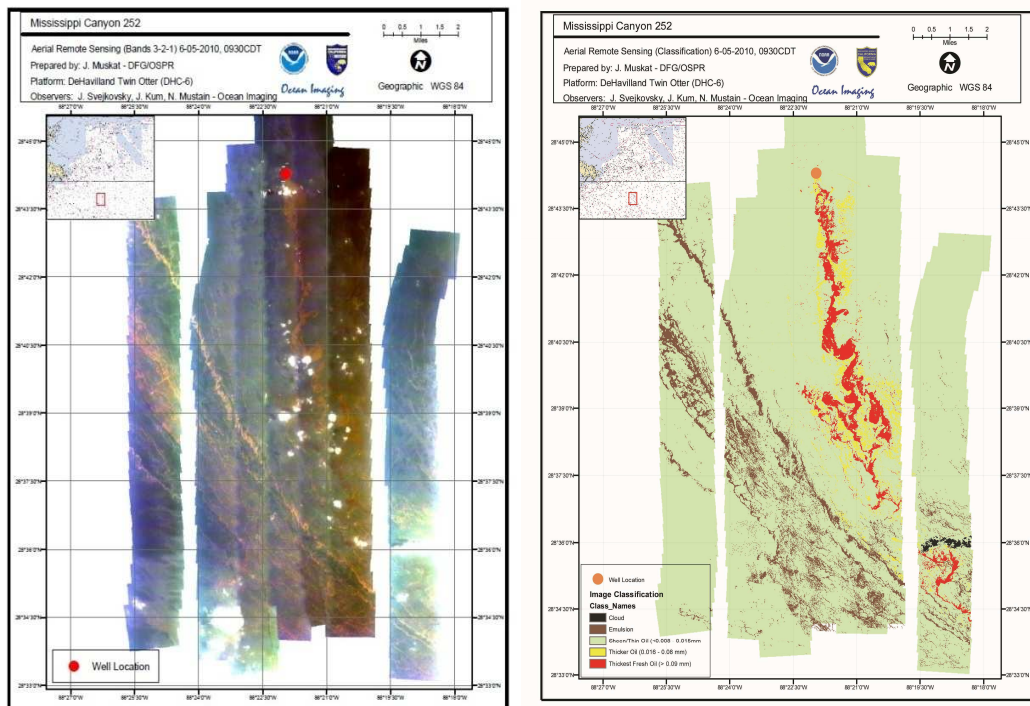
Figure 2. DMSC/IR multispectral image mosaic of the DWH spill source plume region acquired on 6 May 2010 (left) and resulting oil thickness classification (right)
