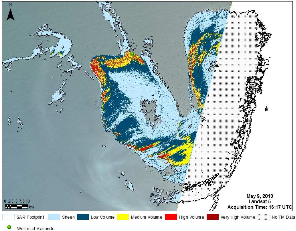
Figure 4. Final TM-derived oiling characterization classification for 9 May, 2010.
