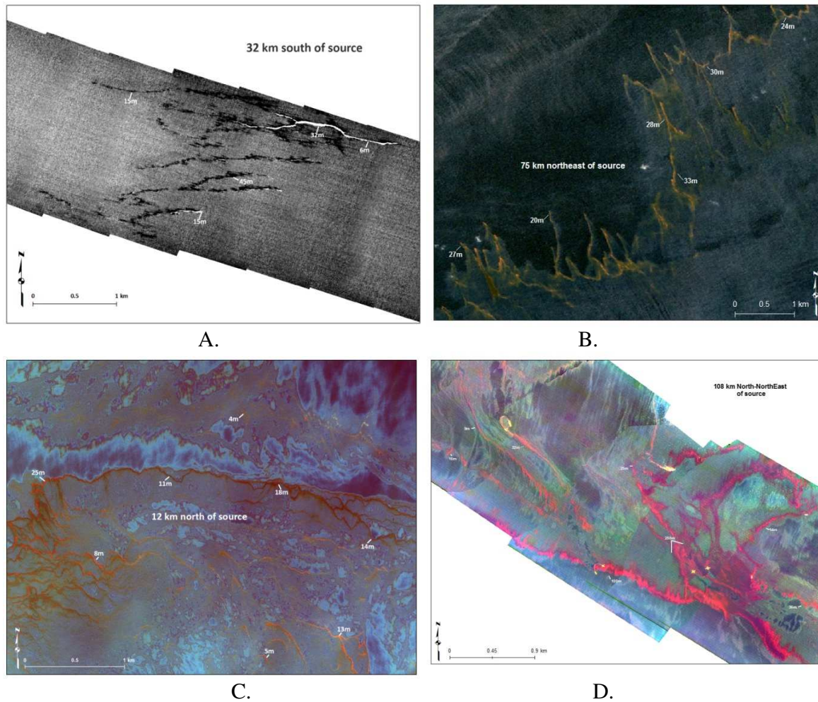
Figure 7. Sample images of sheen, metallic and emulsion oil features existing in regions away from the spill source site, also showing representative widths of the emulsion strands: (A) Thermal IR rendition from the DMSC/IR sensor on 5/10/2010 (note that the sheen and metallic thickness features exhibit no thermal contrast signal and hence are not visible); (B)
