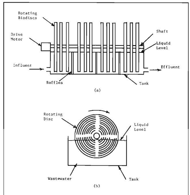
Figure 9—Rotating biodisc system (a) side view and (b) end view.
