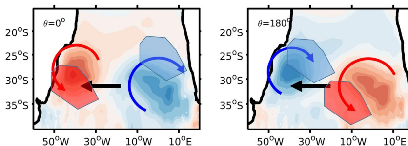
Figure 11. Schematic of the effect of the propagating oceanic heat transport on the warming and cooling of the western and eastern South Atlantic regions at two opposite phases. The contours (colored shading) are for SLA and the black horizontal arrows indicate westward propagation of the oceanic features. The red and blue arrows indicate the tendency for warming and cooling of the regions represented by the polygonal regions.
