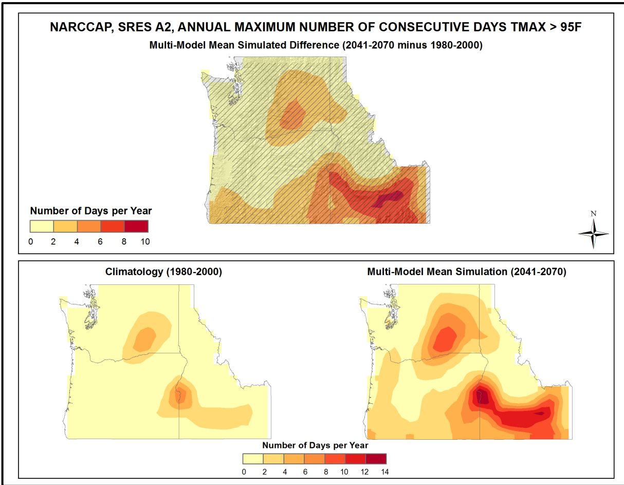
Figure 16. Simulated difference in the mean annual maximum number of consecutive days with a maximum temperature greater than 95^{\circ}\text{F} ( T_{max} > 95^{\circ}\text{F} ) for the Northwest region, for the 2041-2070 time period with respect to the reference period of 1980-2000 (top). Color only (category 1) indicates that less than 50% of the models show a statistically significant change in the number of consecutive days. Color with hatching (category 3) indicates that more than 50% of the models show a statistically significant change in the number of consecutive days, and more than 67% agree on the sign of the change (see text). Mean annual maximum number of consecutive days with T_{max} > 95^{\circ}\text{F} for the 1980-2000 reference period (bottom left). Simulated mean annual maximum number of consecutive days with T_{max} > 95^{\circ}\text{F} for the 2041-2070 future time period (bottom right). These are multi-model means from 8 NARCCAP regional climate simulations for the high (A2) emissions scenario. Note that top and bottom color scales are different. Increases are largest in the southeastern portion of the region.
