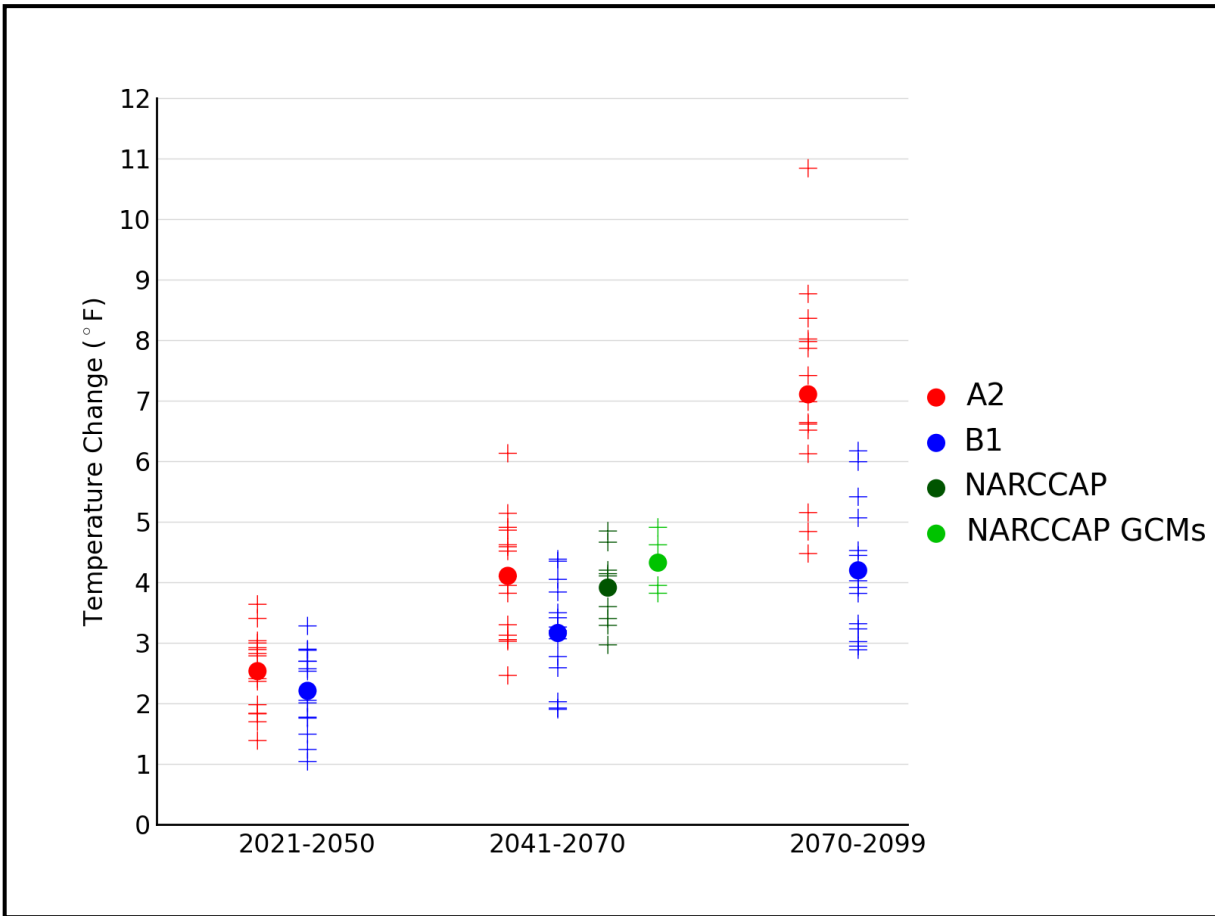
Figure 11. Simulated annual mean temperature change (°F) for the Northwest region, for each future time period (2021-2050, 2041-2070, and 2070-2099) with respect to the reference period of 1971-1999 for the CMIP3 models and 1971-2000 for the NARCCAP models. Values are given for the high (A2) and low (B1) emissions scenarios for the 14 (B1) or 15 (A2) CMIP3 models. Also shown for 2041-2070 (high emissions scenario only) are values for 9 NARCCAP models, as well as for the 4 GCMs used to drive the NARCCAP simulations. The small plus signs indicate each individual model and the circles depict the multi-model means. The range of model-simulated changes is large compared to the mean differences between A2 and B1 in the early and middle 21 st century. By the end of the 21 st century, the difference between A2 and B1 is comparable to the range of B1 simulations.
