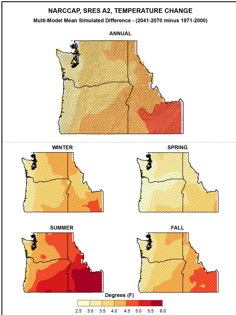
Figure 10. Simulated difference in annual and seasonal mean temperature ( ^{\circ}\text{F} ) for the Northwest region, for 2041-2070 with respect to the reference period of 1971-2000. These are multi-model means from 11 NARCCAP regional climate simulations for the high (A2) emissions scenario. Color with hatching (category 3) indicates that more than 50% of the models show a statistically significant change in temperature, and more than 67% agree on the sign of the change (see text). Note that the color scale is different from that of Fig. 9. Annual temperature changes for the NARCCAP simulations are similar to those for the CMIP3 global models (Fig. 9, middle left panel), but with greater warming in the southeastern portion of the region. Seasonal warming shows similar patterns in all seasons, with the greatest warming occurring in summer and winter.
