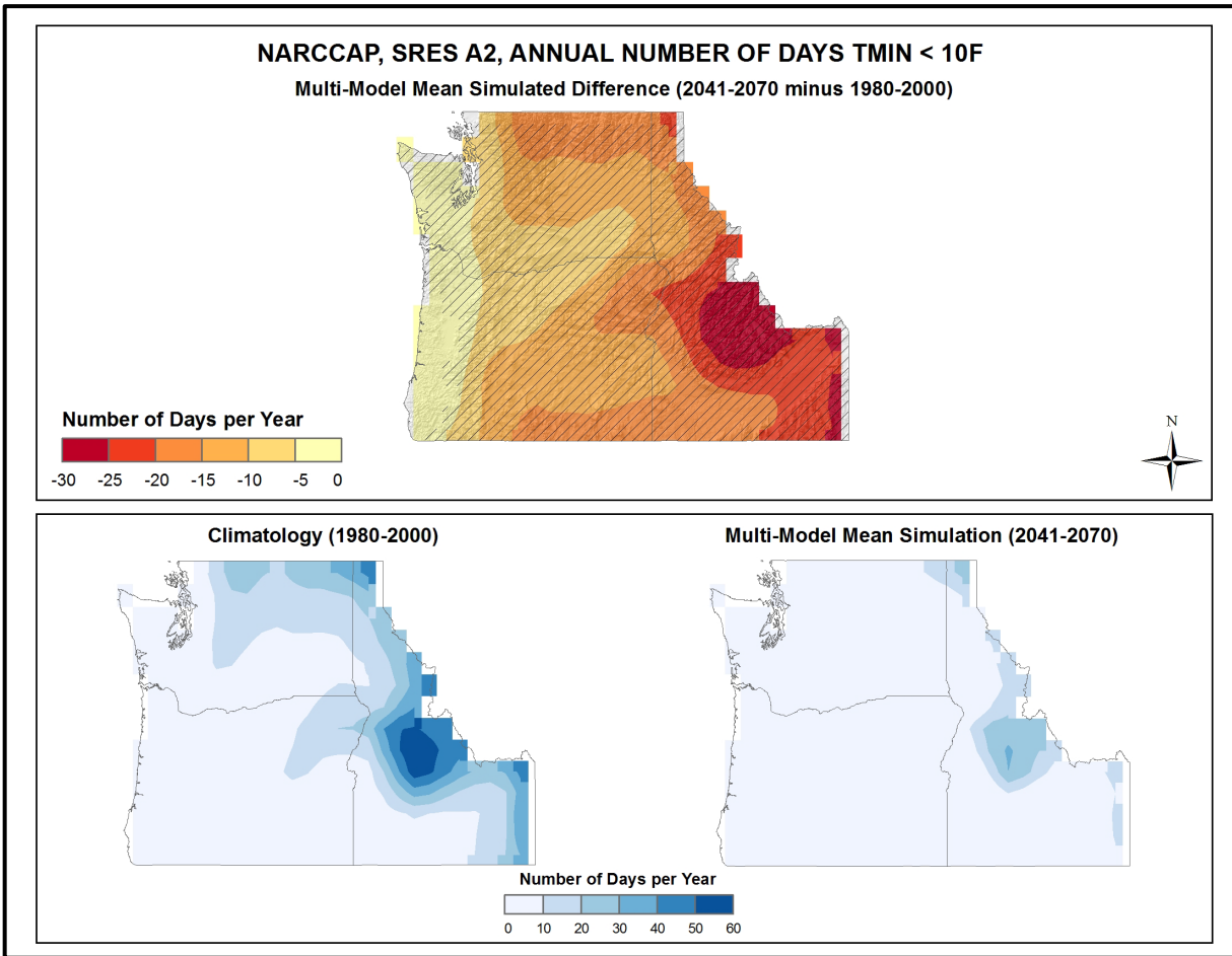
Figure 14. Simulated difference in the mean annual number of days with a minimum temperature less than 10^{\circ}F ( T_{min} < 10^{\circ}F ) for the Northwest region, for the 2041-2070 time period with respect to the reference period of 1980-2000 (top). Color only (category 1) indicates that less than 50% of the models show a statistically significant change in the number of days. Color with hatching (category 3) indicates that more than 50% of the models show a statistically significant change in the number of days, and more than 67% agree on the sign of the change (see text). Mean annual number of days with T_{min} < 10^{\circ}F for the 1980-2000 reference period (bottom left). Simulated mean annual number of days with T_{min} < 10^{\circ}F for the 2041-2070 future time period (bottom right). These are multi-model means from 8 NARCCAP regional climate simulations for the high (A2) emissions scenario. Decreases are largest for inland areas, while coastal regions are simulated to experience almost no change.
