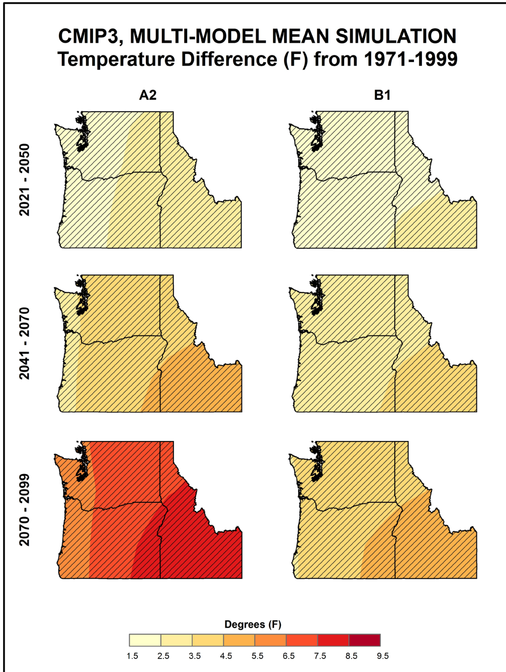
Figure 9. Simulated difference in annual mean temperature (°F) for the Northwest region, for each future time period (2021-2050, 2041-2070, and 2070-2099) with respect to the reference period of 1971-1999. These are multi-model means for the high (A2) and low (B1) emissions scenarios from the 14 (B1) or 15 (A2) CMIP3 global climate simulations. Color with hatching (category 3) indicates that more than 50% of the models show a statistically significant change in temperature, and more than 67% agree on the sign of the change (see text). Temperature changes increase throughout the 21 st century, more rapidly for the high emissions scenario.
