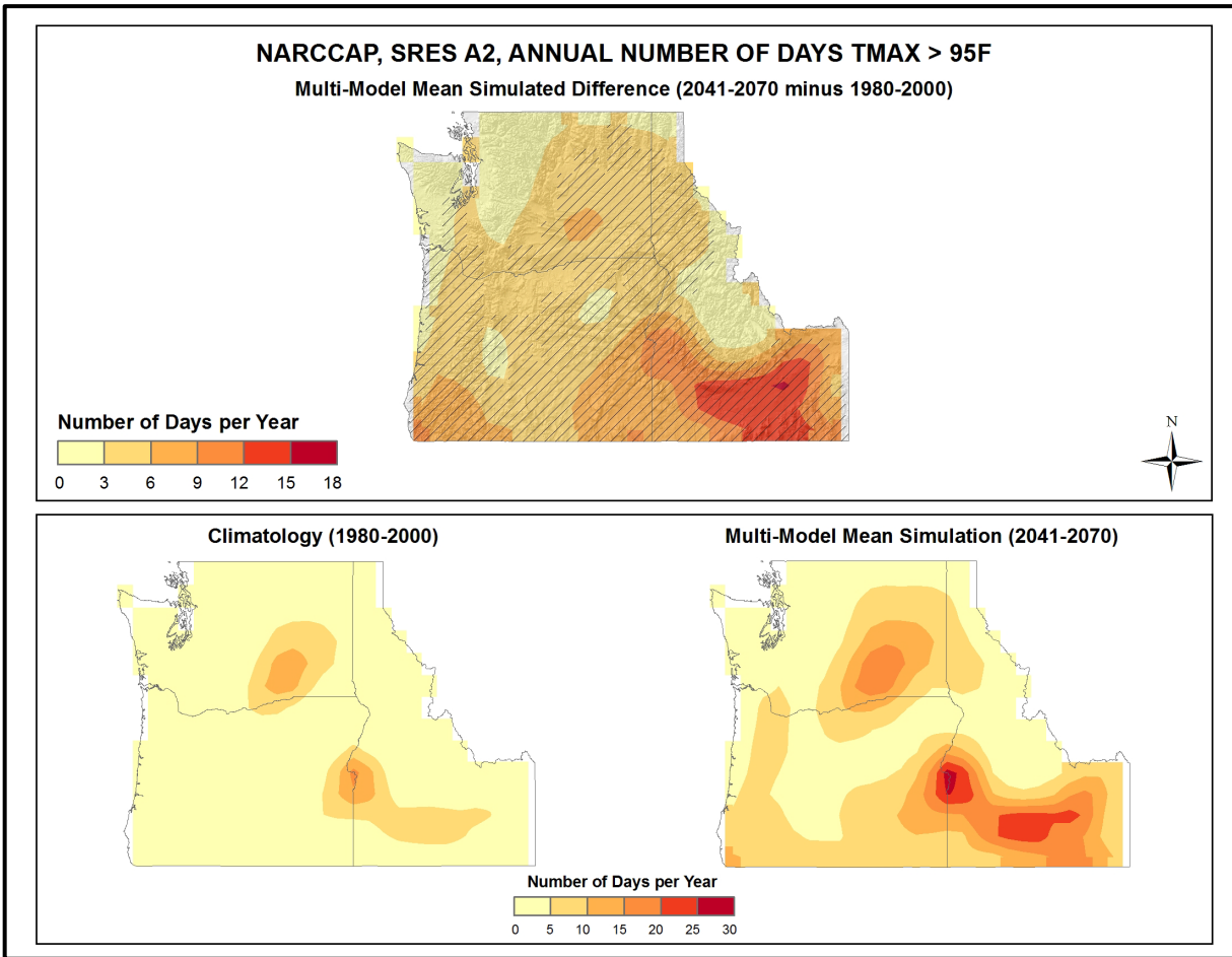
Figure 13. Simulated difference in the mean annual number of days with a maximum temperature greater than 95°F ( T_{max} > 95^{\circ}\text{F} ) for the Northwest region, for the 2041-2070 time period with respect to the reference period of 1980-2000 (top). Color only (category 1) indicates that less than 50% of the models show a statistically significant change in the number of days. Color with hatching (category 3) indicates that more than 50% of the models show a statistically significant change in the number of days, and more than 67% agree on the sign of the change (see text). Mean annual number of days with T_{max} > 95^{\circ}\text{F} for the 1980-2000 reference period (bottom left). Simulated mean annual number of days with T_{max} > 95^{\circ}\text{F} for the 2041-2070 future time period (bottom right). These are multi-model means from 8 NARCCAP regional climate simulations for the high (A2) emissions scenario. Note that top and bottom color scales are different. Increases are smallest at high elevations and largest in the southeastern portion of the region.
