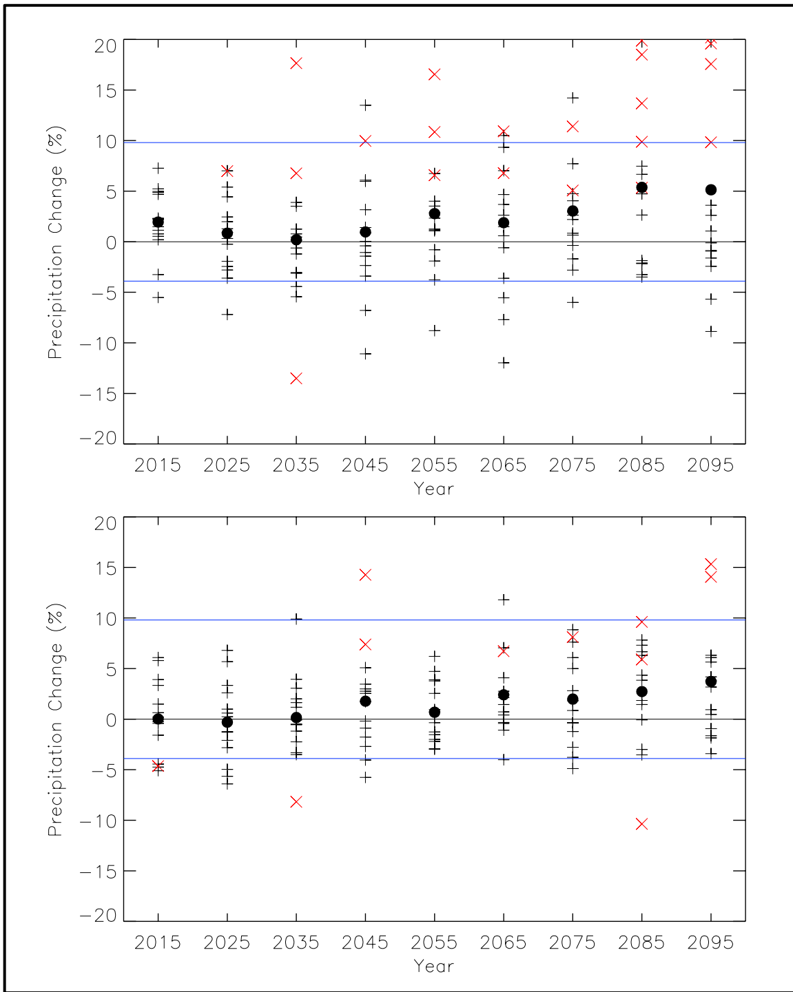
Figure 33. Simulated decadal mean change in annual precipitation (%) for the Northwest U.S. for each future decadal time period (represented by their approximate midpoints, e.g., 2015 = 2011-2020), with respect to the reference period of 2001-2010. Values are given for the high (A2, top) and low (B1, bottom) emissions scenarios for the 14 (B1) or 15 (A2) CMIP3 models. Large circles depict the multi-model means. Each individual model is represented by a black plus sign (+), or a red x if the value is statistically significant at the 95% confidence level. Blue lines indicate the 10 th and 90 th percentiles of the 30 annual anomaly values from 1981-2010. Many models simulate precipitation changes that are not statistically significant out to the end of the 21 st century.
