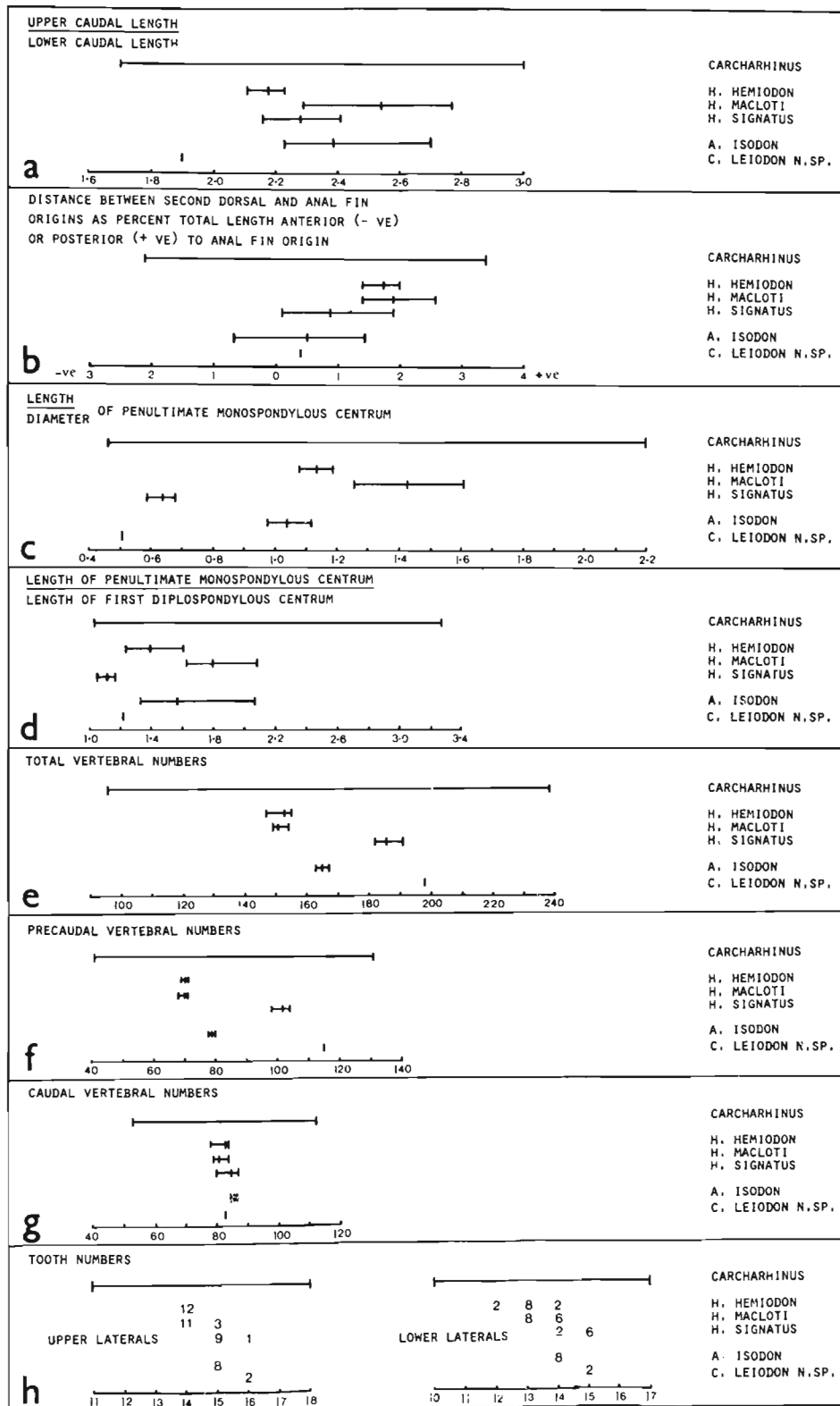
Figure 4.—Proportional dimensions, vertebral numbers, and tooth numbers of the species formerly referred to Hypoprion ( H. hemiodon , H. macloti , and H. signatus ) and of Aprionodon ( A. isodon ), and those of Carcharhinus leiodon n.sp. In a-g, data are expressed as ranges and means. In h, tooth numbers are given as a frequency table. For a-h, the range in 25 species of Carcharhinus is also shown for comparison.
